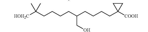
1-(11-Hydroxy-5-hydroxymethyl-10,10-dimethyl-undecyl)-cyclopropanecarboxylic acid Compound 85
