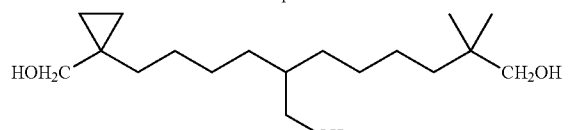
7-[4-(1-Hydroxymethyl-cyclopropyl)-butyl]-2,2-dimethyl-octane-1,8-diol Compound 83
