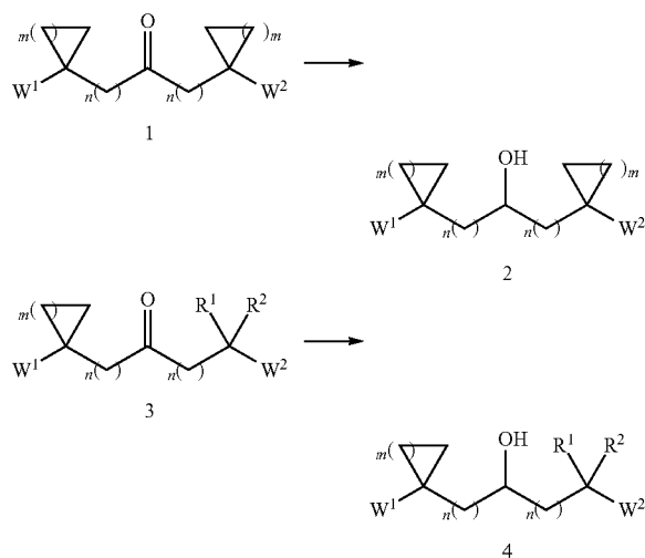
Scheme 1: Synthesis of compounds of formula 2 and 4
