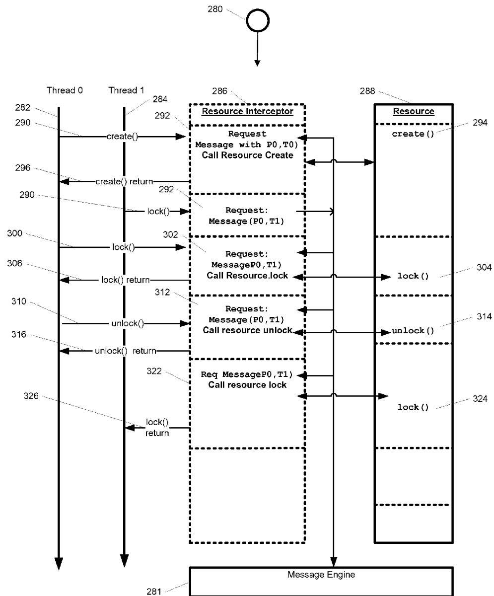
FIG.8 – Backup's Processing of replication messages
