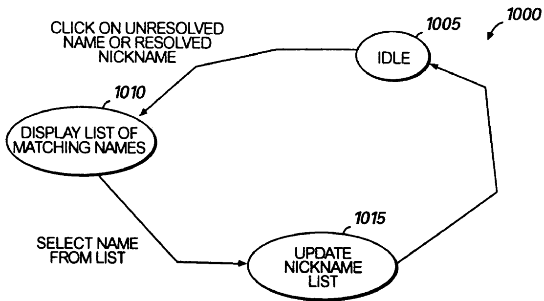
STATE DIAGRAM - NICKNAME RESOLUTION FROM PROGRAM'S PERSPECTIVE
