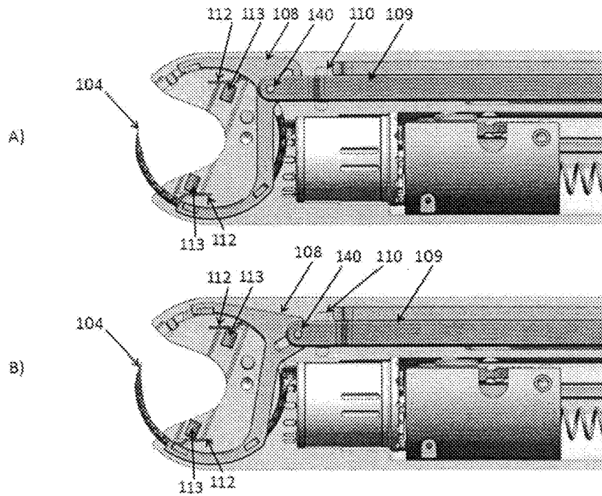
Figure 36: Needle Advancer Arm Actuation
