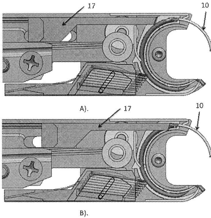
Figure 17: Clip Cutting
