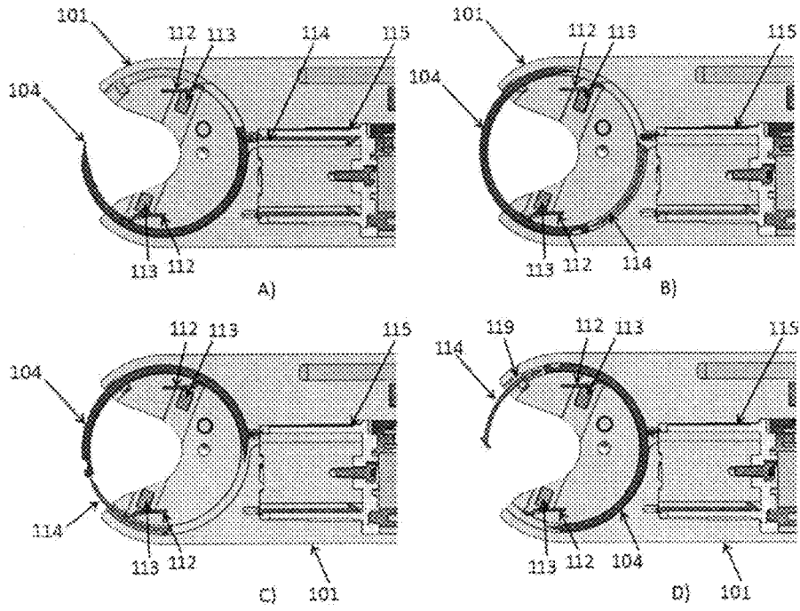
Figure 37: Needle Advancement Sequence
