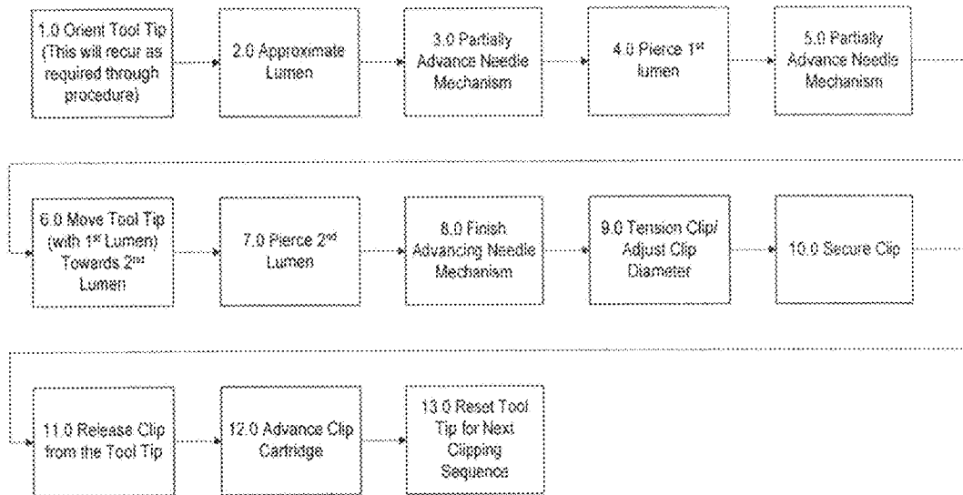
Figure 52: Sequence of Operation for the Clipping Method
