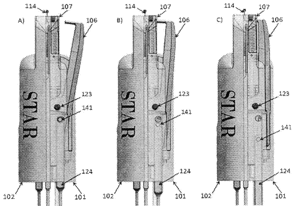
Figure 41: Clasp Closing Actuator
