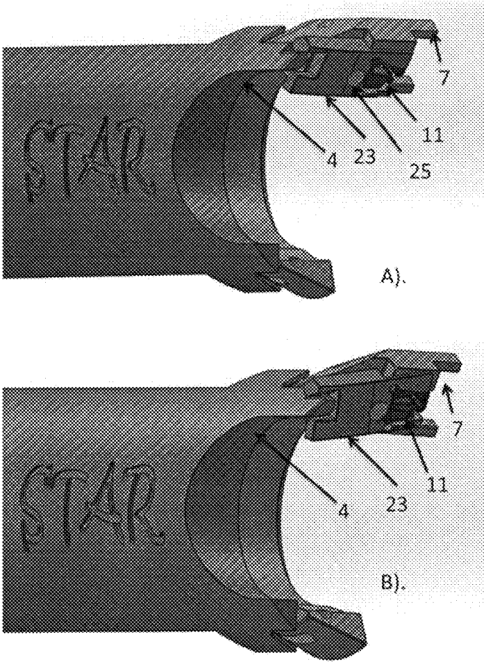
Figure 16: Clasp Closing
