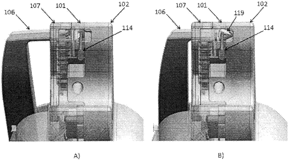
Figure 42: Clasp Closing
