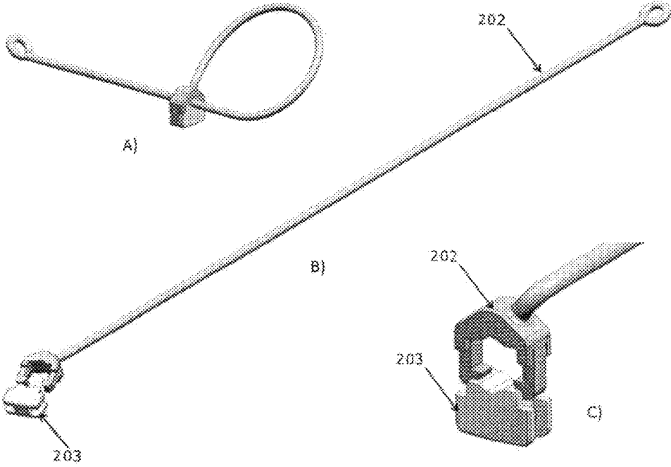
Figure 56: Clip and Clasp
