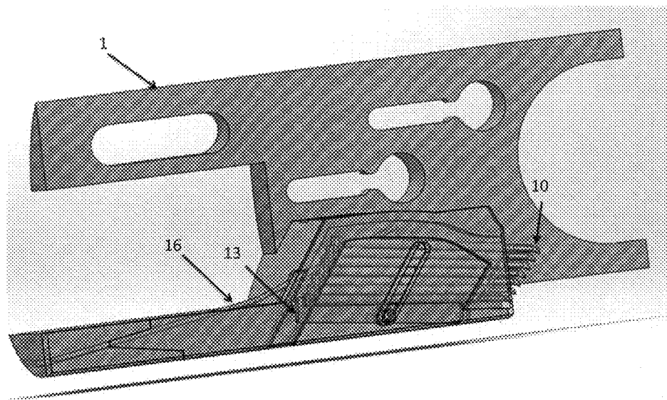
Figure 18: Clip Cartridge Advancement Mechanism (Top View)
