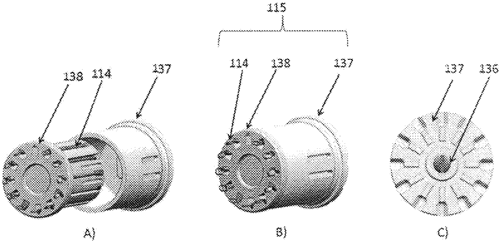
Figure 32: Clip Cartridge Loading
