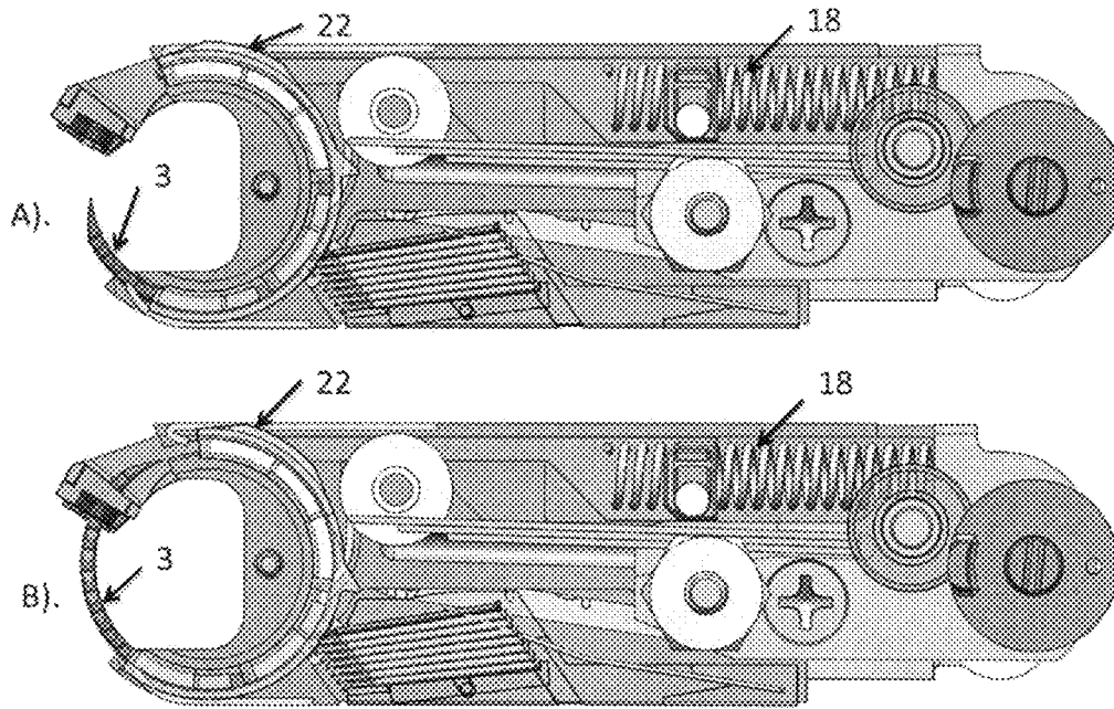
Figure 10: Needle Advancer Arm Actuation
