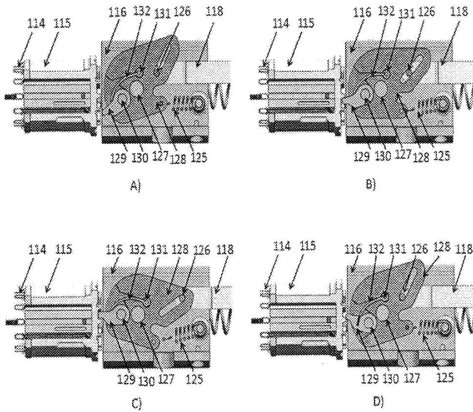
Figure 48: Cartridge Advancement Sequence (Top View)
