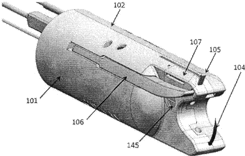
Figure 28: Clipping Tool Tip Isometric View #2
