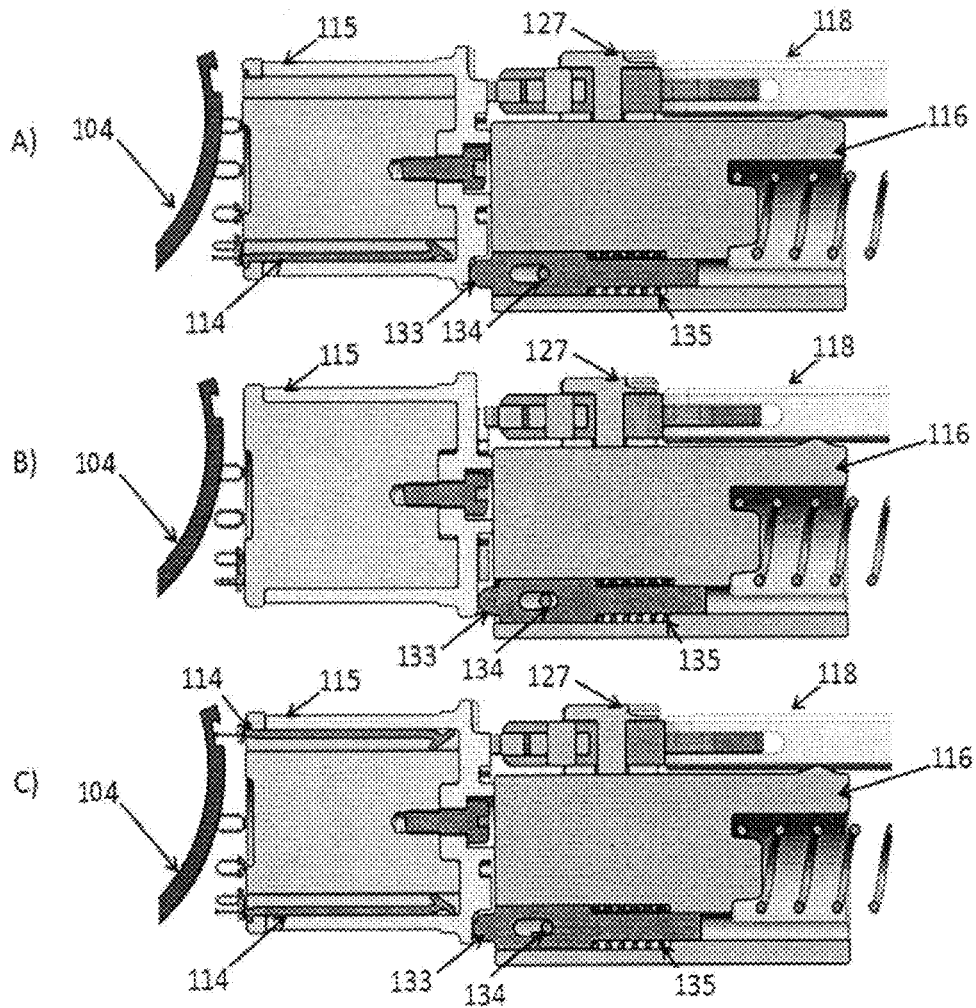
Figure 49: Cartridge Advancement Sequence (Side View)
