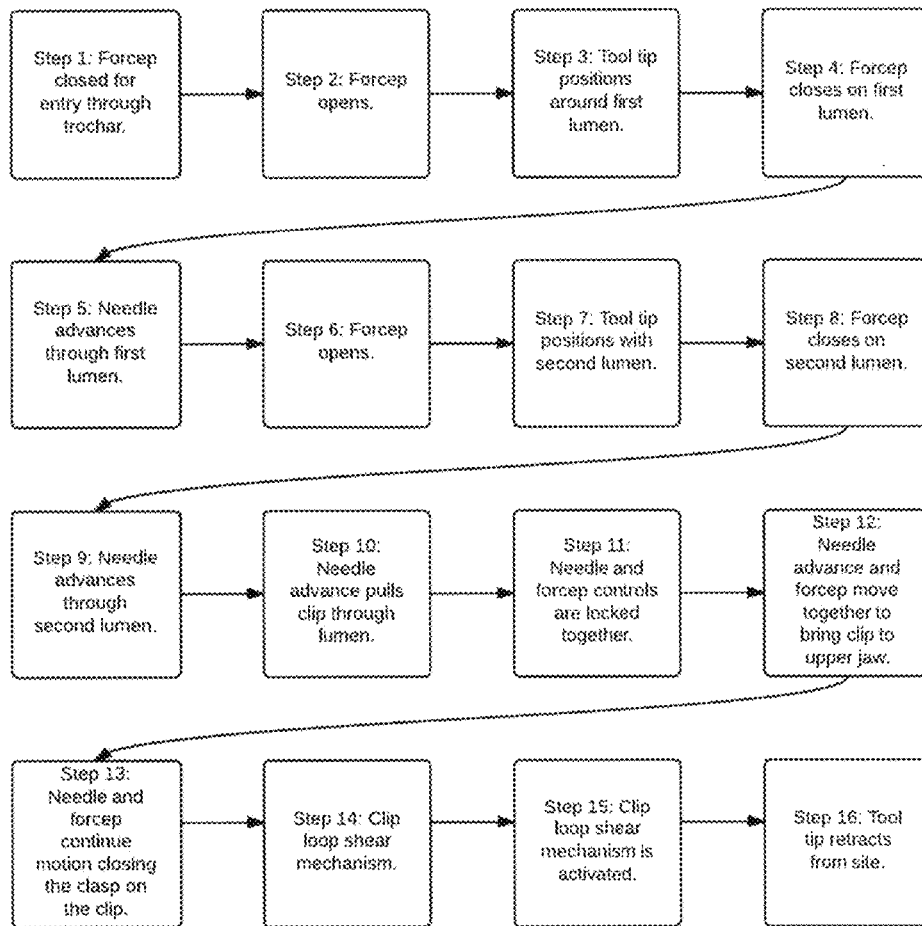
Figure 21: Sequence of Operation for the Clipping Method
