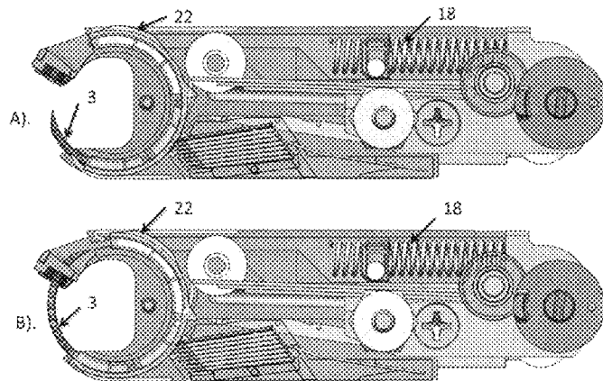
Needle Advancer Arm Actuation
