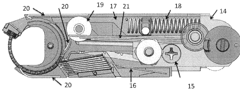
Figure 7: Clipping Tool Tip Cross-Sectional View #1
