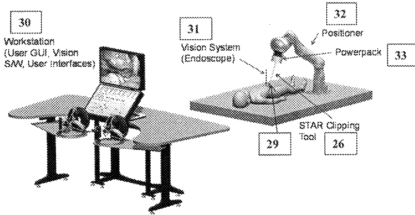
Figure 23: Overview of the Clipping System Robotic Embodiment
