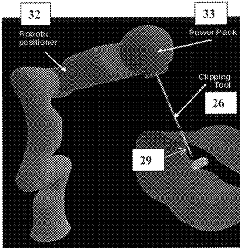
Figure 25: Robot-driven Embodiment of the Clipping Apparatus
