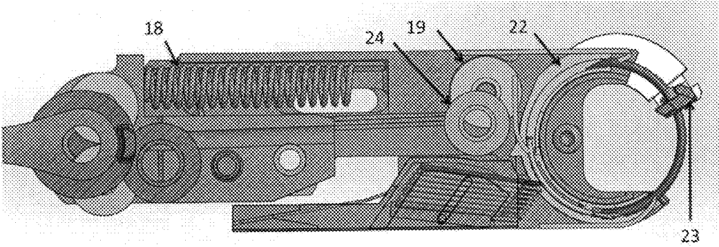
Figure 9: Clipping Tool Tip Cross-Sectional View #2
