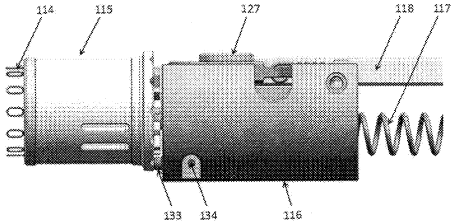
Figure 46: Clip Cartridge Advancement Mechanism (Side View)
