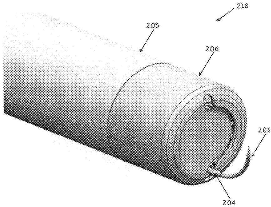
Figure 54 : Shape Memory Alloy Needle Clipping Tool Tip
