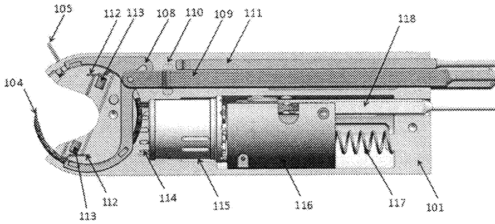
Figure 33: Clipping Tool Tip Cross-Sectional View #1
