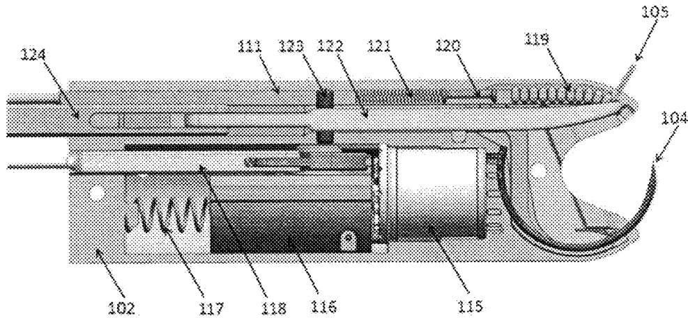
Figure 35: Clipping Tool Tip Cross-Sectional View #2
