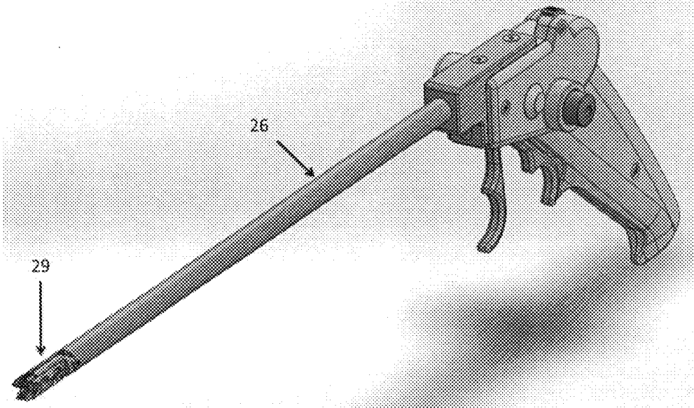
Figure 26: Manual/Handheld Embodiment of the Clipping Apparatus
