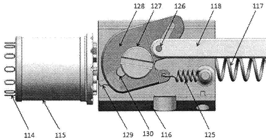
Figure 44: Clip Cartridge Advancement Mechanism (Top View)
