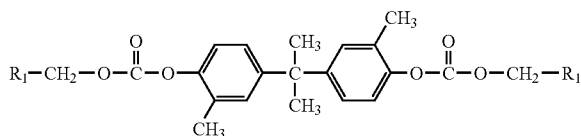
Formula (III)
