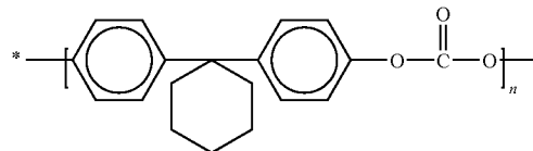
Formula (B)
