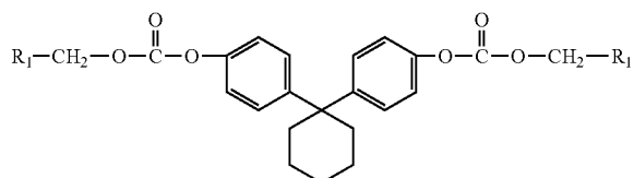
Formula (IV)
