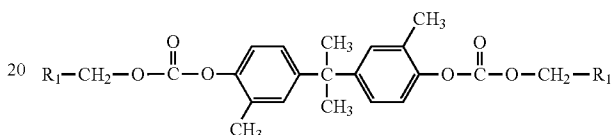
Formula (IV)
