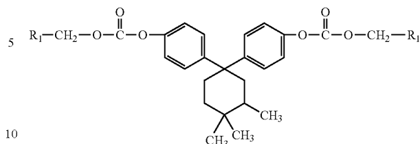
Formula (V)
