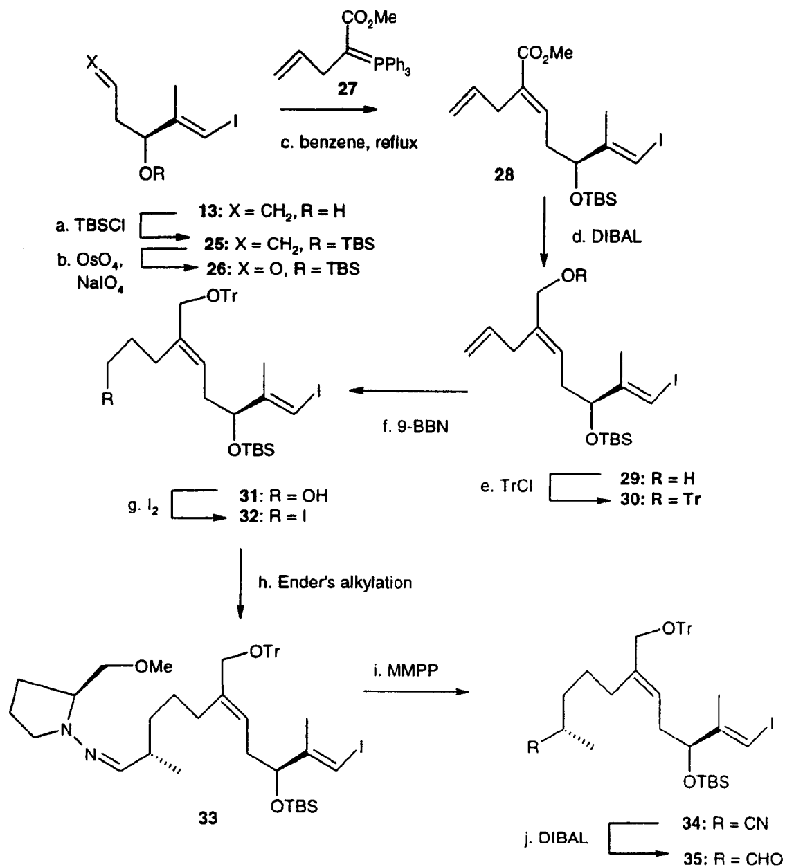
—Scheme 7:
