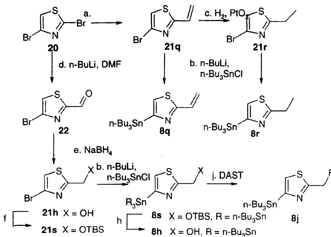
—Scheme 5:
