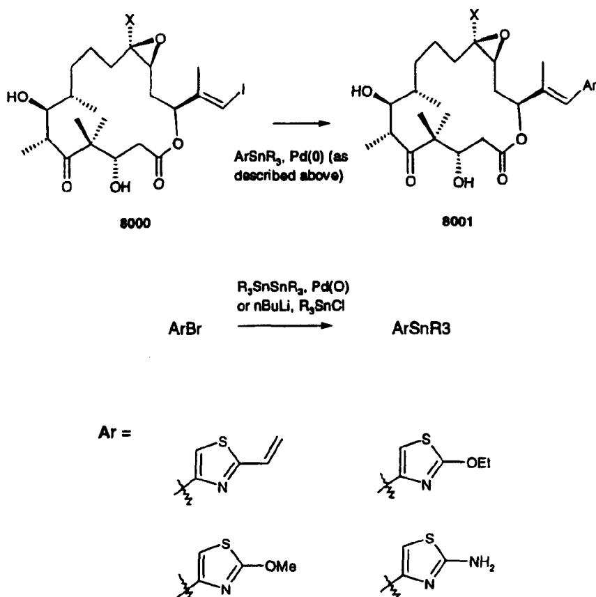
—Scheme 12:
