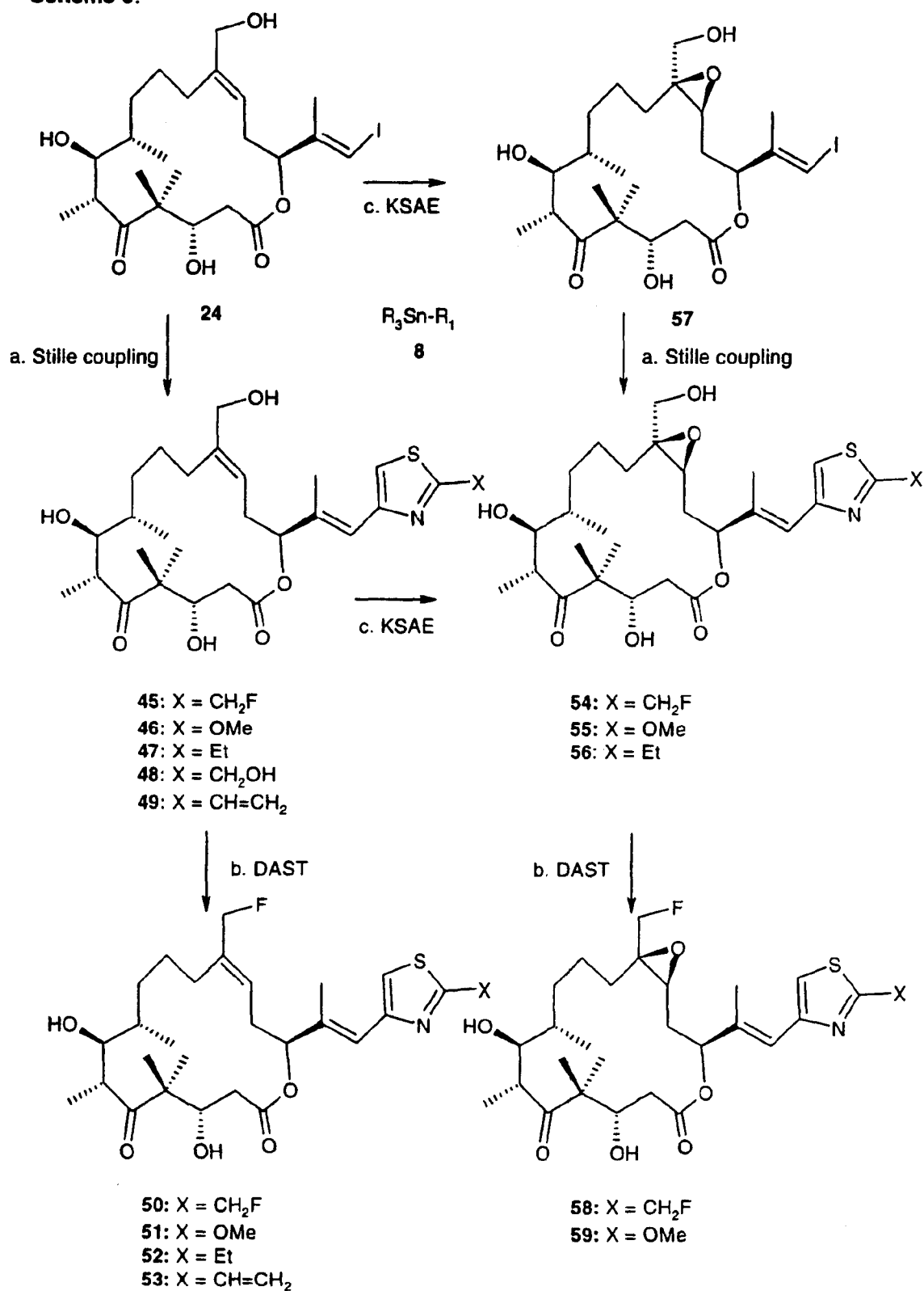
—Scheme 9:
