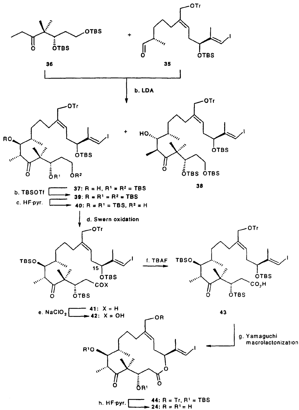
---Scheme 8:
