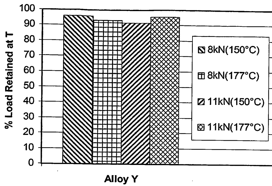
Figure 9: BLR behaviour at temperature for Alloy Y.
