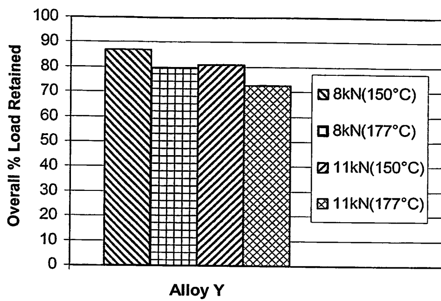
Figure 8: Overall BLR behaviour for Alloy Y.
