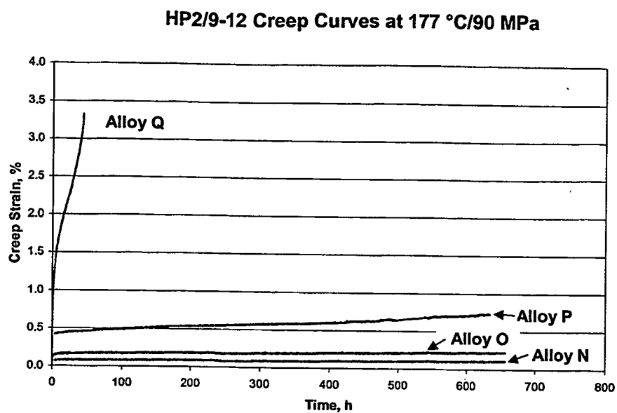
Figure 7 Creep curves at 177°C and 90 MPa showing the influence of increasing Al content (from 0.05 wt.% in Alloy N, to 0.09 wt.% in Alloy O, to 0.12 wt.% in Alloy P, to 0.23 wt.% in Alloy Q) on the creep behaviour.
