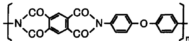
FIG. 10A POLYPYROMELLITICIMIDE (POLYIMIDE PRODUCED BY DEGENERATIVE REACTION)
