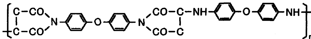
FIG. 10B POLYAMINOBISMALEIMIDE (POLYIMIDE PRODUCED BY ADDITIONAL REACTION)
