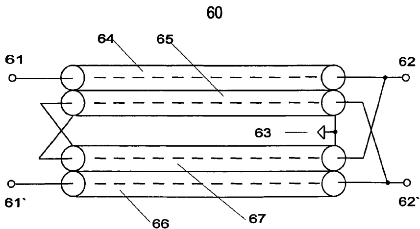
FIG.6 PRIOR ART
