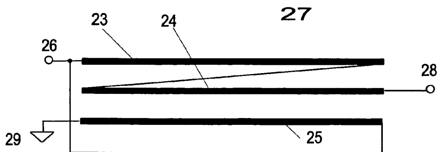
FIG.3 PRIOR ART
