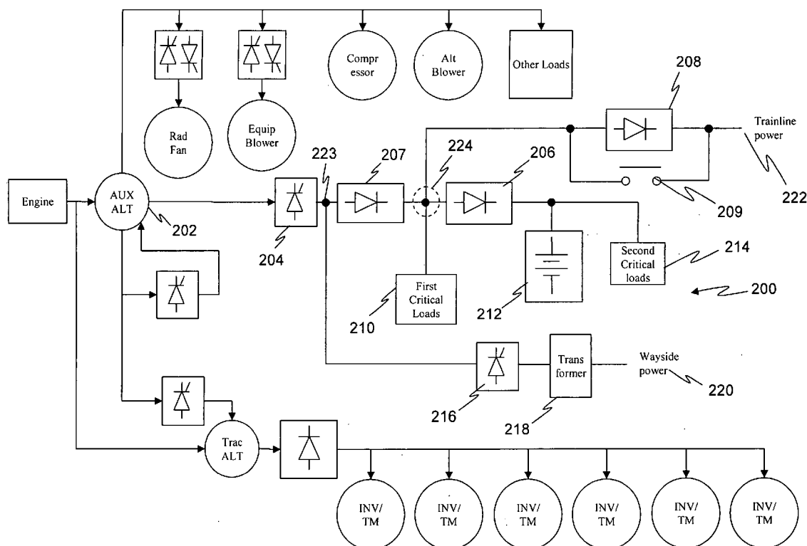
Battery Charger Trainline
