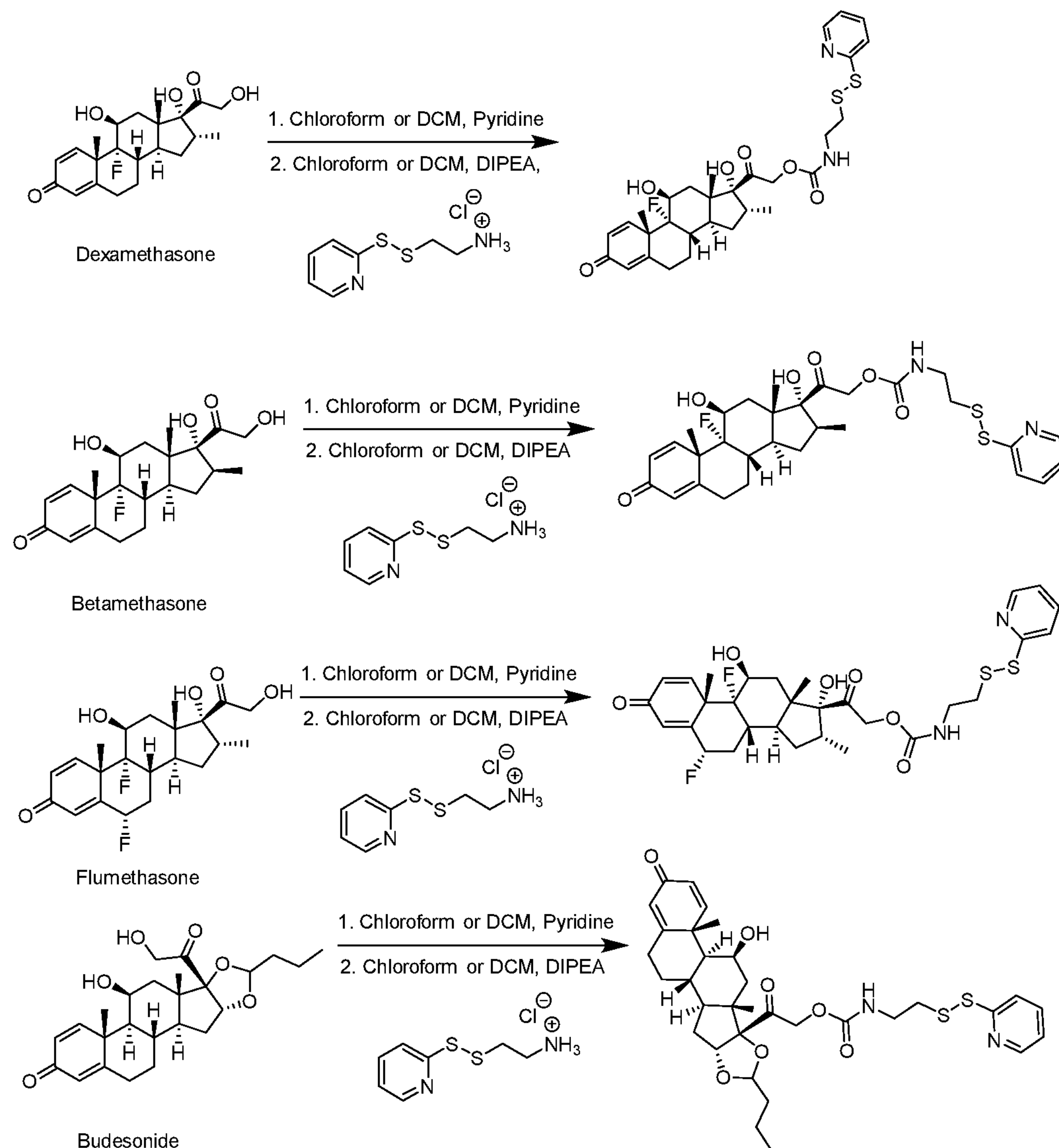
Scheme 7 - Synthetic Scheme of Steroid-Carbamate-Pyridyl Disulfide Compounds
