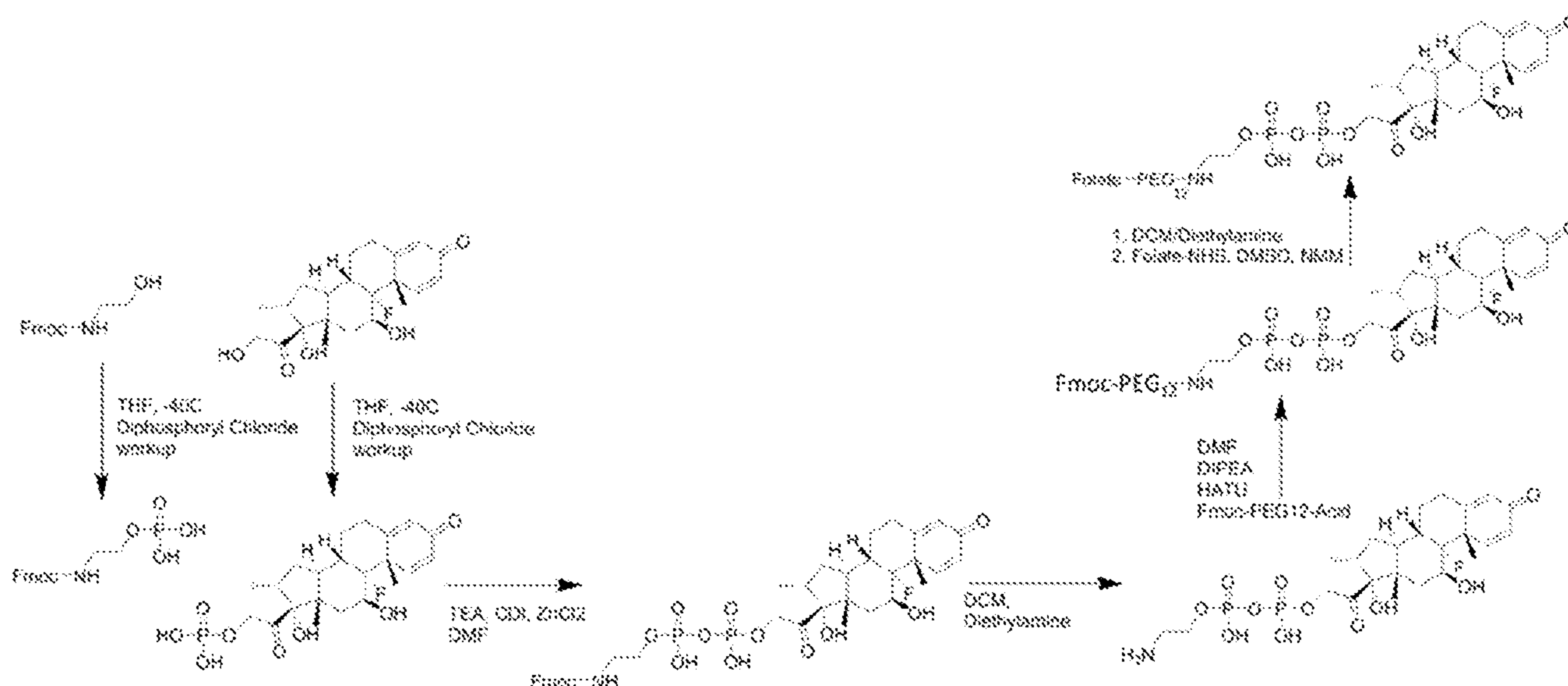
Scheme 12 - Synthetic Scheme of Compound 108 (Folate-PEG12(CH 2 )-Pyrophosphate-Dexamethasone)
