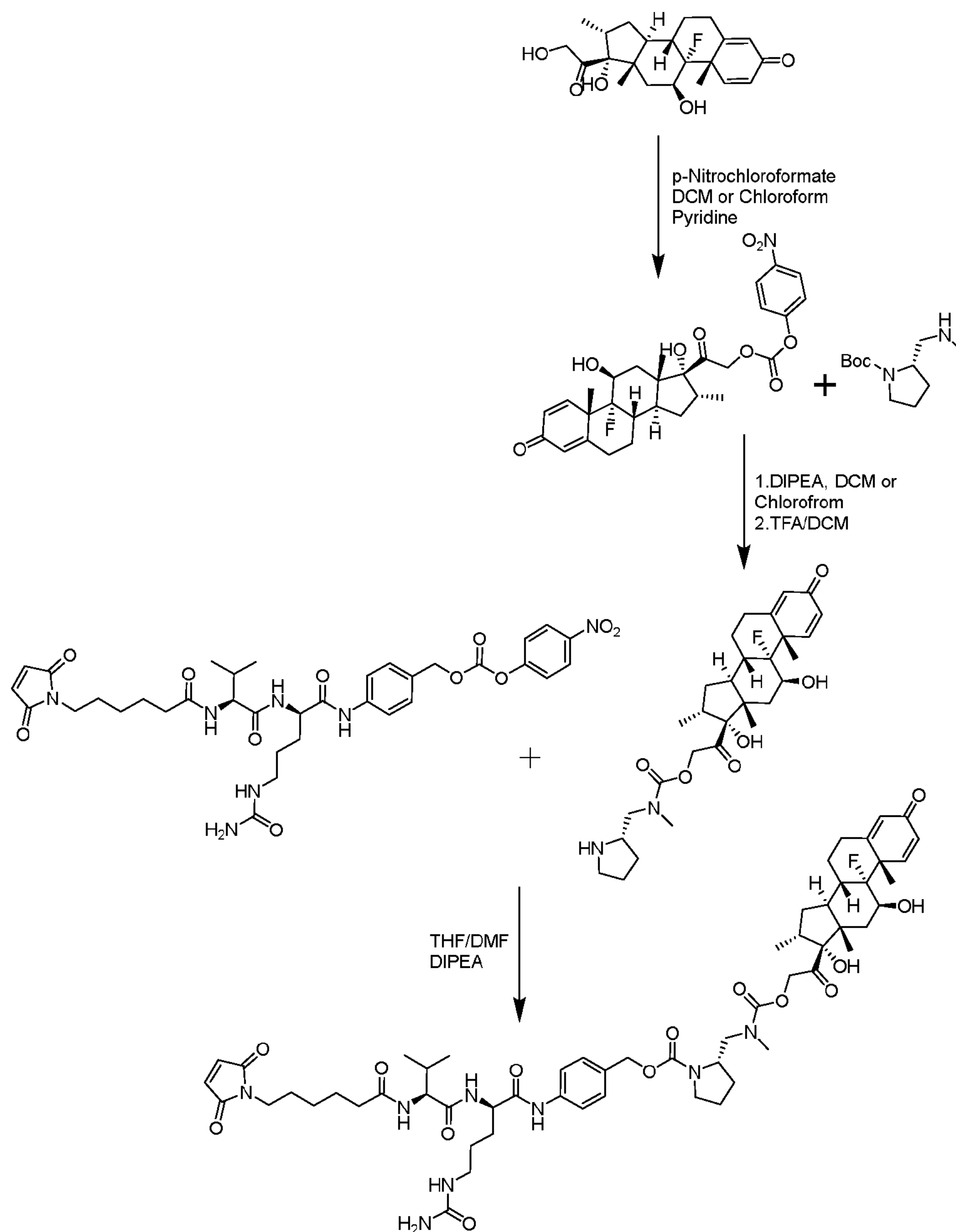
Scheme 10 - Synthetic Scheme for Maleimide-CathepsinBCleavable-Dicarbamate-Dex
