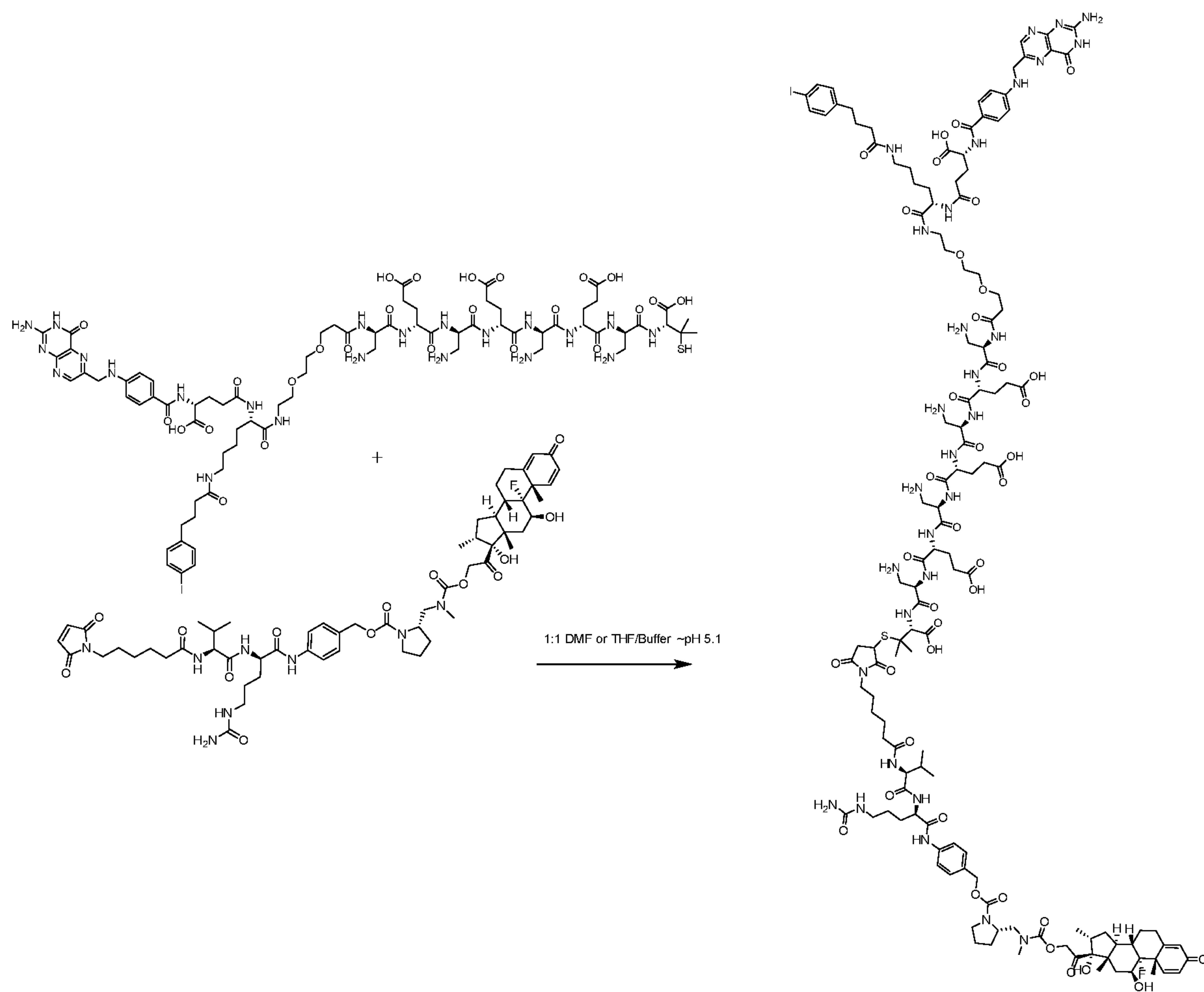
Scheme 11 - Synthesis of Compound 125 (Fol-Alb-PEG2-Hydrolink-DimethylCysteine-Maleimide- (CH_2)_5 -CathepsinBCleavable-Dicarbamate-Dexamethasone)
