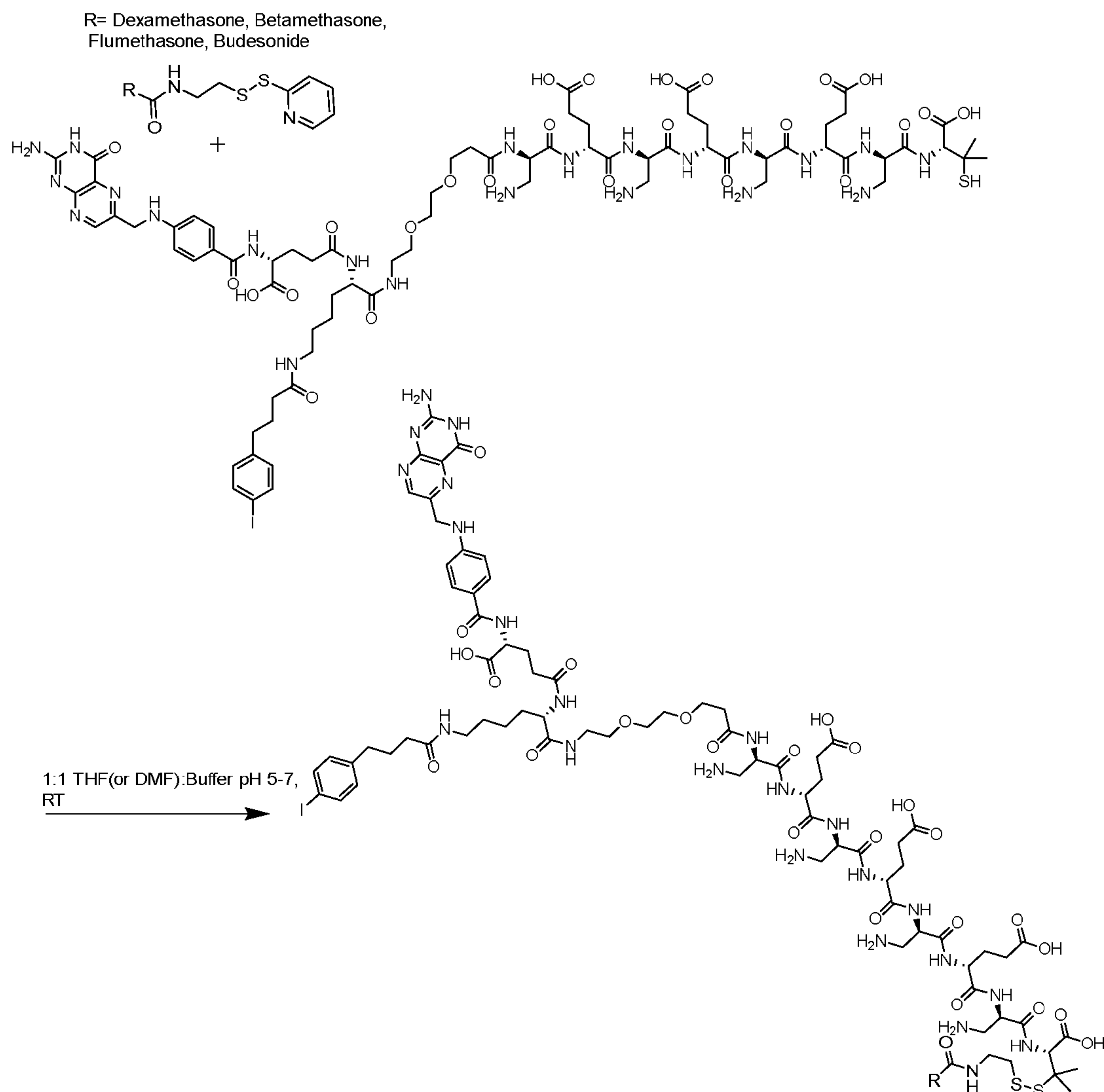
Scheme 8 Final DimethylCys-Maleimide Coupling of Compounds.
