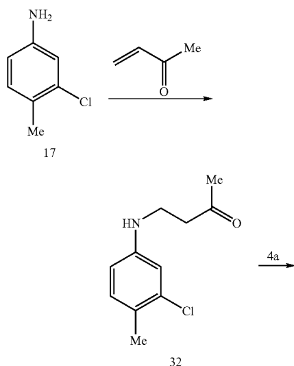
SCHEME 7
