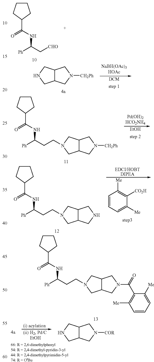
SCHEME 1
