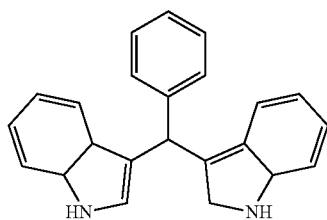
3-((2,7a-dihydro-1H-indol-3-yl)(phenyl)methyl)-3a, 7a-dihydro-1H-indole
