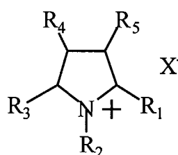
Pyrrolidinium
