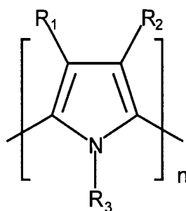
Polypyrrole
