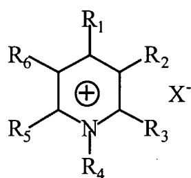
Pyridinium
