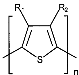
Polythiophene
