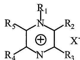
Pyrazinium
