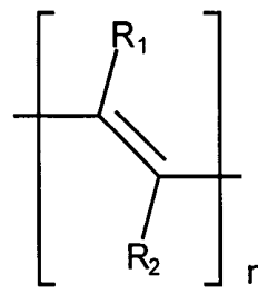
Polyacetylene
