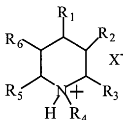
Piperidinium
