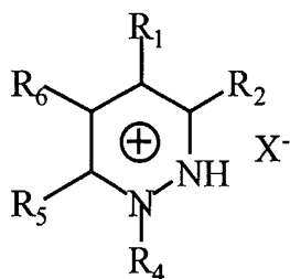
Pyridazinium
