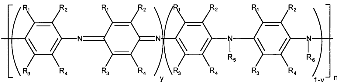
Polyaniline
