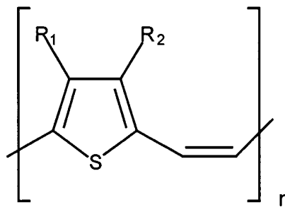
Polythiophenevinylene
