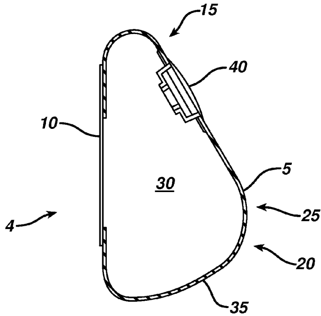
FIG. 1 PRIOR ART
