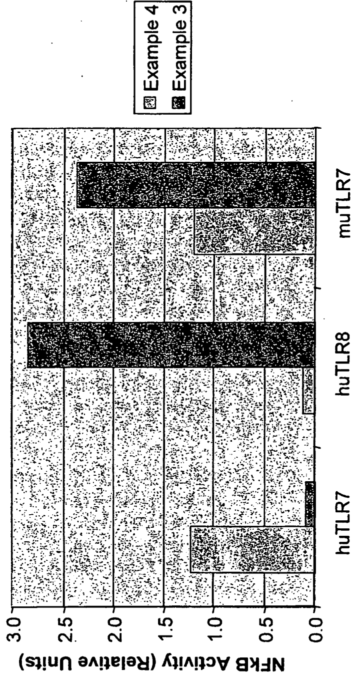
FIG. 1 TLR7/8 Selectivity
