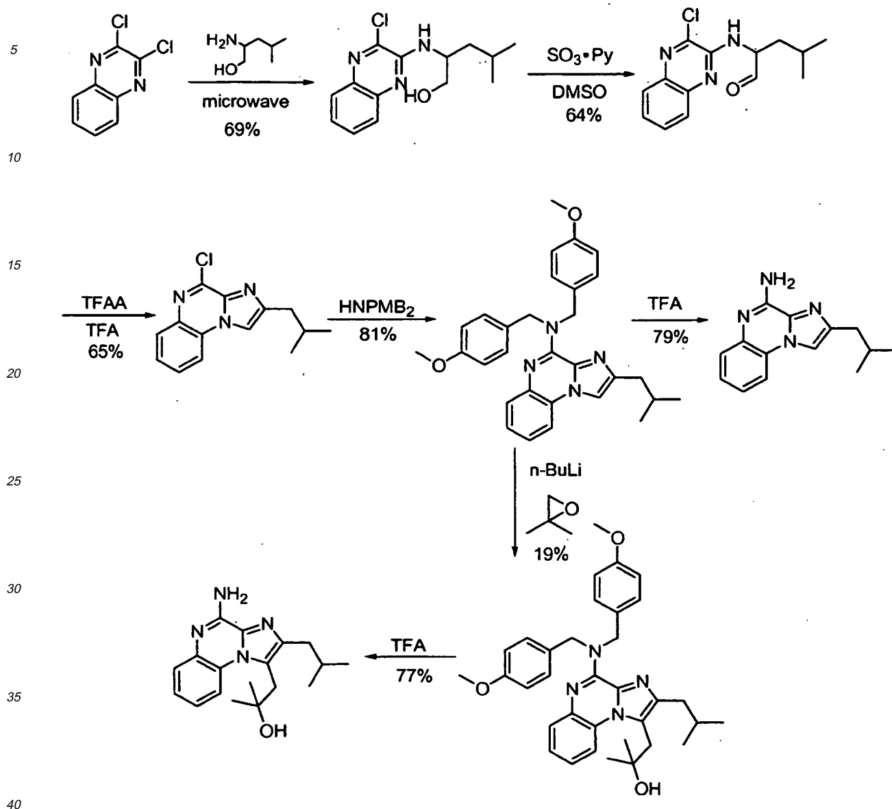
Scheme 4
