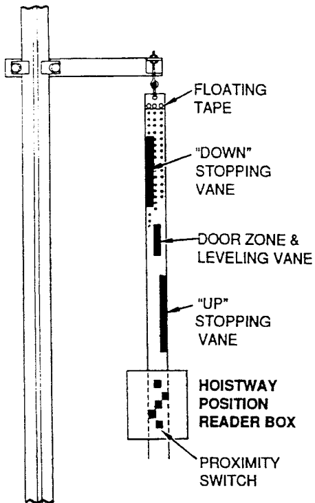
fig. 2 PRIOR ART
