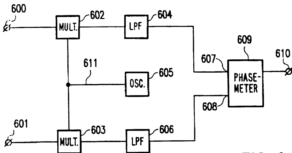
FIG. 6 PRIOR ART
