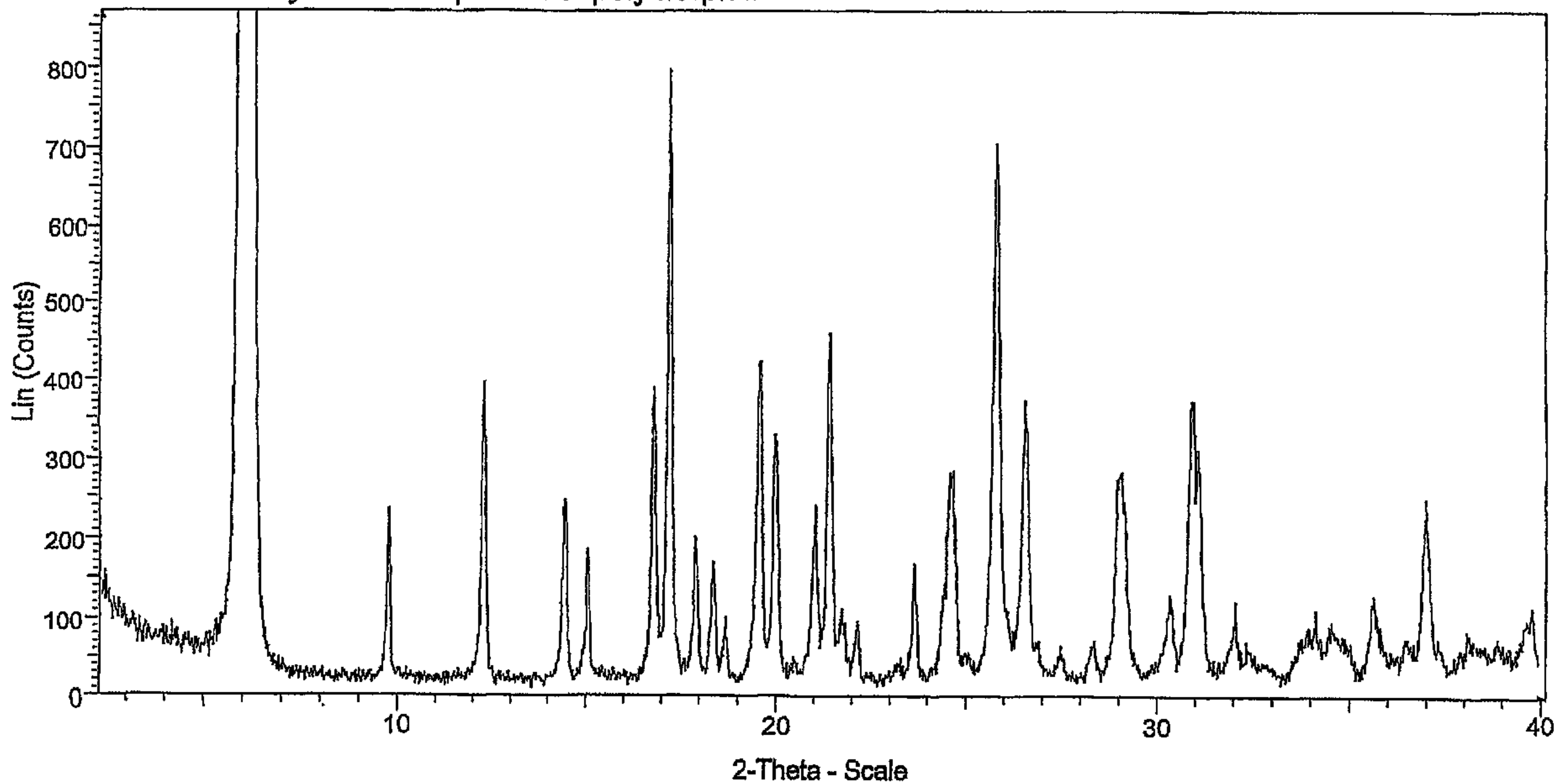
X-ray diffraction pattern of polymorph B
