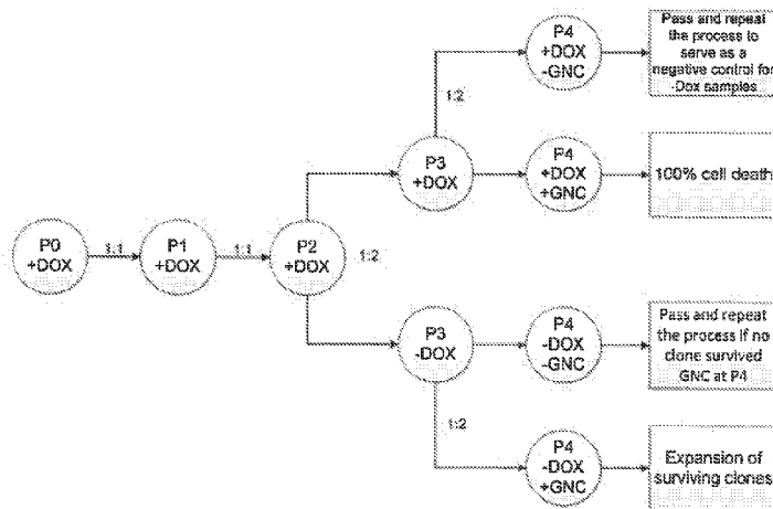
Figure 1. Procedure of iPSC colonies expansion and analysis
