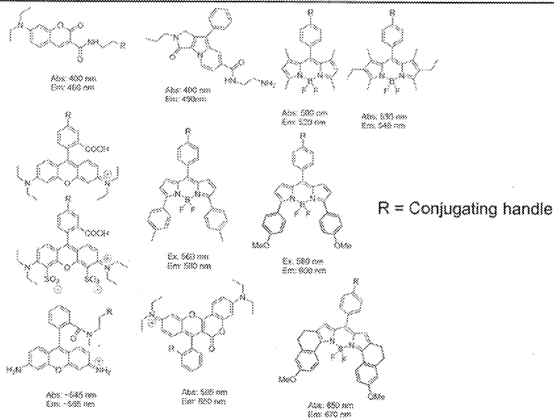
FIGURE 30 Amino Acid Fluorophores
