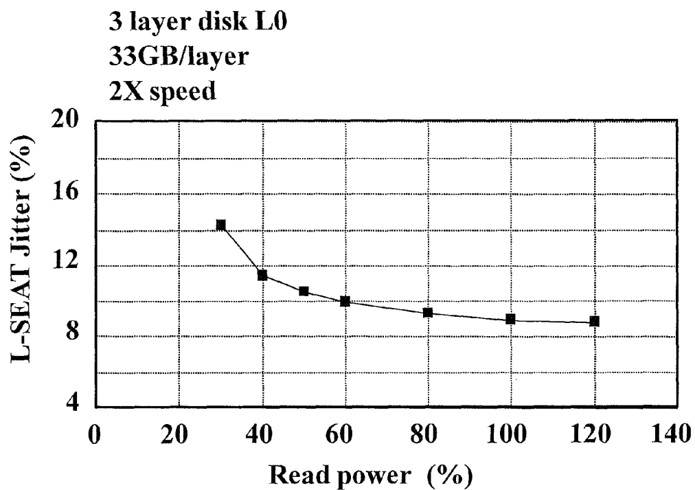
(a) Jitter
