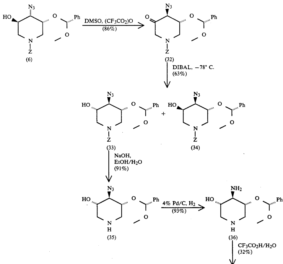
Scheme E: Synthesis of 3-amino-1,5-iminosugars.
