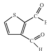
2,3-thiophenedicarboxaldehyde
