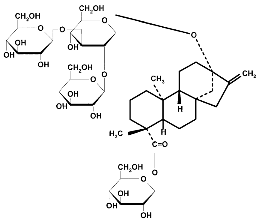
Rebaudioside A
