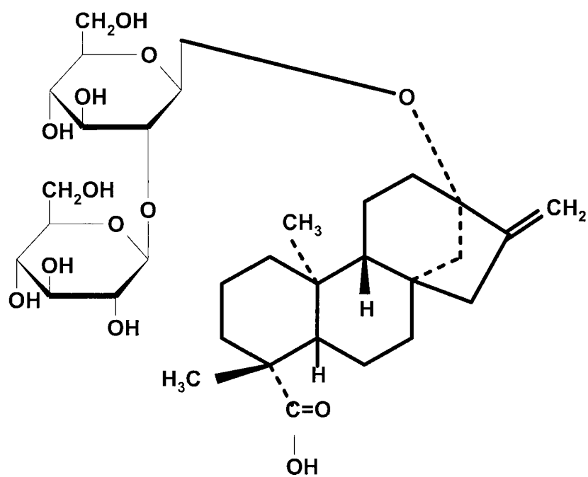
Steviolbioside
