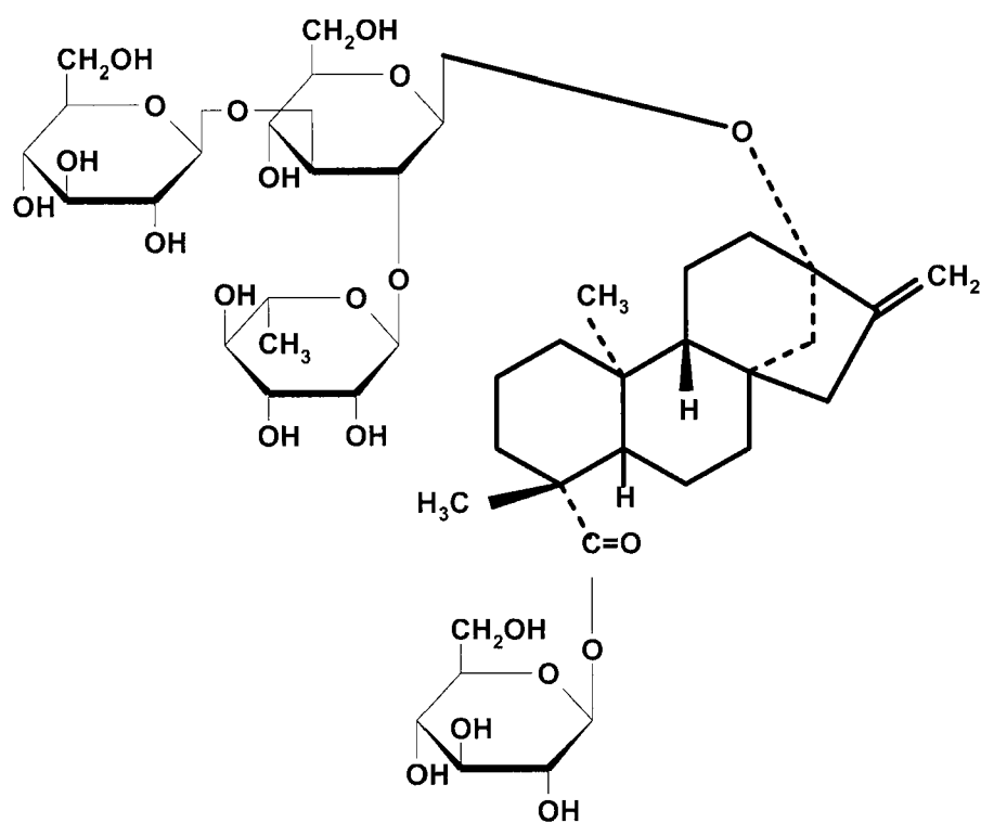
Rebaudioside C
