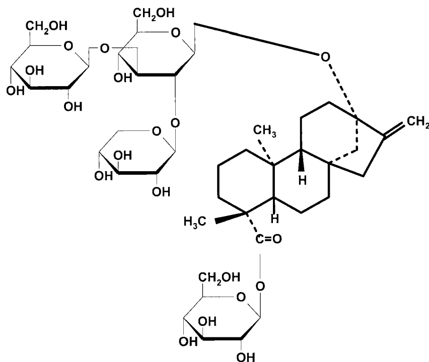
Rebaudioside F
