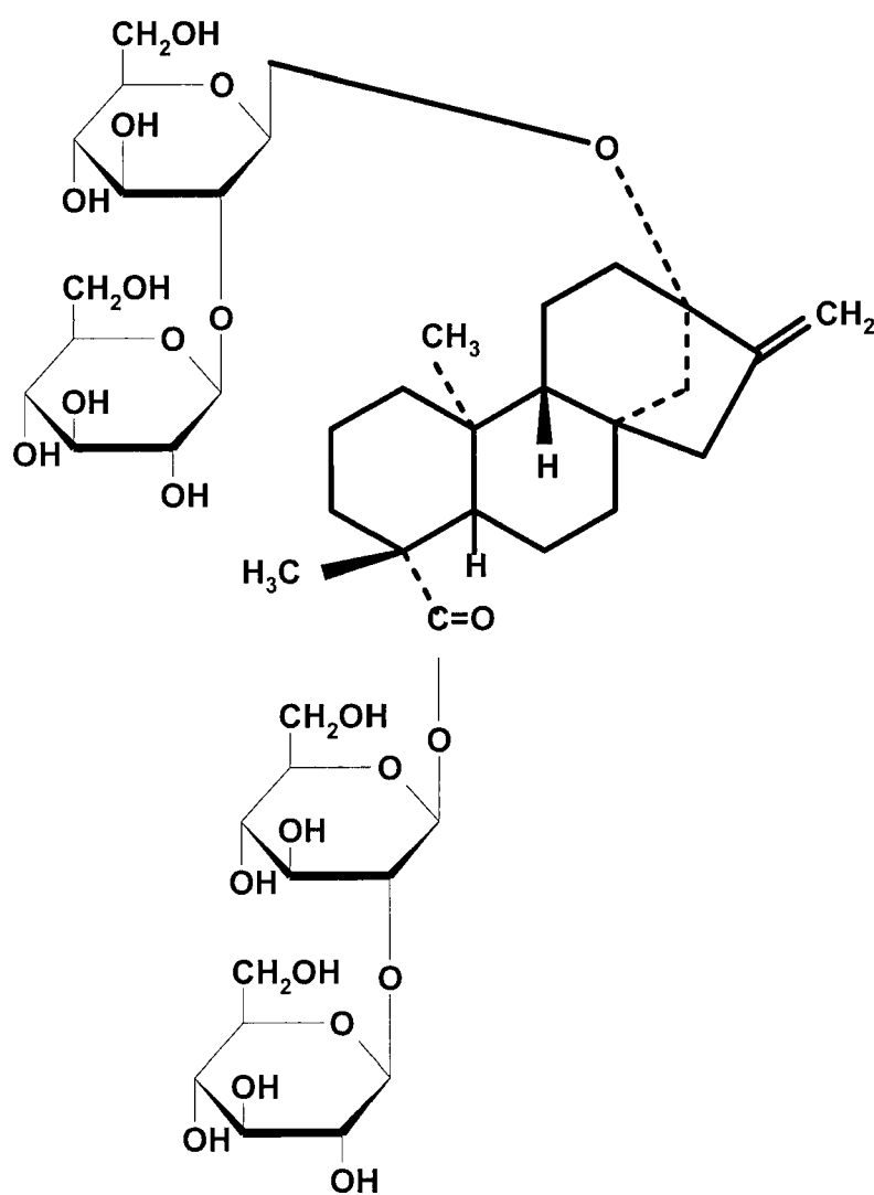
Rebaudioside E
