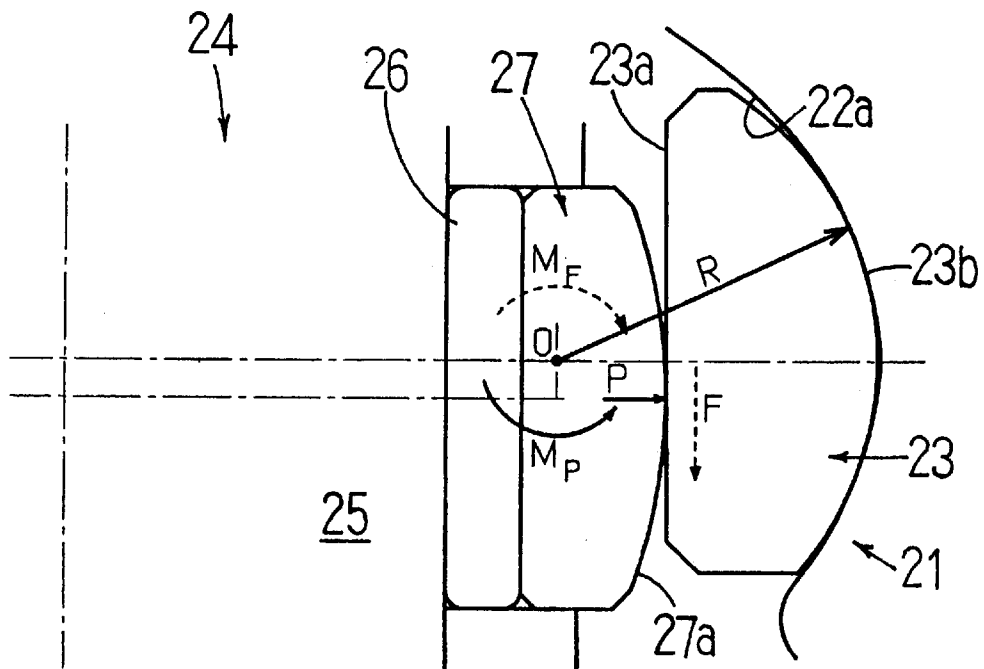
FIG.17 PRIOR ART
