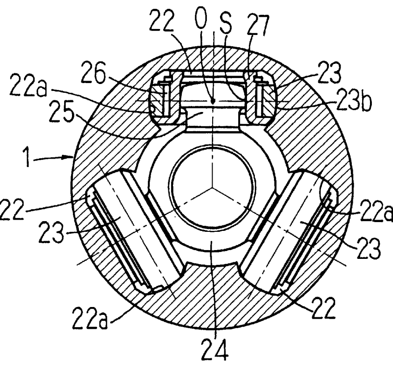
FIG.20 PRIOR ART
