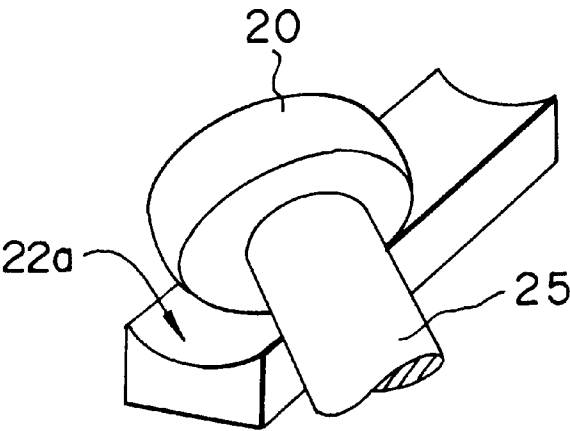
FIG. 12 PRIOR ART
