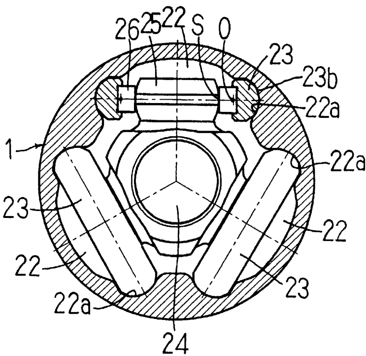
FIG. 19 PRIOR ART
