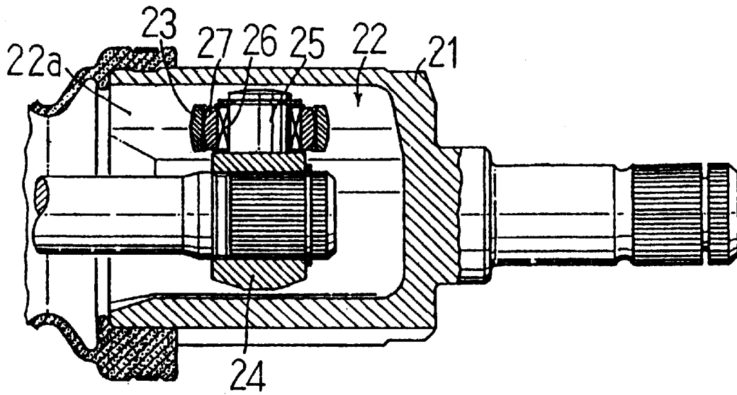
FIG.13 PRIOR ART
