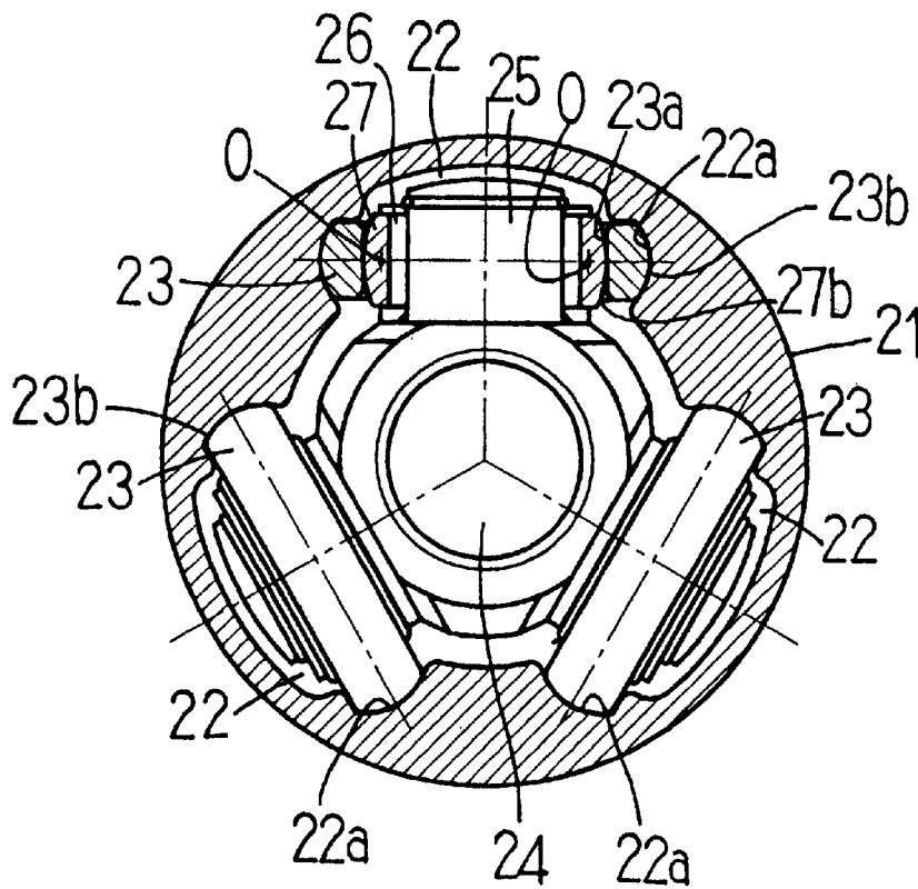
FIG.14 PRIOR ART
