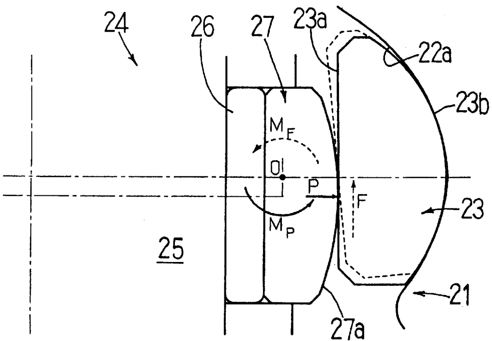
FIG.17 PRIOR ART
