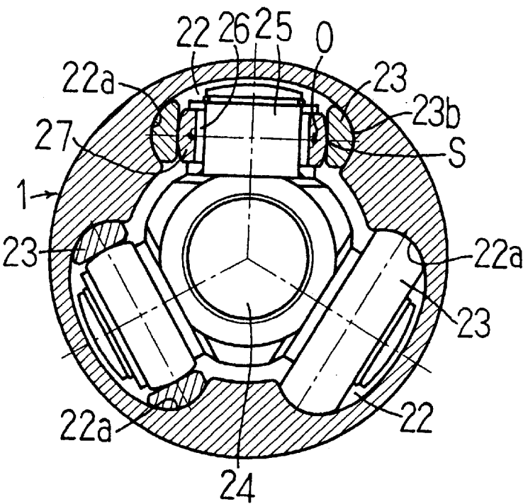
FIG. 19 PRIOR ART
