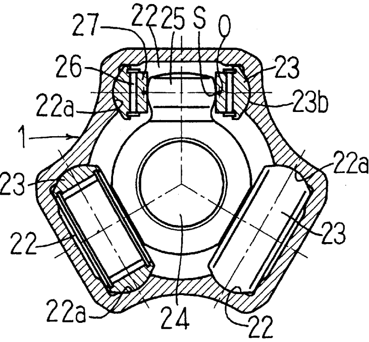
FIG.21 PRIOR ART
