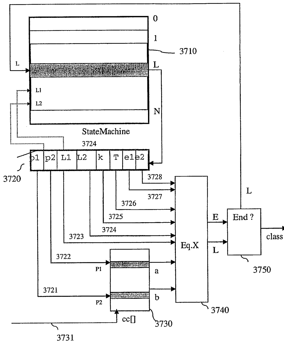
Figure 3h State machine
