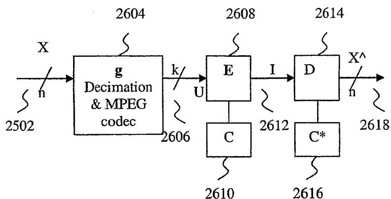
Figure 2g Gersho NLIVQ '90 adapted to interpolation of MPEG coded video
