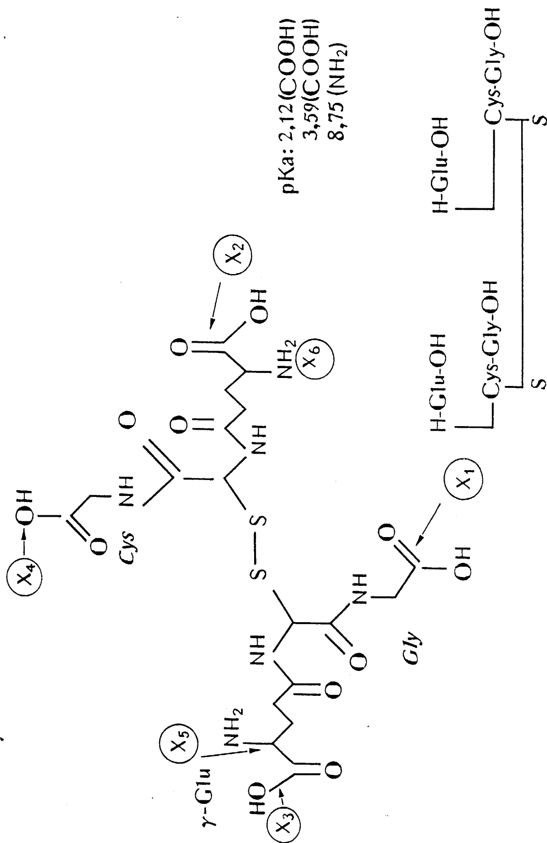
Glutathione oxidized
