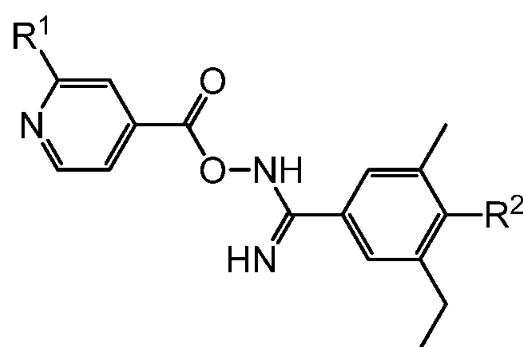
Structure 1
