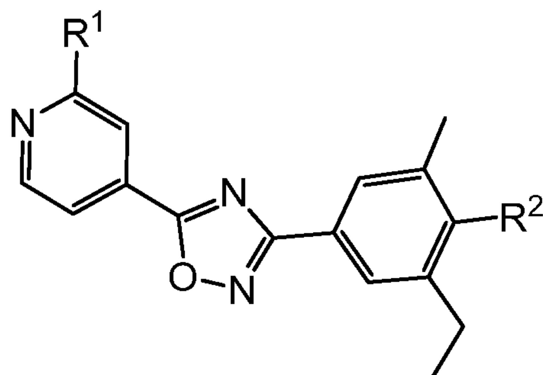
Formula (I)
