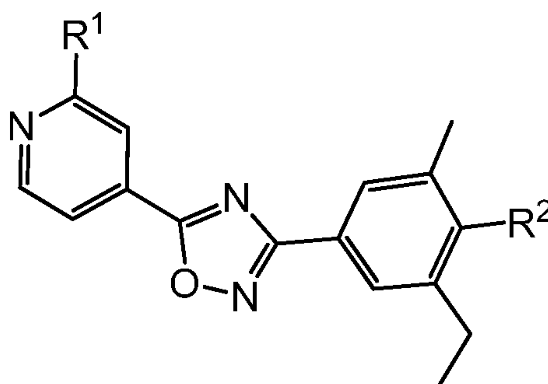
Formula (I)
