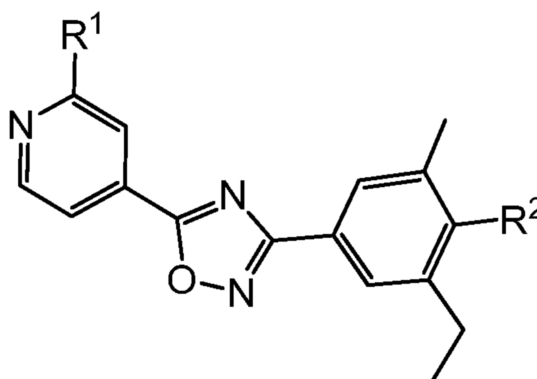
Formula (I)
