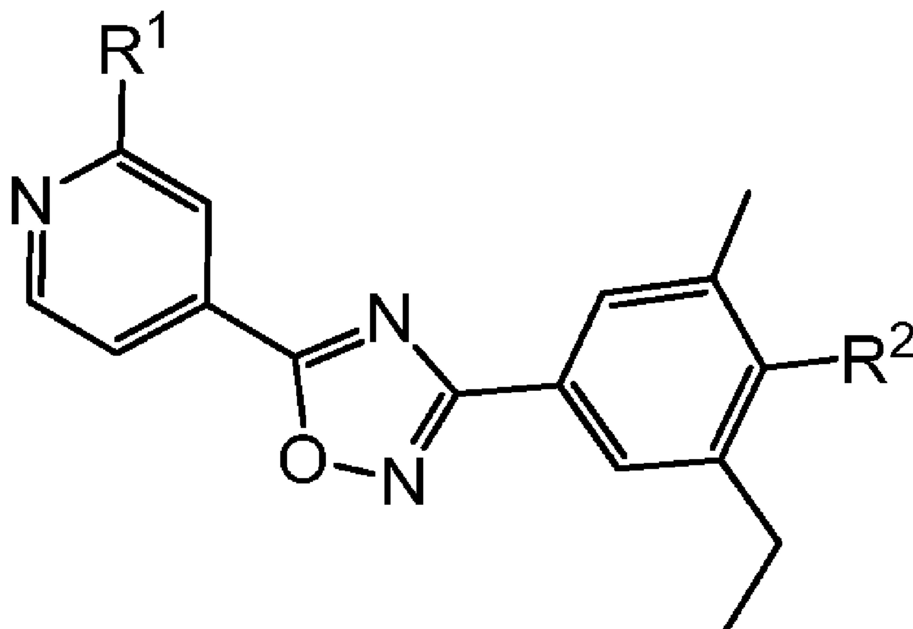
Formula (I)
