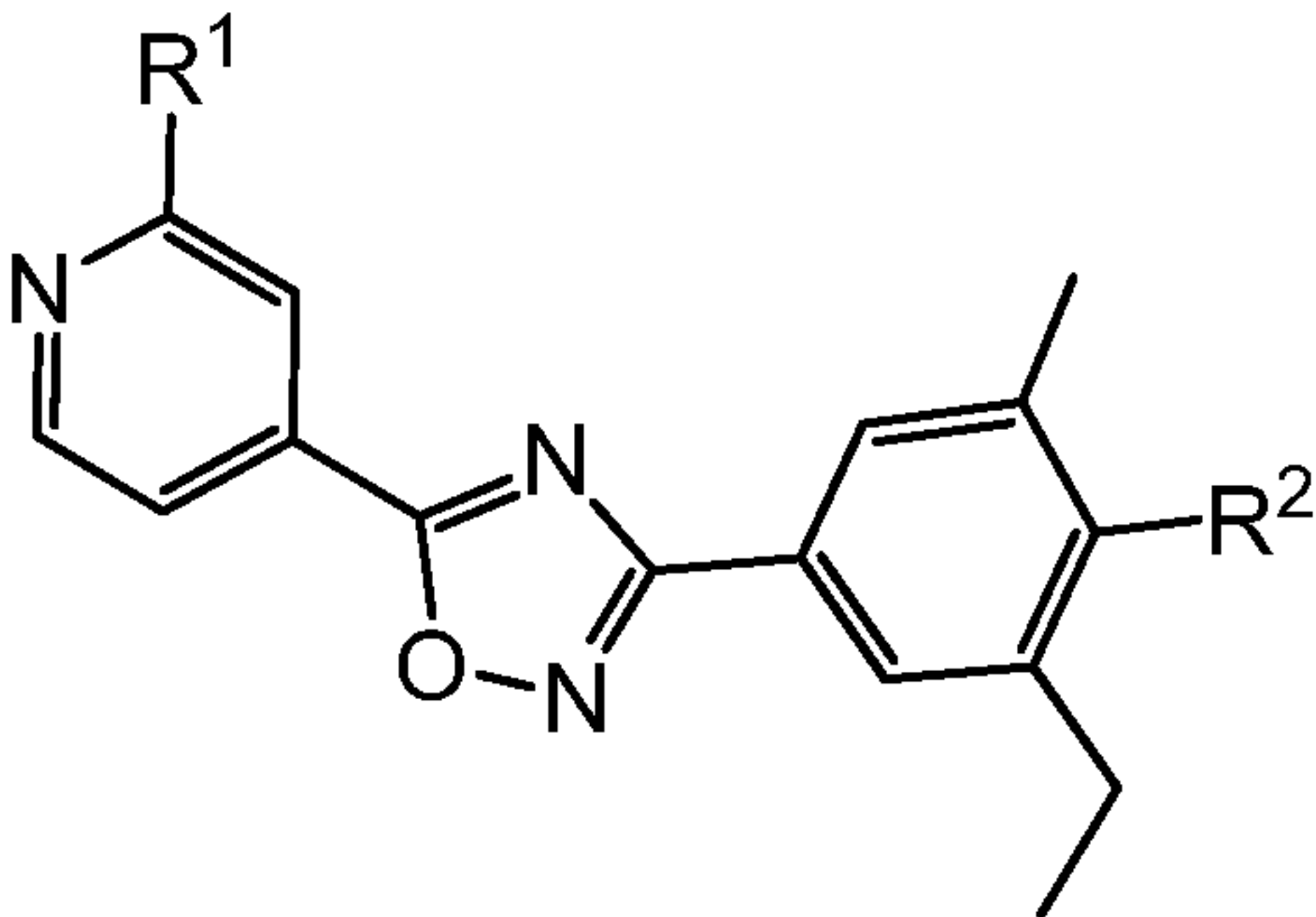
Formula (I)
