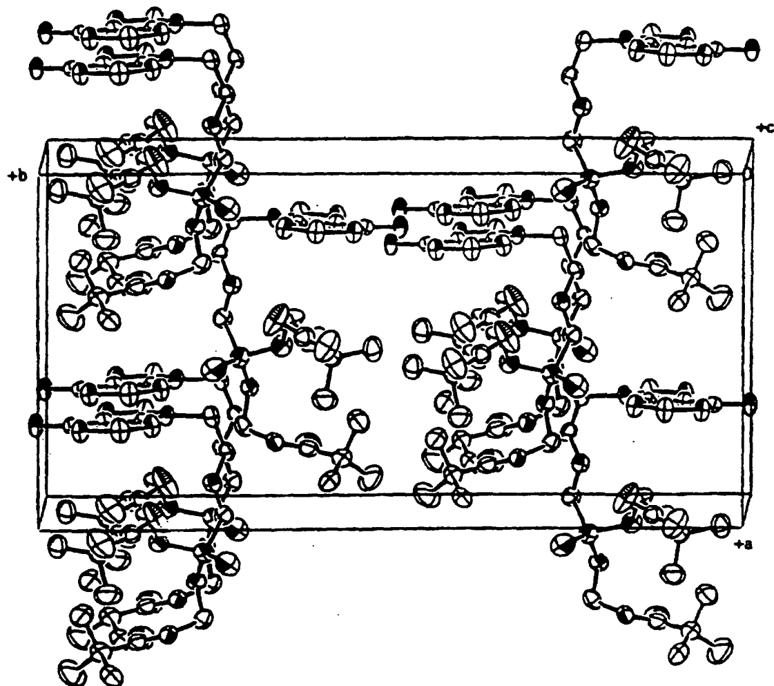
Packing diagram showing unit cell of Form 1 AD.
