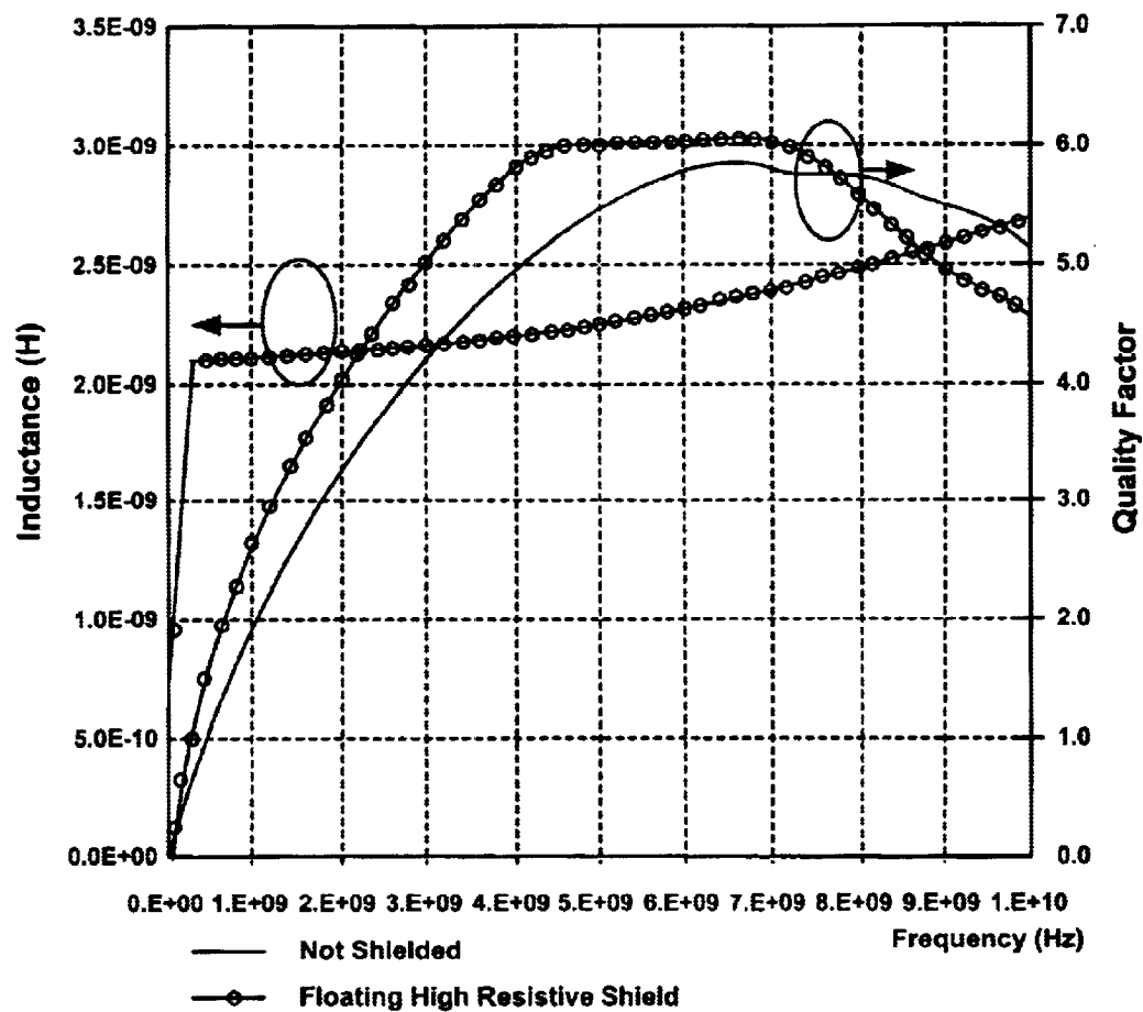
Quality Factor and Inductance Plots of Unshielded Inductor and Inductor with High Sheet Resistance Floating Polysilicon Shield
