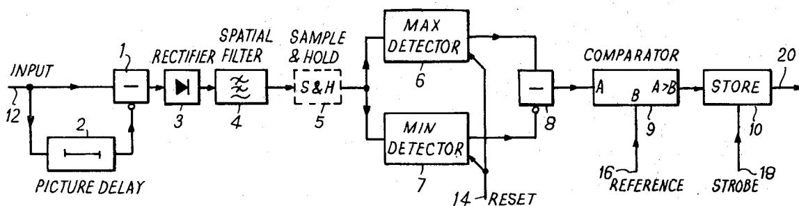
GENERAL REALISATION OF THE MOVEMENT DETECTOR
