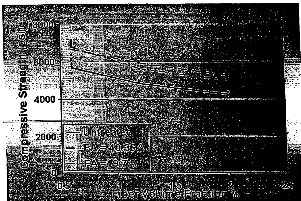
Figure 7 shows a comparative data of the compressive strength of mineral based materials for a period of twenty-eight days. The figure illustrates that treated fibers have an improved compressive strength as compared to the untreated fibers.
