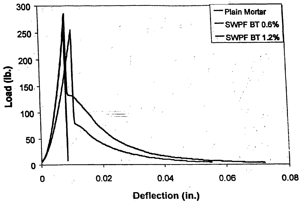
Figure 4 Load vs. deflection curve for unreinforced and treated softwood (SF) fiber reinforced mortars.
