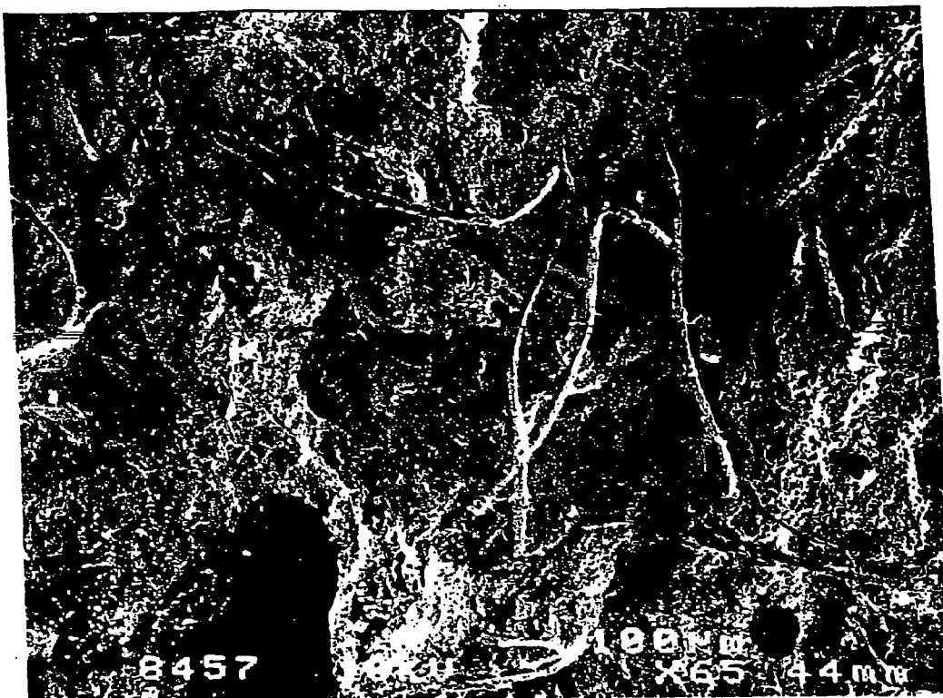
Figure 3 After treatment (beating and adsorption of fly ash), softwood pulp fibers added to mortar at a volume fraction of 1.2% show uniform dispersion. (Compare to untreated fibers in Fig.1)
