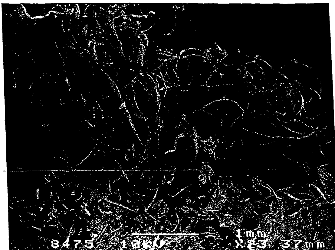
Figure 1 Poor distribution of untreated softwood fibers, added at a volume fraction of 1.7% to a portland cement mortar.
