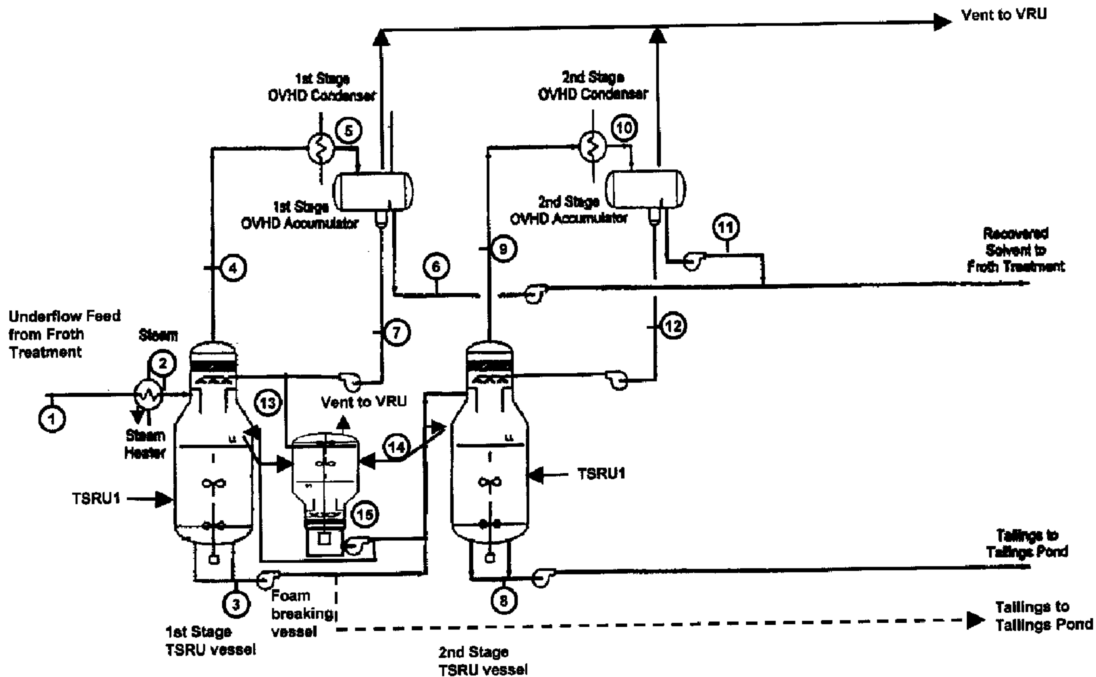
Tailings Solvent Recovery Unit
