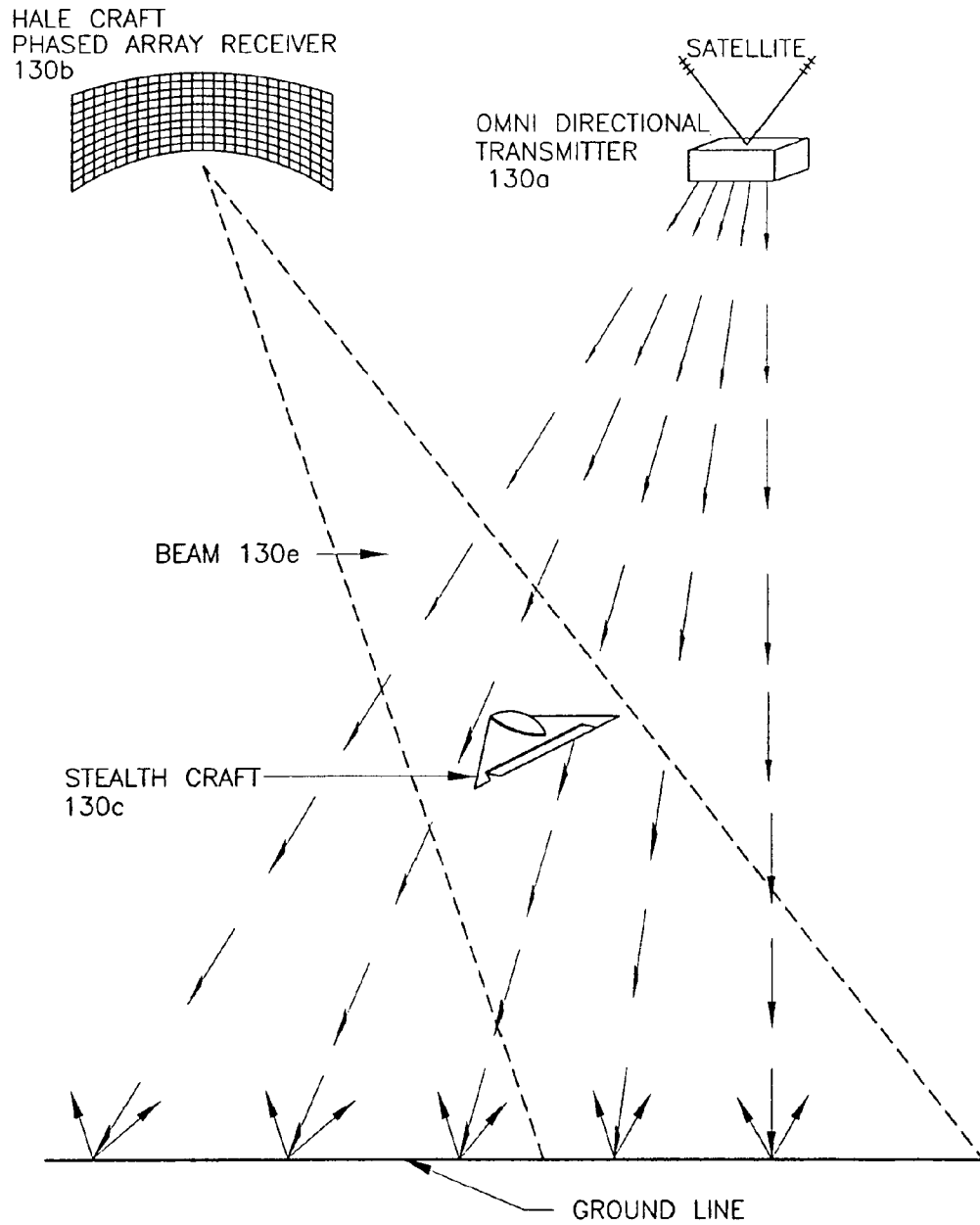
DETECTING A STEALTH CRAFT WITH OMNI DIRECTIONAL TRANSMITTER AND SEPARATE RECEIVER
