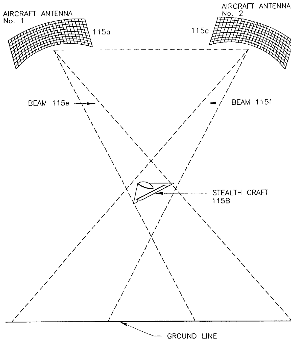
DETECTING DISTANCE TO STEALTH CRAFT BY TRIANGULATION
