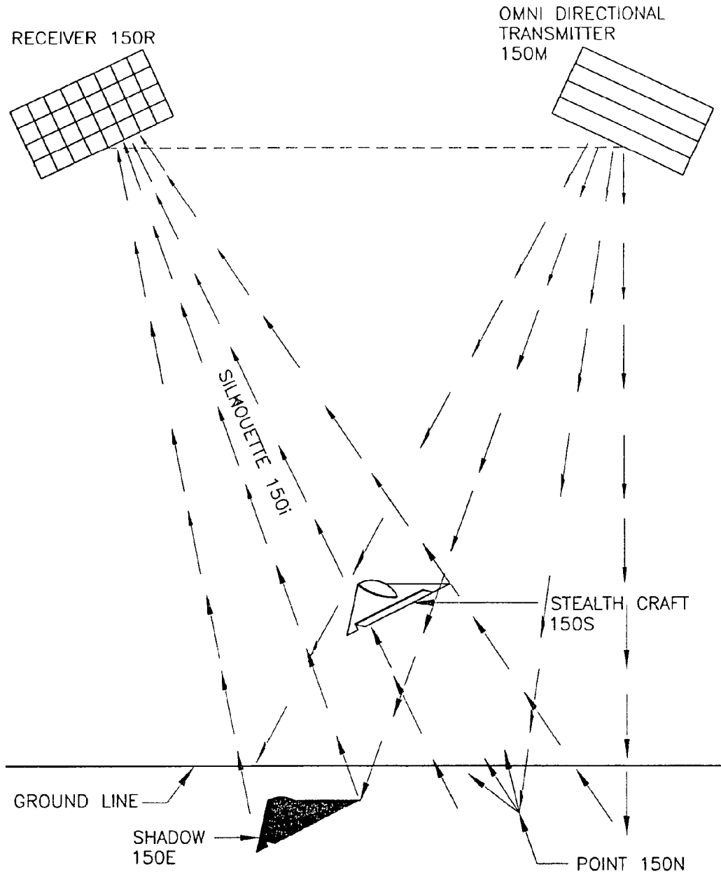
DETECTION AND DISTANCE DETERMINATION WITH ONE TRANSMITTER AND ONE RECEIVER USING BOTH SILHOUETTE AND SHADOW
