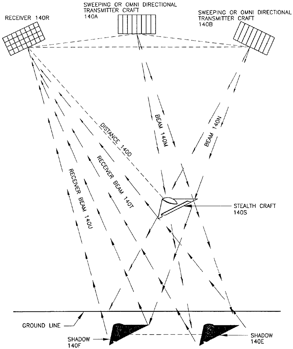
DETECTION AND DISTANCE DETERMINATION WITH TWO TRANSMITTERS AND ONE RECEIVER USING SHADOWS FIG. 9
