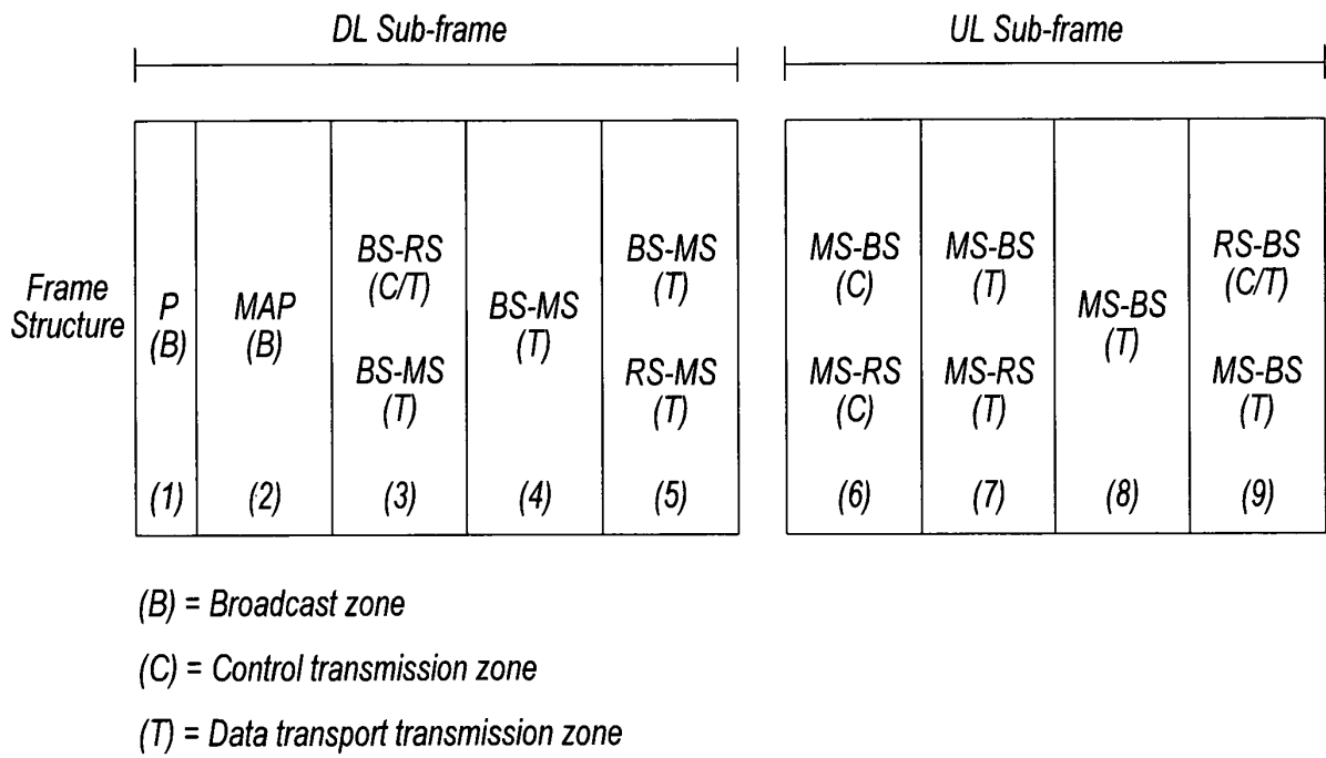
Fig. 1 Frame Structure
