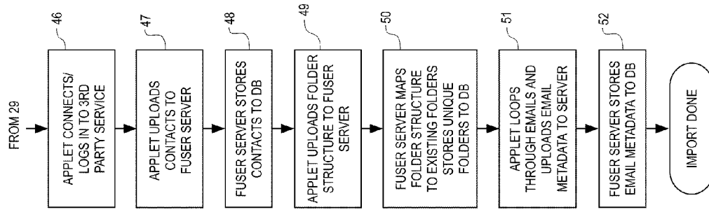
Fig. 10 INITIAL ACCOUNT IMPORT
