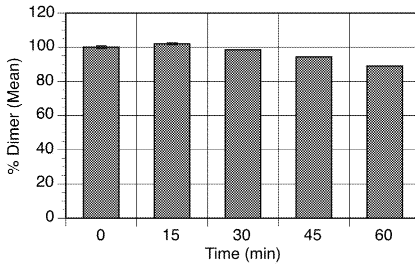
Figure 2 Metabolic stability of acetaminophen dimer
