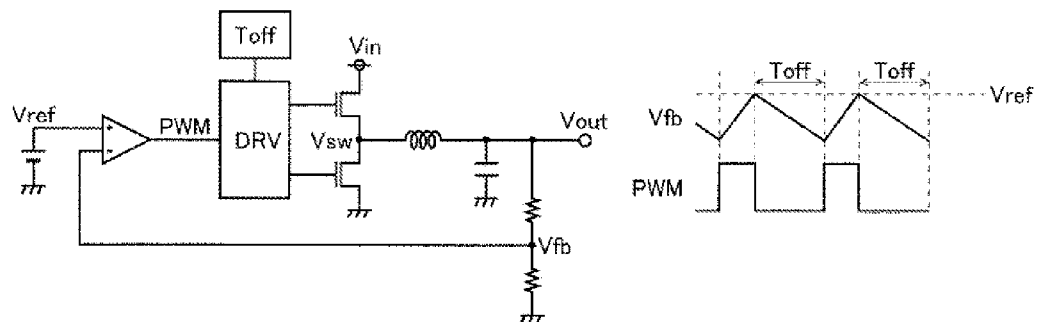
FIG. 14C PRIOR ART
