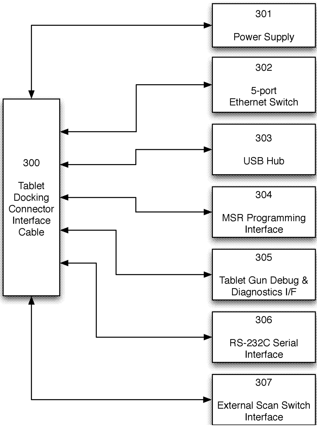
Primary Electronics Printed Circuit Board Functional Block Diagram (PCB2)
