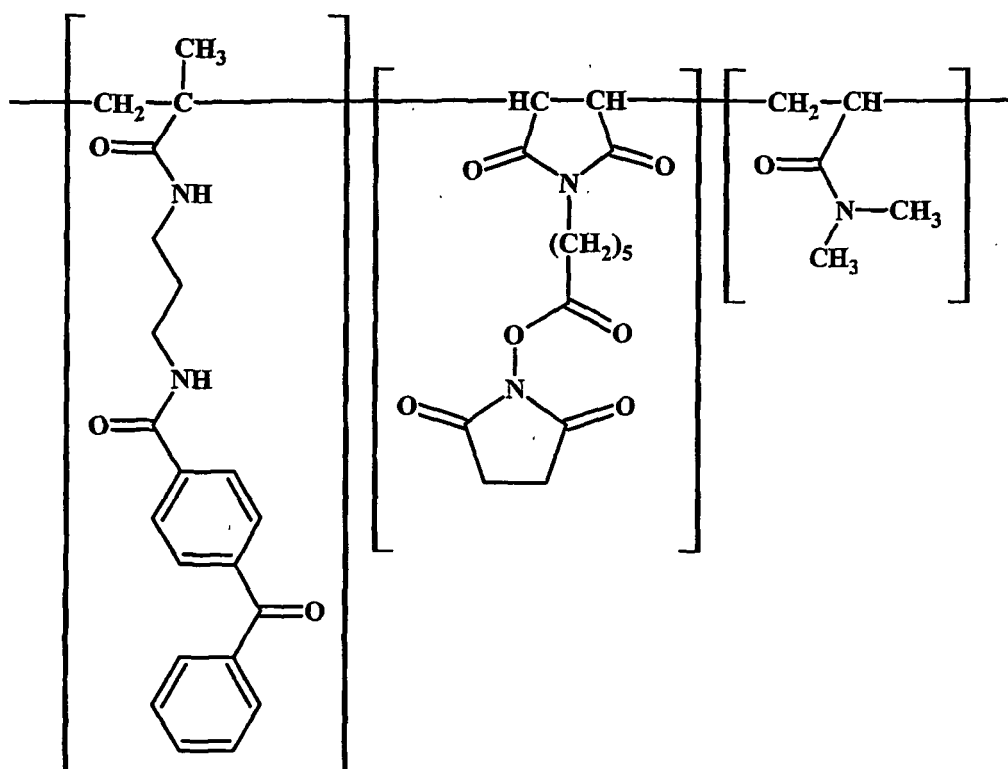
Compound V (Photo-DMA-NOS)
