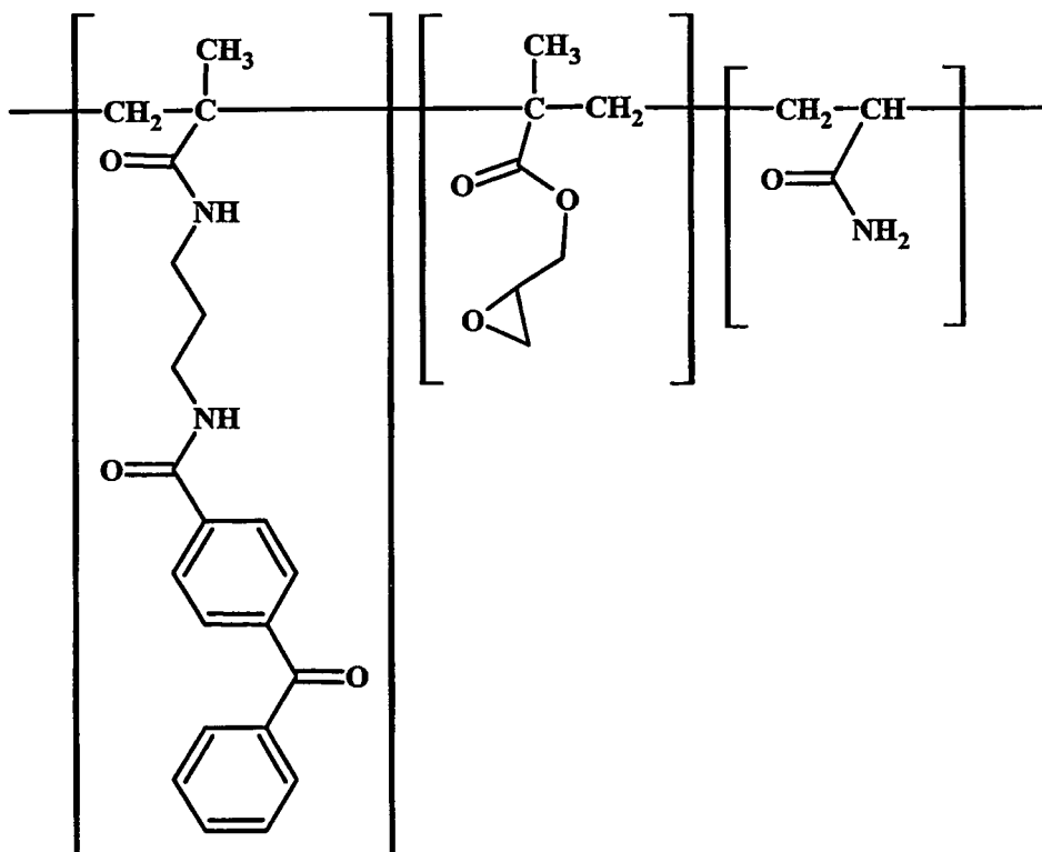
Comparative Compound IX
