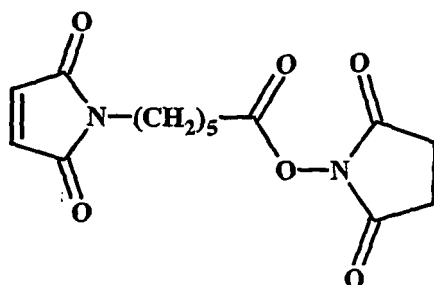
Compound IV (MAL-EAC-NOS)
