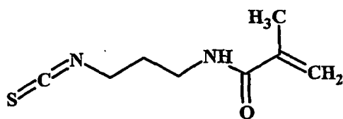
Compound VI (APMA-NCS)
