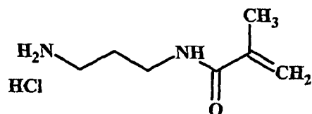
Compound II (APMA-HCL)
