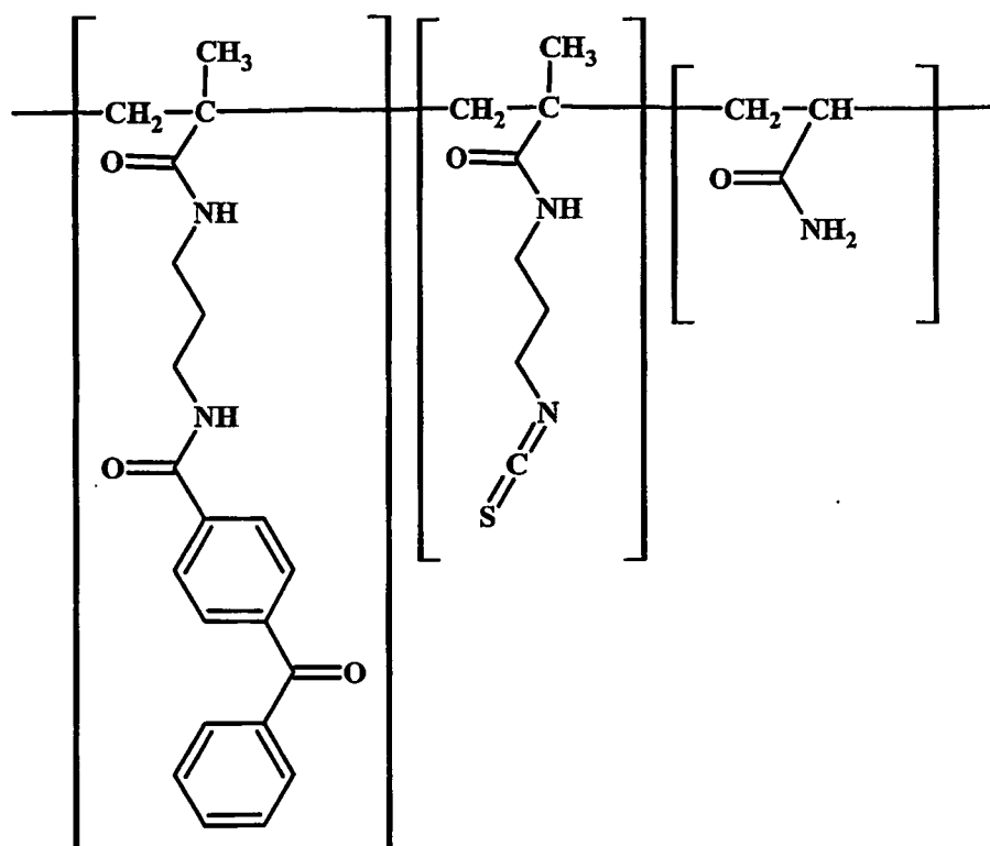
Comparative Compound VIII
