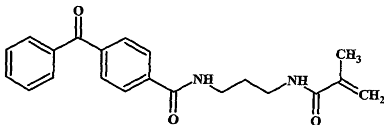
Compound III (BBA-APMA)
