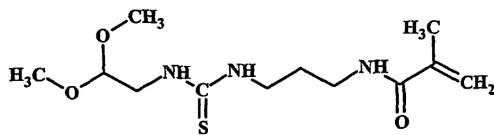
Compound VII (DMA-APMA)
