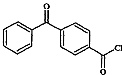
Compound I (BBA)
