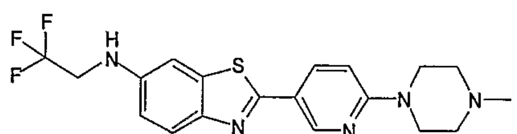
2-[6-(4-Methylpiperazin-1-yl)pyridin-3-yl]-N-(2,2,2-trifluoroethyl)-1,3-benzothiazol-6-amine
