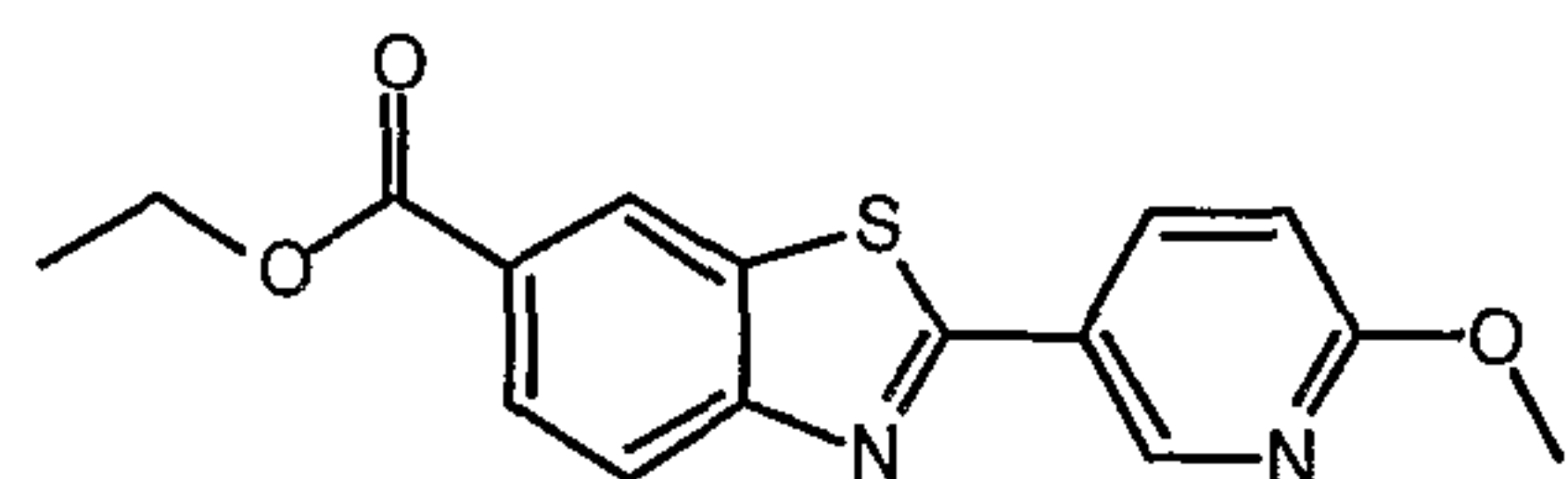
Ethyl 2-(6-methoxypyridin-3-yl)-1,3-benzothiazole-6-carboxylate
