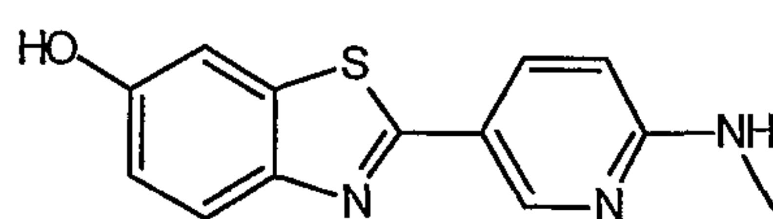
2-[6-(Methylamino)pyridin-3-yl]-1,3-benzothiazol-6-ol
