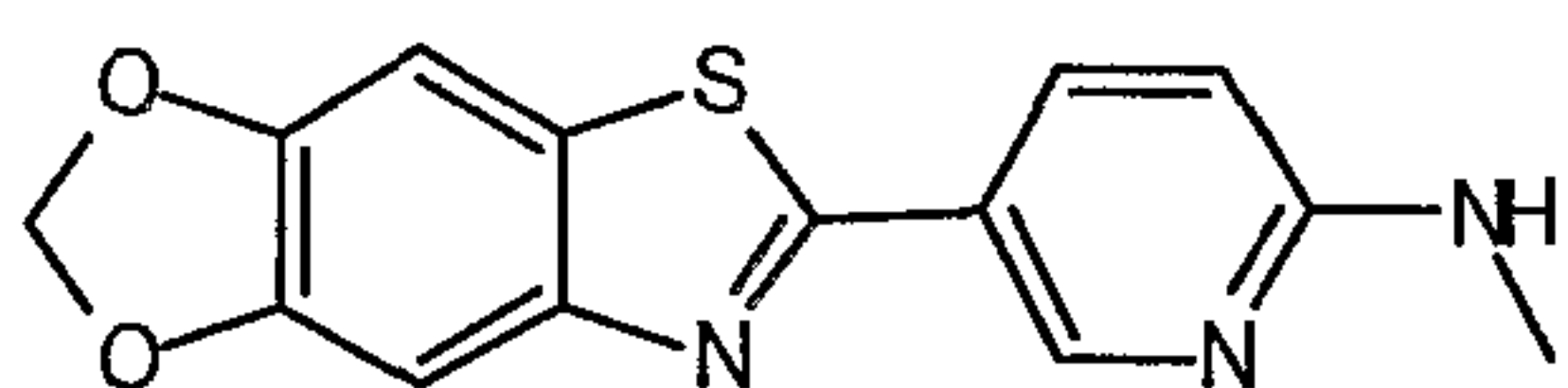
5-[1,3]dioxolo[4,5-f][1,3]benzothiazol-6-yl-N-methylpyridin-2-amine
