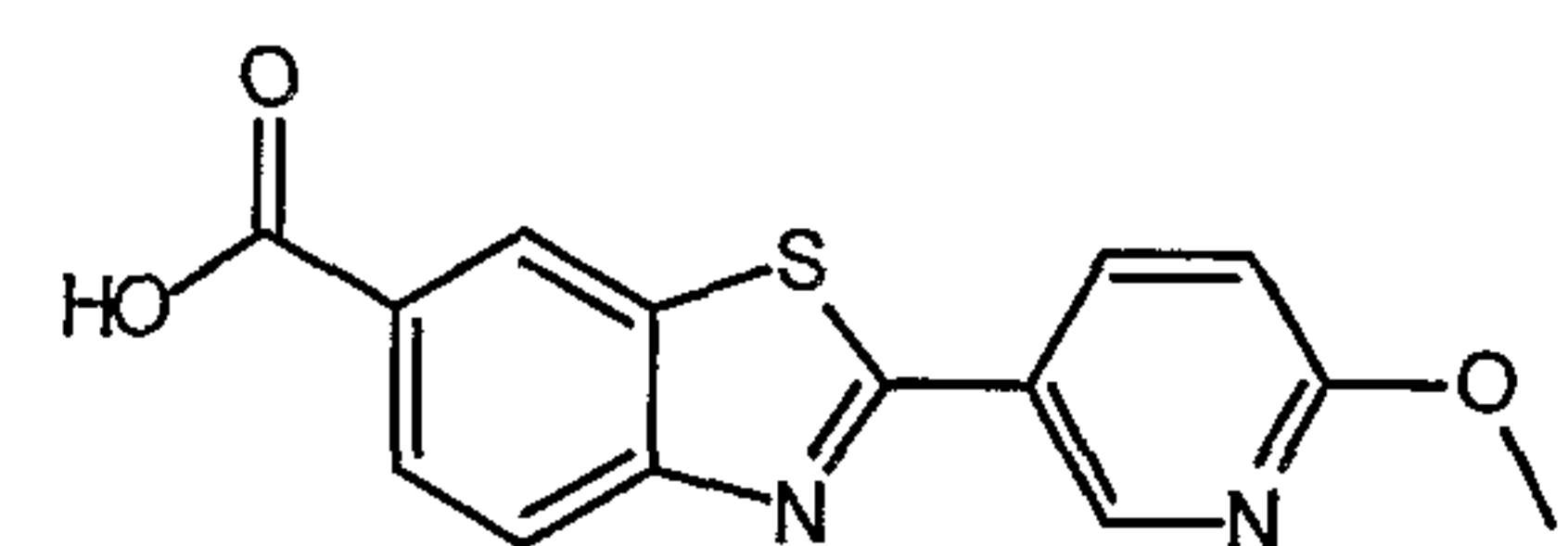
2-(6-methoxypyridin-3-yl)-1,3-benzothiazole-6-carboxylic Acid
