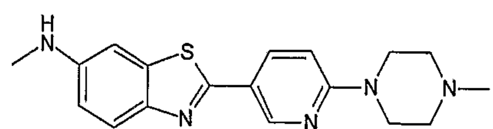
N-Methyl-2-[6-(4-methylpiperazin-1-yl)pyridin-3-yl]-1,3-benzothiazol-6-amine
