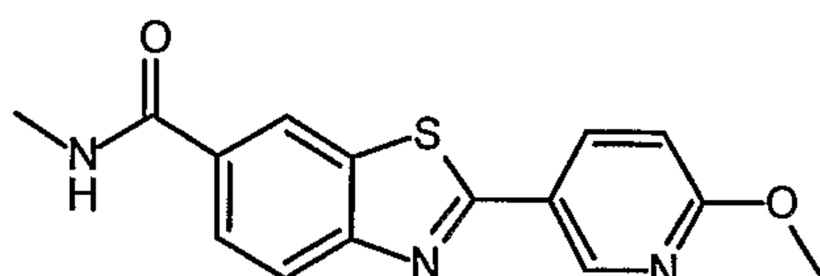
2-(6-Methoxypyridin-3-yl)-N-methyl-1,3-benzothiazole-6-carboxamide
