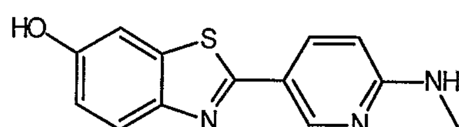
2-[6-(Methylamino)pyridin-3-yl]-1,3-benzothiazol-6-ol
