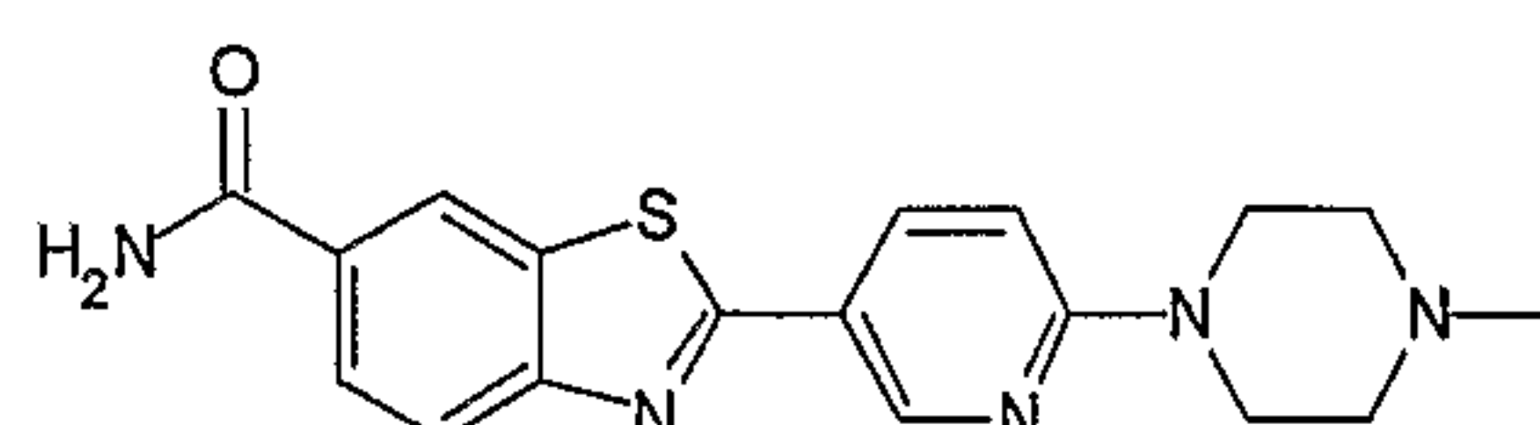
2-[6-(4-Methylpiperazin-1-yl)pyridin-3-yl]-1,3-benzothiazole-6-carboxamide Acetate
