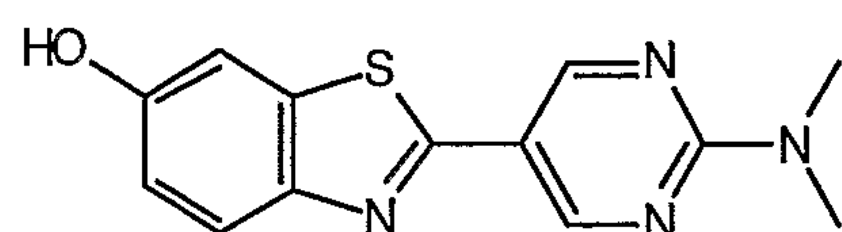
2-[2-(dimethylamino)pyrimidin-5-yl]-1,3-benzothiazol-6-ol
