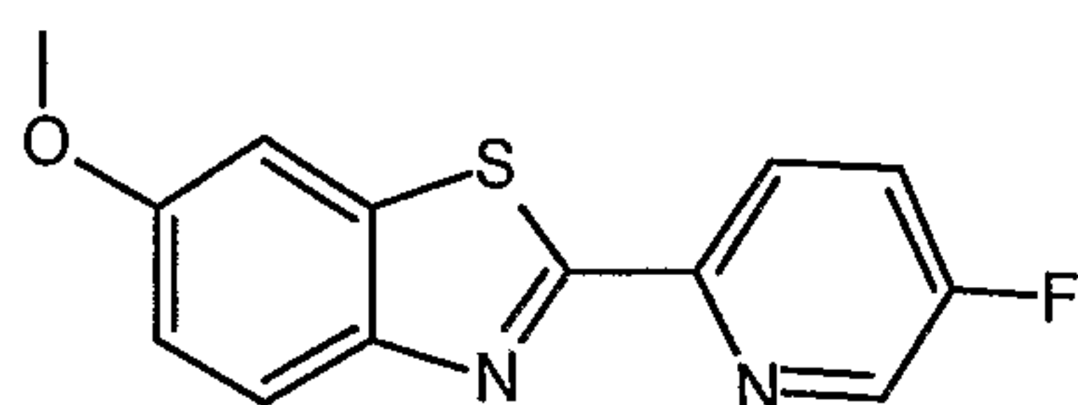
2-(5-fluoropyridin-2-yl)-6-methoxy-1,3-benzothiazole
