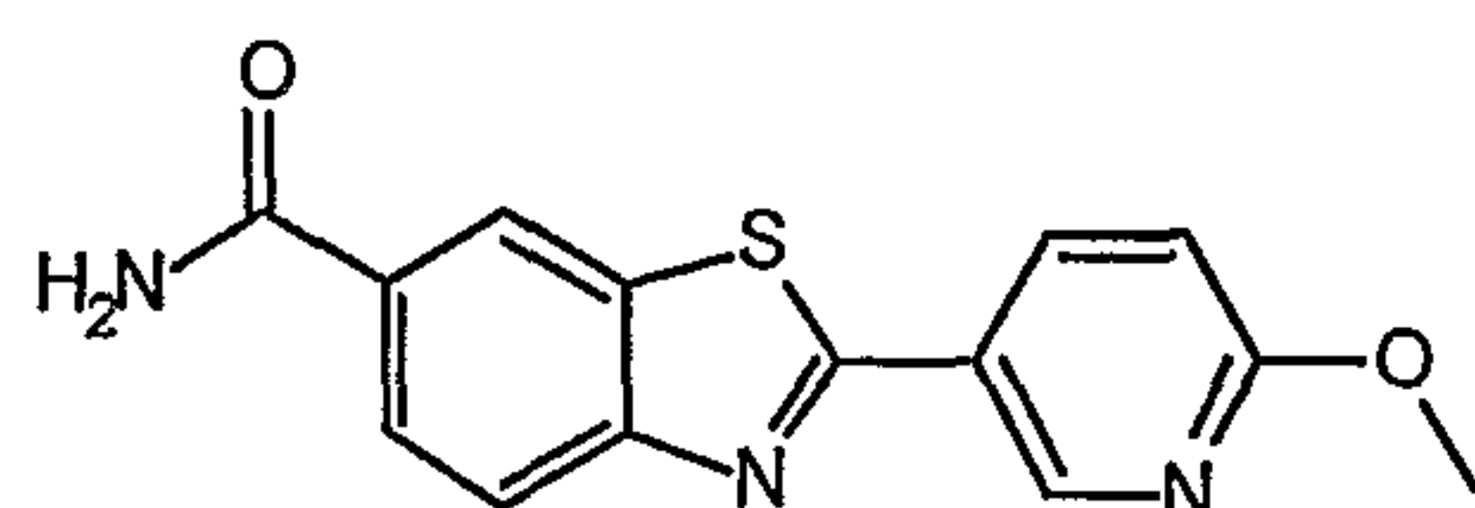
2-(6-Methoxypyridin-3-yl)-1,3-benzothiazole-6-carboxamide
