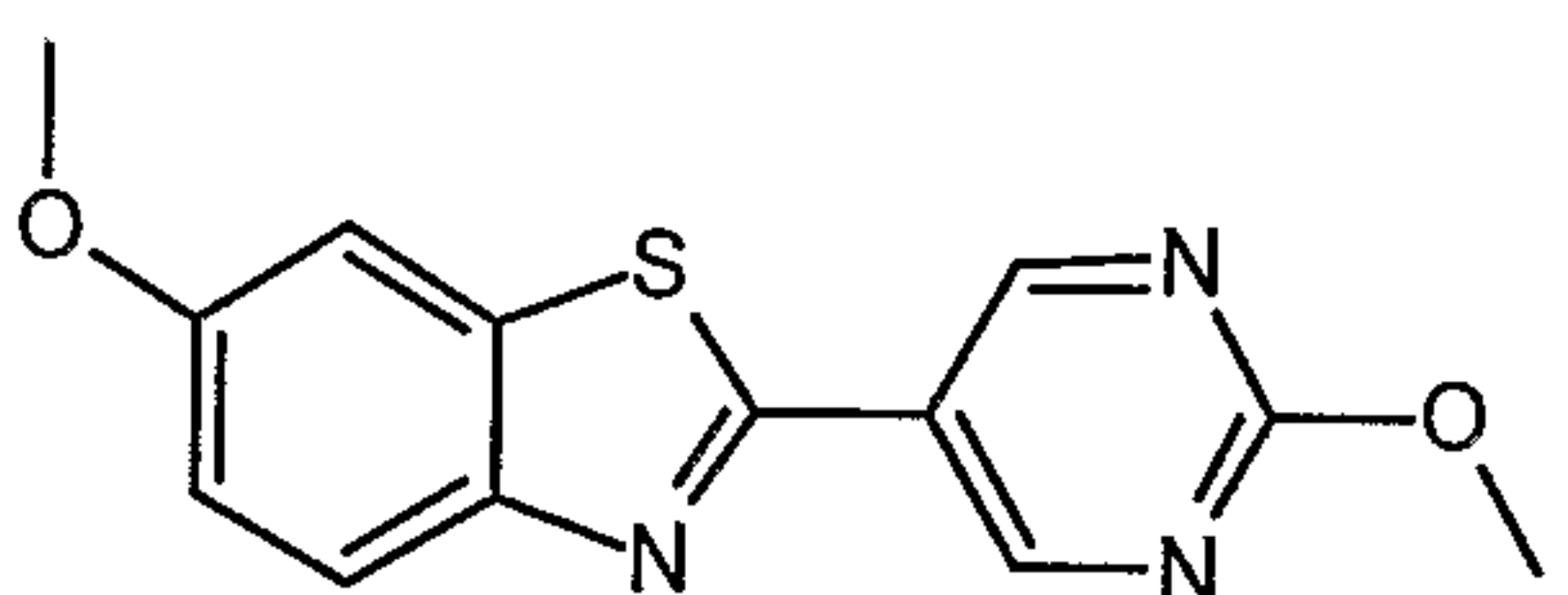
6-methoxy-2-(2-methoxypyrimidin-5-yl)-1,3-benzothiazole
