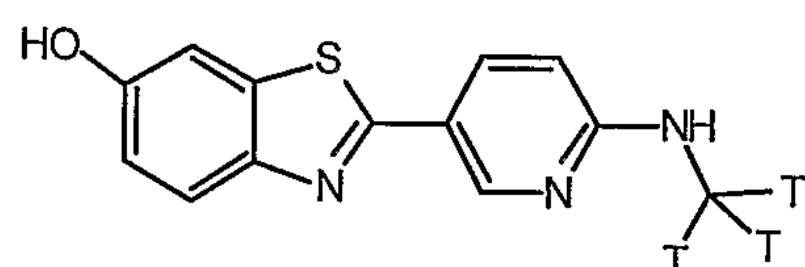
[N-Methyl-3H3]-2-(6-Methylamino-pyridin-3-yl)-benzothiazol-6-ol
