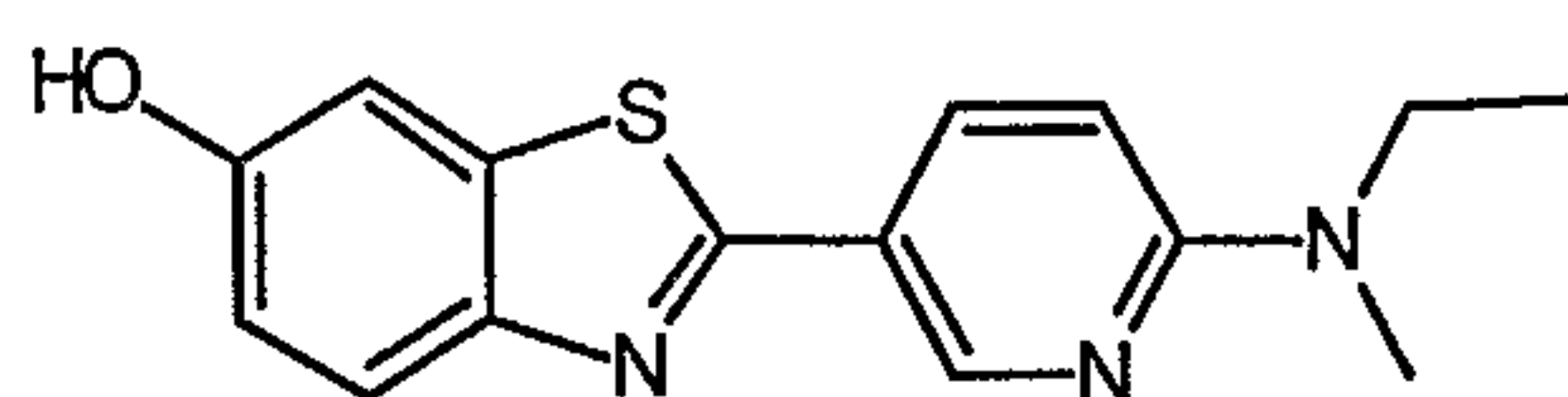
2-{6-[ethyl(methyl)amino]pyridin-3-yl}-1,3-benzothiazol-6-ol
