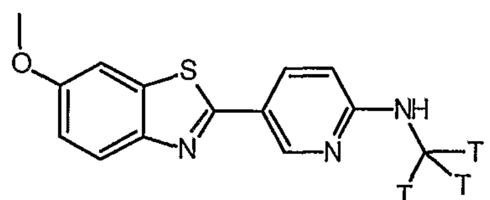
[N-Methyl-3H3]-[5-(6-Methoxy-benzothiazol-2-yl)-pyridin-2-yl]-methyl-amine
