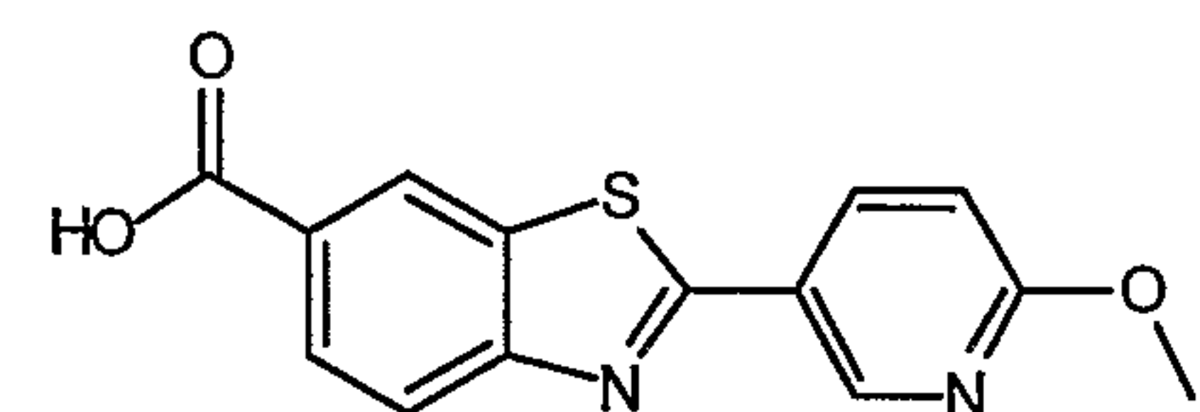
2-(6-Methoxypyridin-3-yl)-1,3-benzothiazole-6-carboxylic Acid
