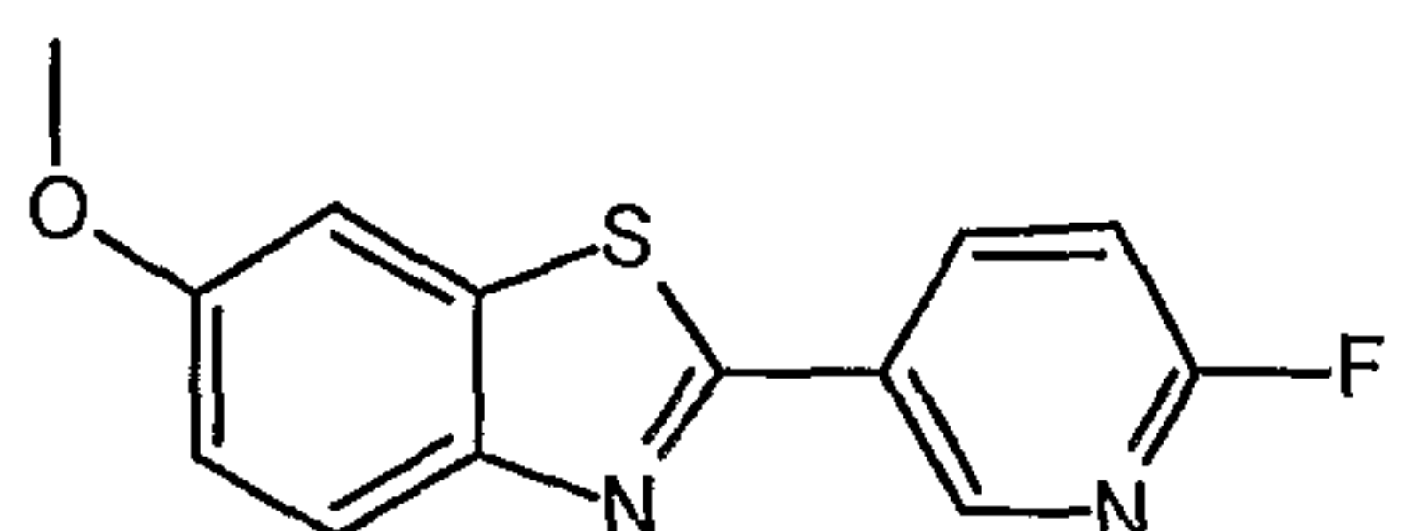
2-(6-Fluoropyridin-3-yl)-6-methoxy-1,3-benzothiazole
