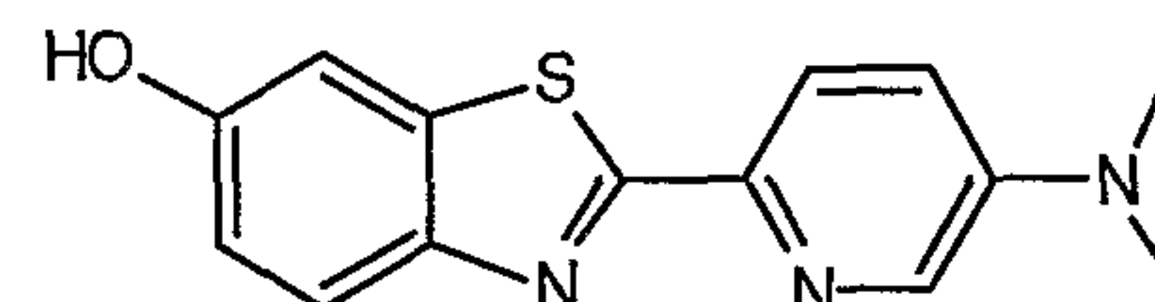
2-[5-(dimethylamino)pyridin-2-yl]-1,3-benzothiazol-6-ol
