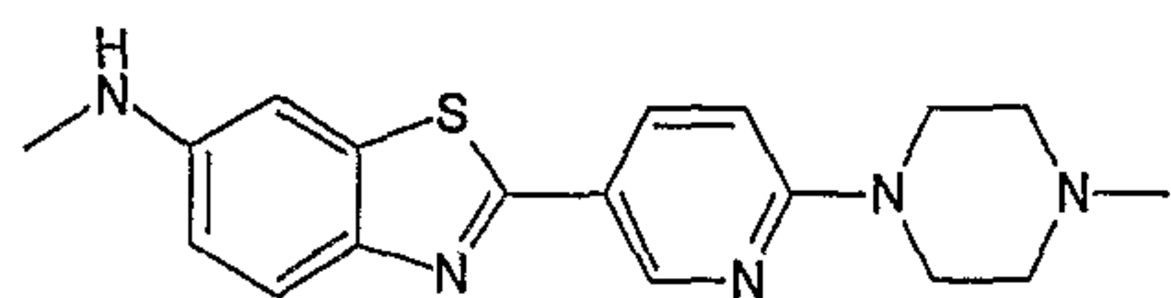
N-Methyl-2-[6-(4-methylpiperazin-1-yl)pyridin-3-yl]-1,3-benzothiazol-6-amine
