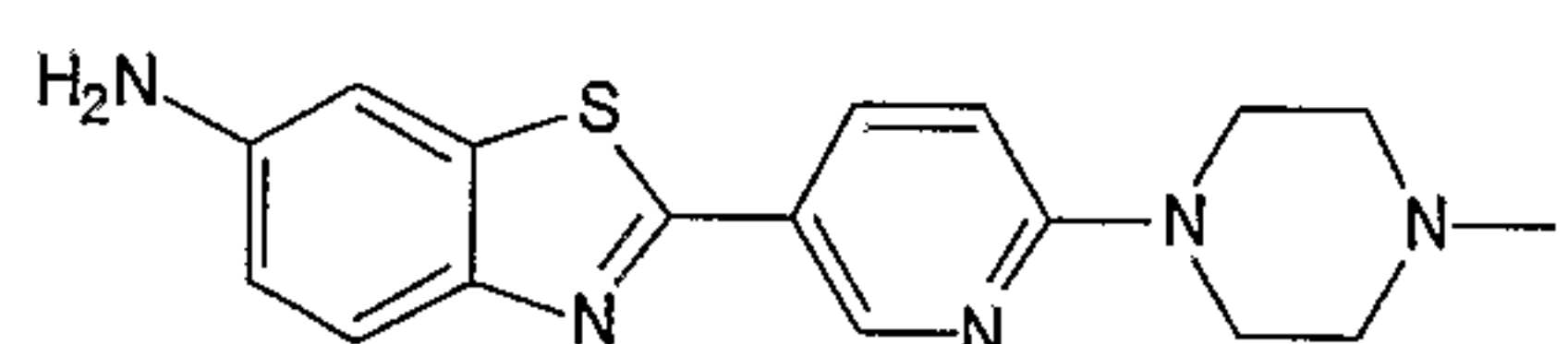
2-[6-(4-Methylpiperazin-1-yl)pyridin-3-yl]-1,3-benzothiazol-6-amine Trifluoroacetate
