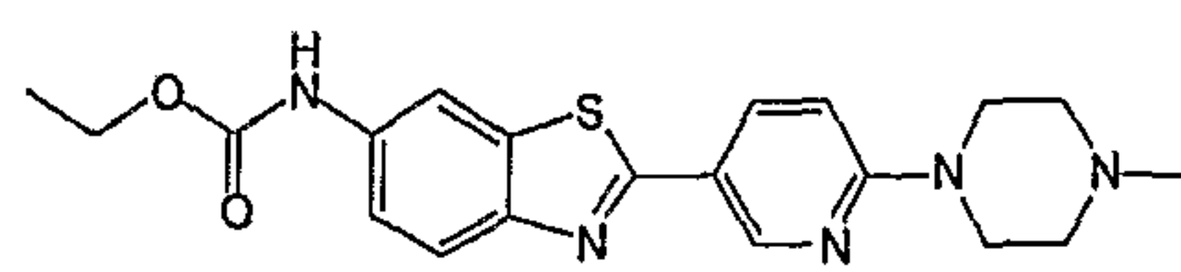
Ethyl {2-[6-(4-Methylpiperazin-1-yl)pyridin-3-yl]-1,3-benzothiazol-6-yl}carbamate
