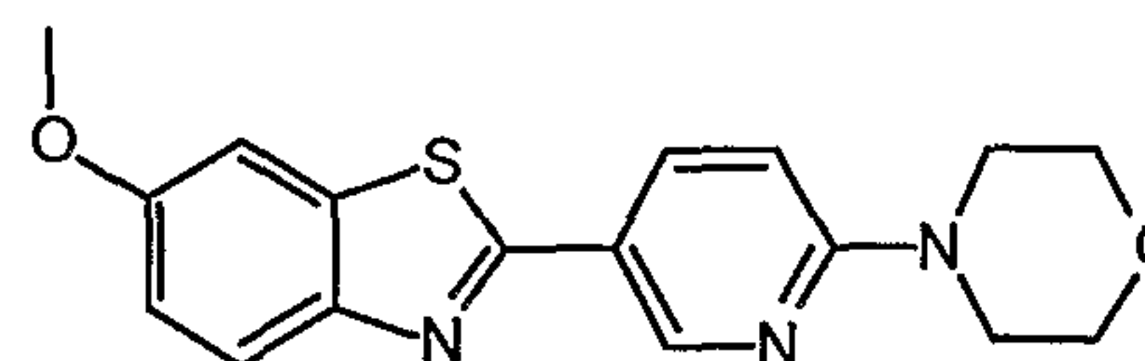
6-methoxy-2-(6-morpholin-4-ylpyridin-3-yl)-1,3-benzothiazole
