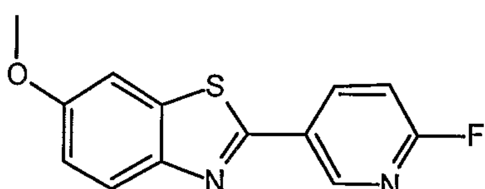
2-(6-Fluoropyridin-3-yl)-6-methoxy-1,3-benzothiazole
