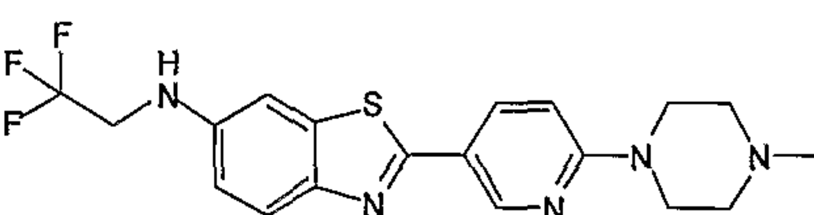
2-[6-(4-Methylpiperazin-1-yl)pyridin-3-yl]-N-(2,2,2-trifluoroethyl)-1,3-benzothiazol-6-amine
