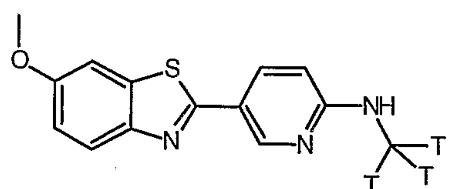
[N-Methyl-3H3]-[5-(6-Methoxy-benzothiazol-2-yl)-pyridin-2-yl]-methyl-amine
