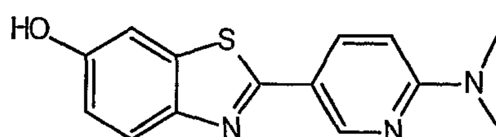
2-[6-(dimethylamino)pyridin-3-yl]-1,3-benzothiazol-6-ol
