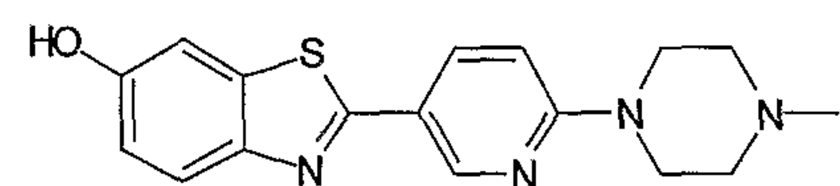
2-[6-(4-methylpiperazin-1-yl)pyridin-3-yl]-1,3-benzothiazol-6-ol Acetate
