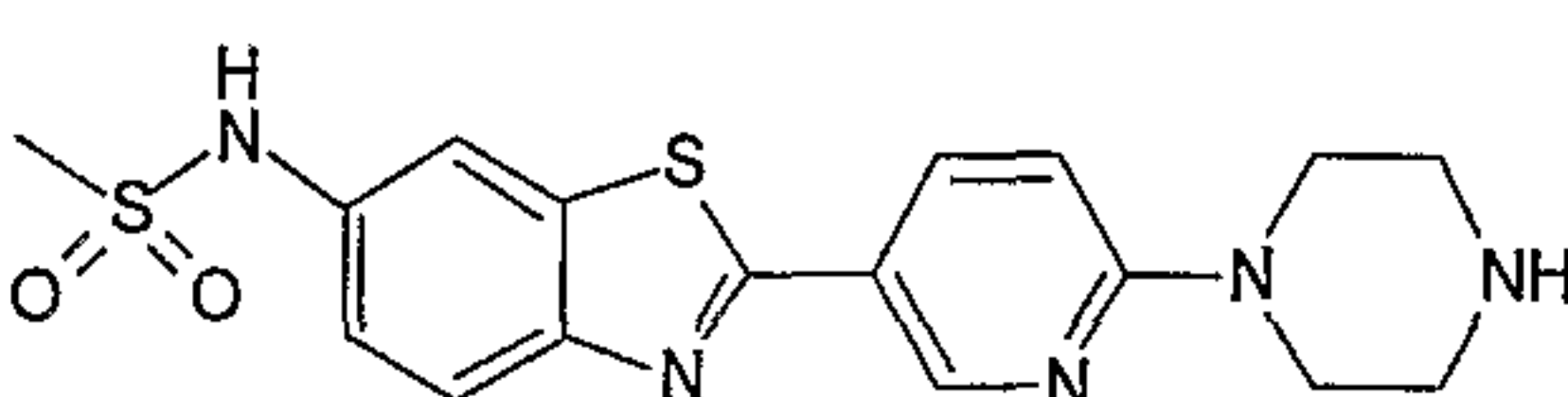
N-[2-(6-Piperazin-1-ylpyridin-3-yl)-1,3-benzothiazol-6-yl]methanesulfonamide
