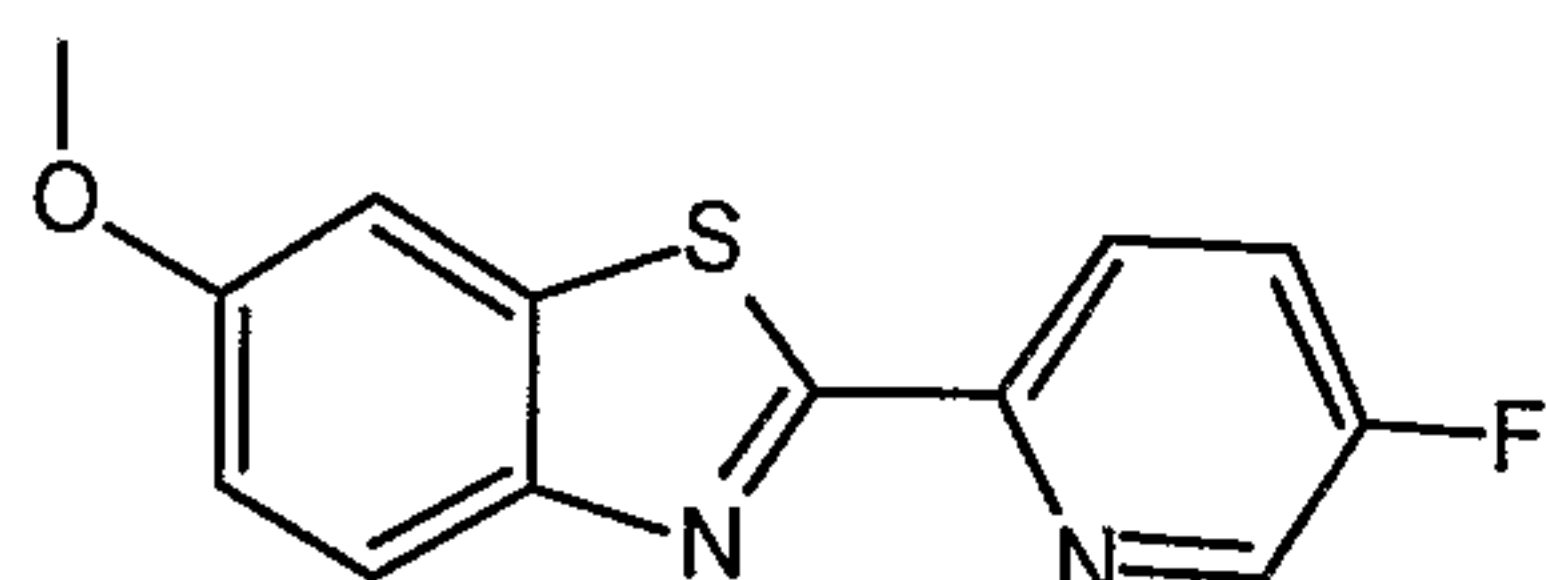
2-(5-fluoropyridin-2-yl)-6-methoxy-1,3-benzothiazole
