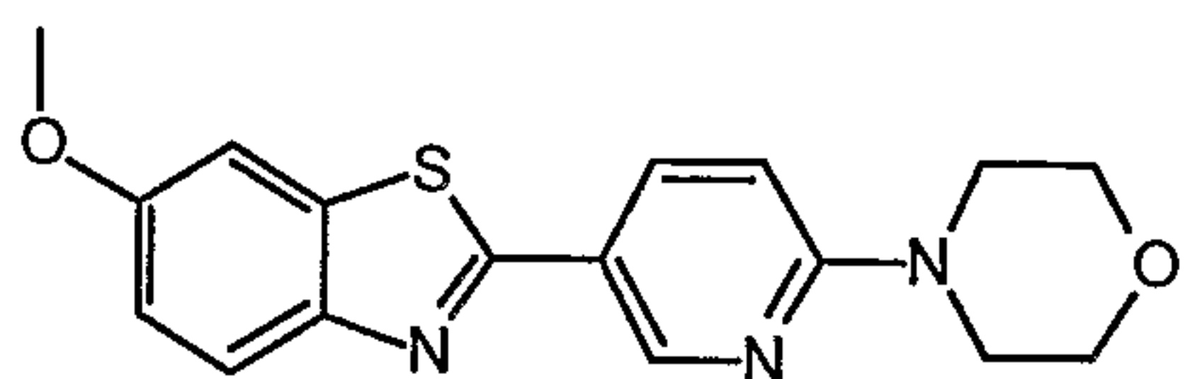
6-methoxy-2-(6-morpholin-4-ylpyridin-3-yl)-1,3-benzothiazole
