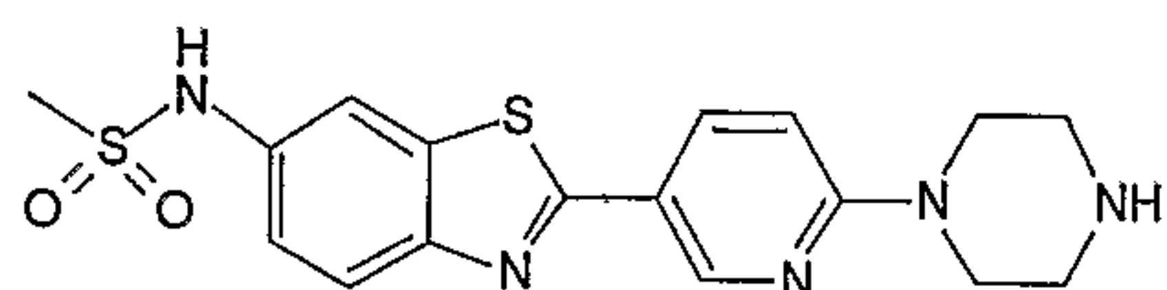
N-[2-(6-Piperazin-1-ylpyridin-3-yl)-1,3-benzothiazol-6-yl]methanesulfonamide
