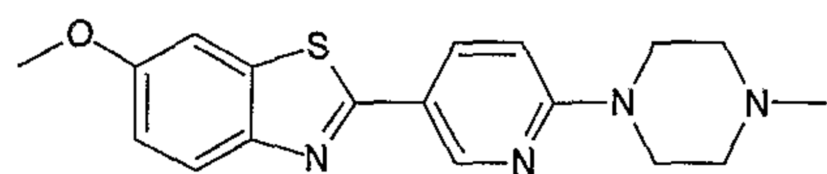
6-methoxy-2-[6-(4-methylpiperazin-1-yl)pyridin-3-yl]-1,3-benzothiazole
