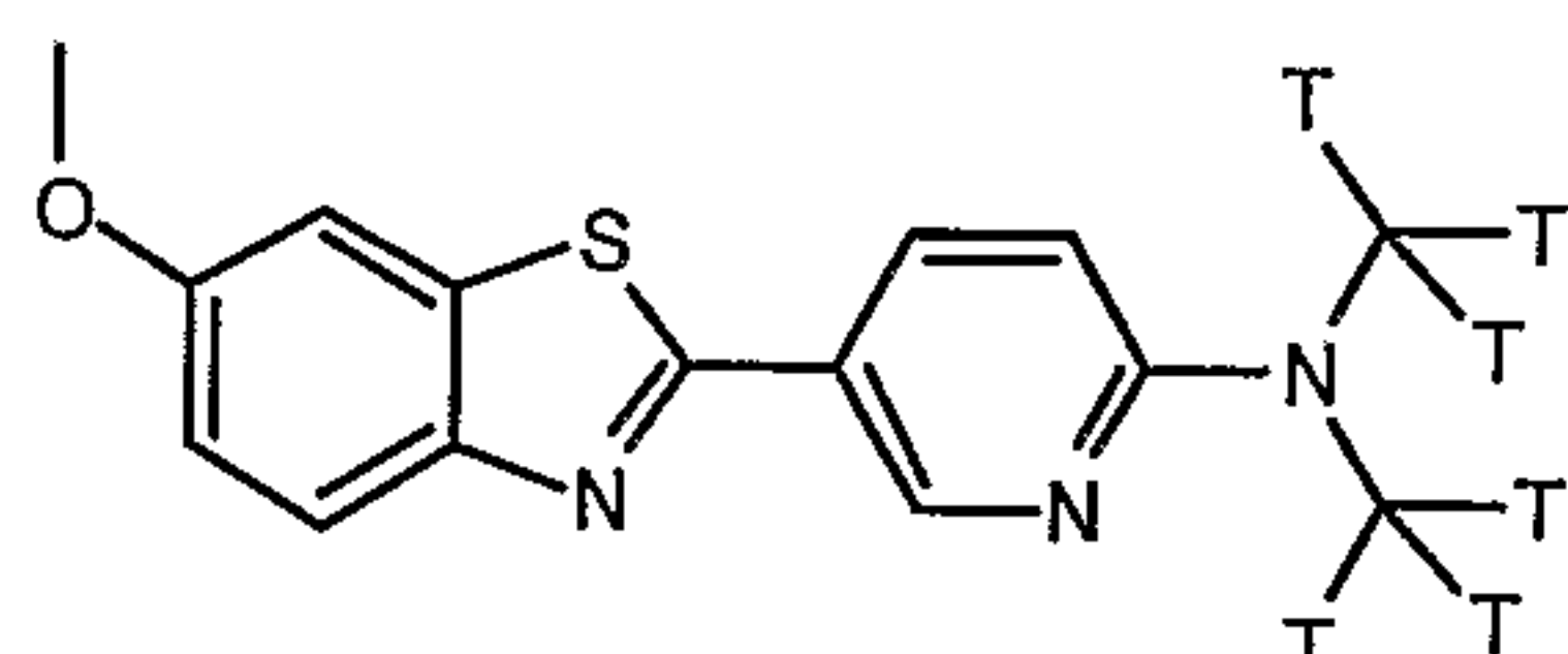
[N-Dimethyl-3H6]-[5-(6-Methoxy-benzothiazol-2-yl)-pyridin-2-yl]-dimethyl-amine
