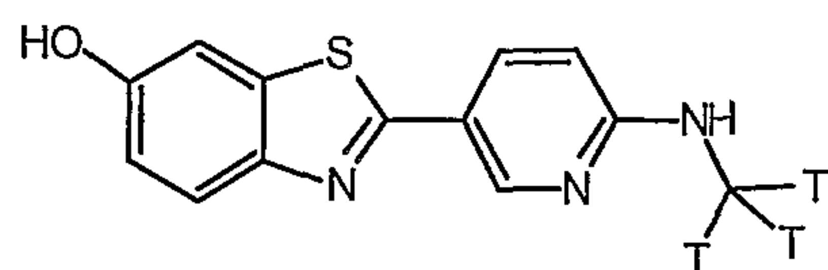
[N-Methyl-3H3]-2-(6-Methylamino-pyridin-3-yl)-benzothiazol-6-ol
