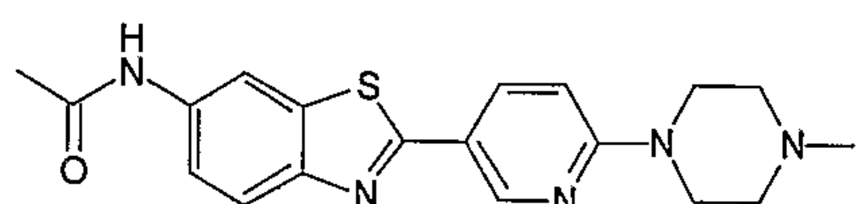
N-{2-[6-(4-Methylpiperazin-1-yl)pyridin-3-yl]-1,3-benzothiazol-6-yl}acetamide
