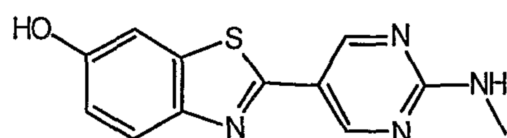
2-[2-(methylamino)pyrimidin-5-yl]-1,3-benzothiazol-6-ol
