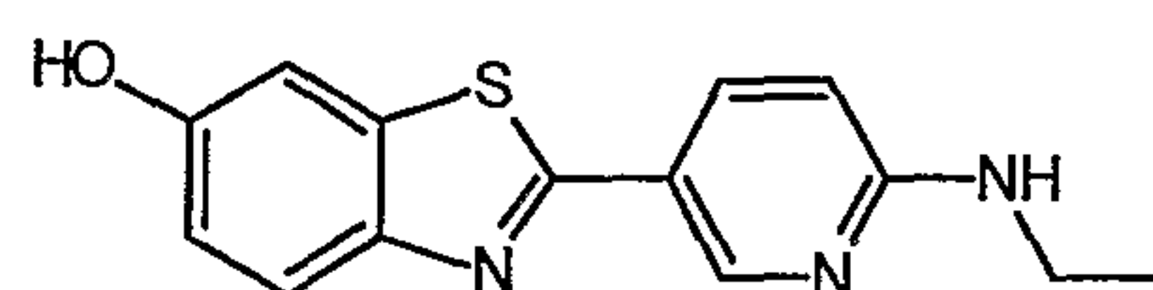
2-[6-(ethylamino)pyridin-3-yl]-1,3-benzothiazol-6-ol
