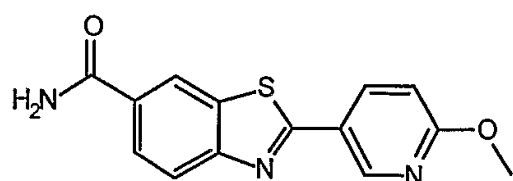
2-(6-Methoxypyridin-3-yl)-1,3-benzothiazole-6-carboxamide
