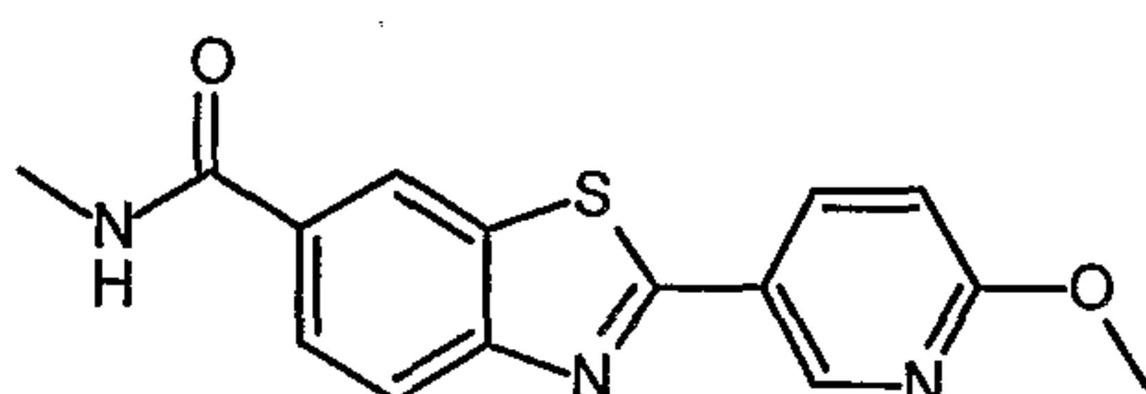
2-(6-Methoxypyridin-3-yl)-N-methyl-1,3-benzothiazole-6-carboxamide
