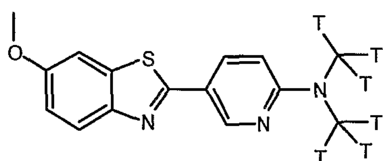
[N-Dimethyl-3H6]-[5-(6-Methoxy-benzothiazol-2-yl)-pyridin-2-yl]-dimethyl-amine
