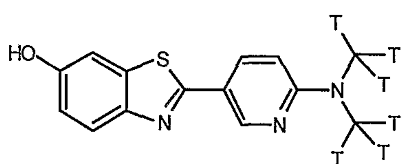
[N-Dimethyl-3H6]-2-(6-Dimethylamino-pyridin-3-yl)-benzothiazol-6-ol
