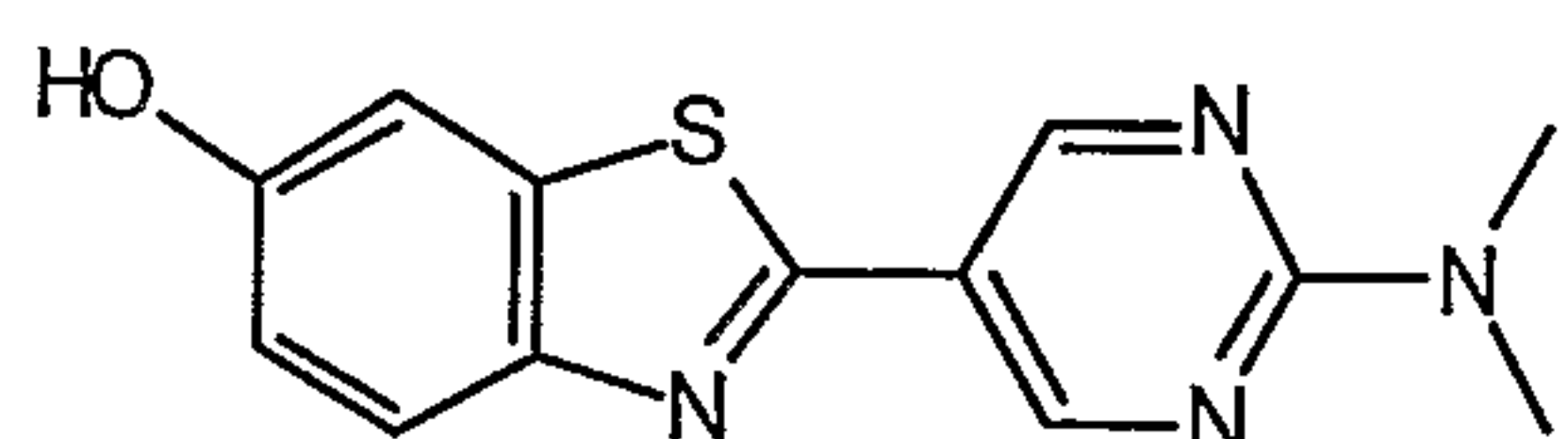
2-[2-(dimethylamino)pyrimidin-5-yl]-1,3-benzothiazol-6-ol
