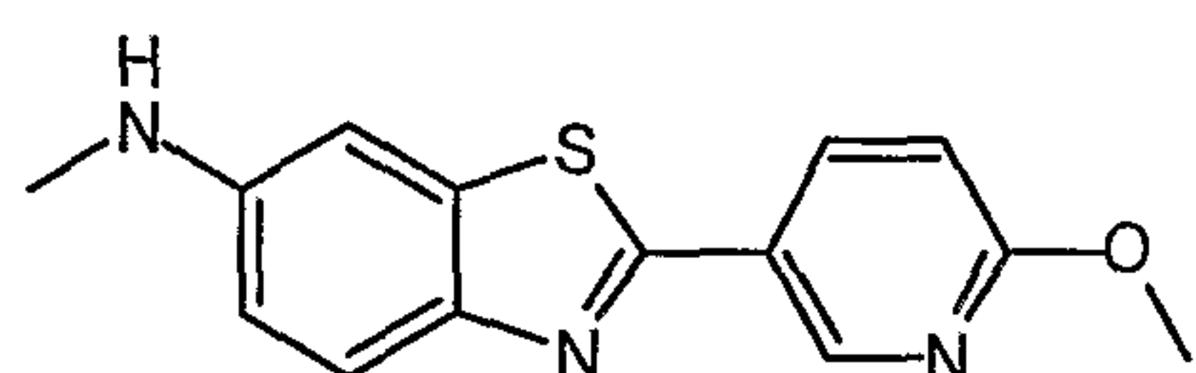
2-(6-Methoxypyridin-3-yl)-N-methyl-1,3-benzothiazol-6-amine
