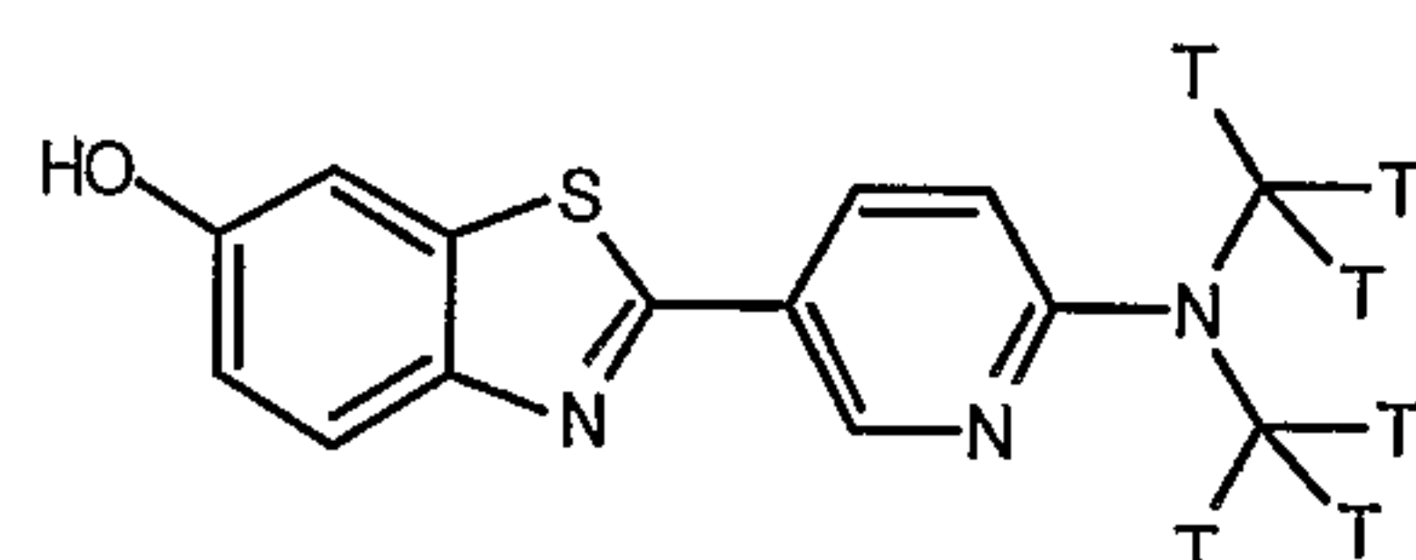
[N-Dimethyl-3H6]-2-(6-Dimethylamino-pyridin-3-yl)-benzothiazol-6-ol
