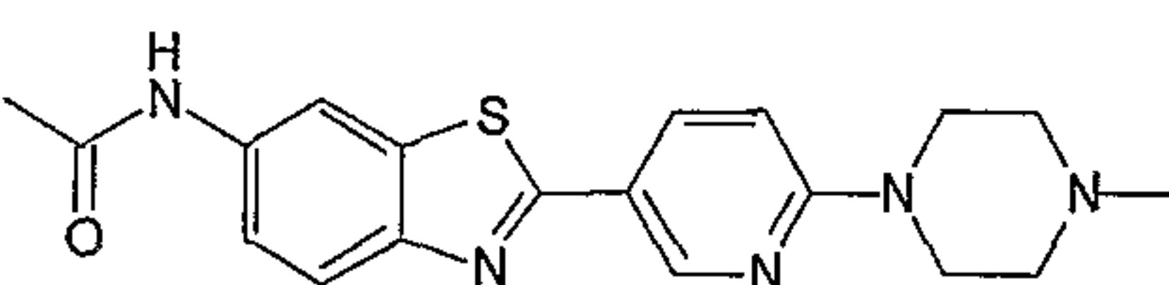
N-[2-[6-(4-Methylpiperazin-1-yl)pyridin-3-yl]-1,3-benzothiazol-6-yl]acetamide
