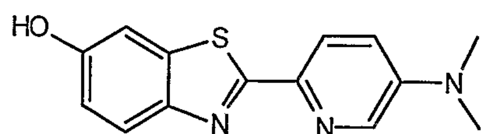
2-[5-(dimethylamino)pyridin-2-yl]-1,3-benzothiazol-6-ol
