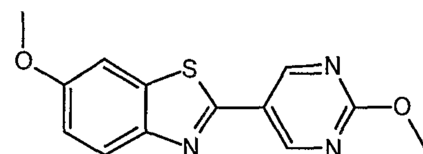
6-methoxy-2-(2-methoxypyrimidin-5-yl)-1,3-benzothiazole
