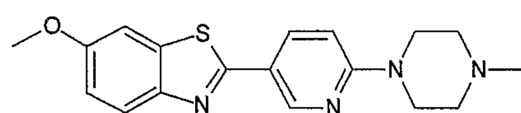
6-Methoxy-2-[6-(4-methylpiperazin-1-yl)pyridin-3-yl]-1,3-benzothiazole
