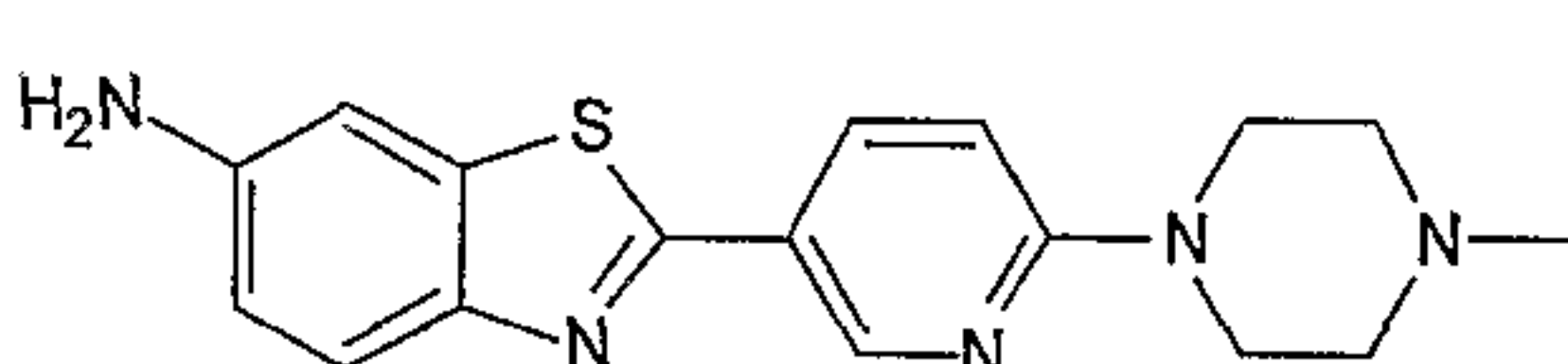
2-[6-(4-Methylpiperazin-1-yl)pyridin-3-yl]-1,3-benzothiazol-6-amine Trifluoroacetate
