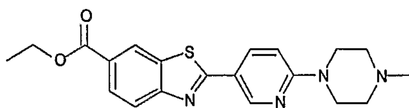
Ethyl 2-[6-(4-Methylpiperazin-1-yl)pyridin-3-yl]-1,3-benzothiazole-6-carboxylate
