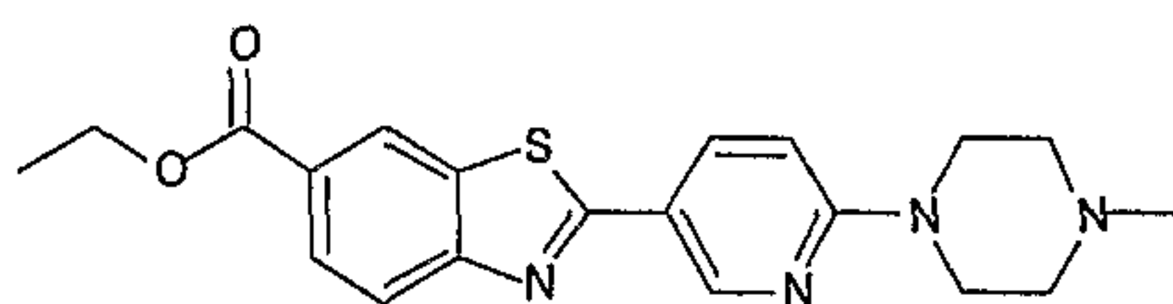
Ethyl 2-[6-(4-methylpiperazin-1-yl)pyridin-3-yl]-1,3-benzothiazole-6-carboxylate
