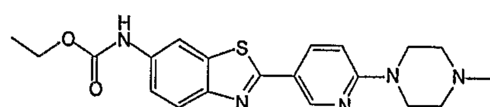
Ethyl {2-[6-(4-Methylpiperazin-1-yl)pyridin-3-yl]-1,3-benzothiazol-6-yl}carbamate
