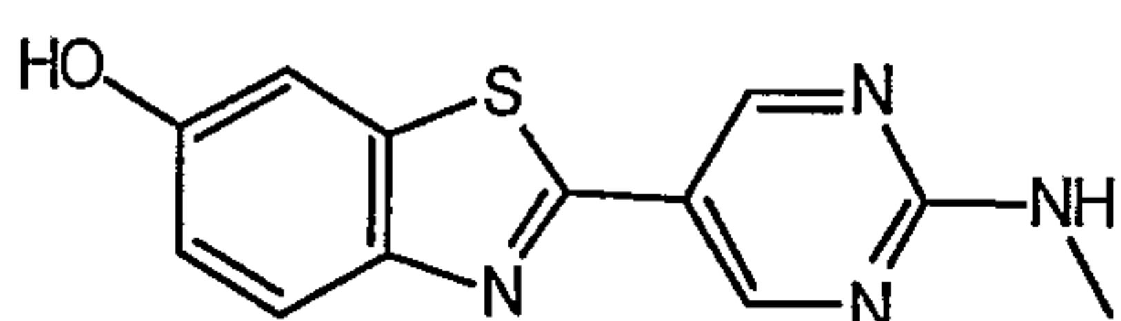
2-[2-(methylamino)pyrimidin-5-yl]-1,3-benzothiazol-6-ol
