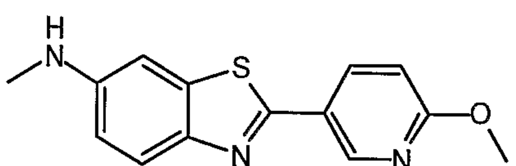
2-(6-Methoxypyridin-3-yl)-N-methyl-1,3-benzothiazol-6-amine
