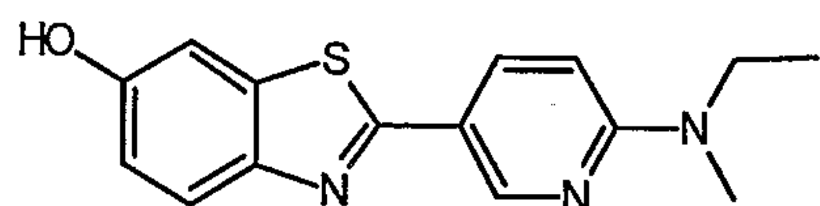
2-{6-[ethyl(methyl)amino]pyridin-3-yl}-1,3-benzothiazol-6-ol
