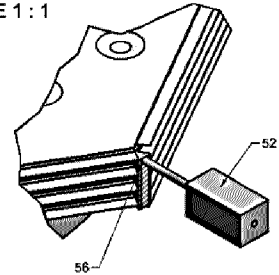
FIG. 7C HOT MELT DETAIL D SCALE 1 : 1
