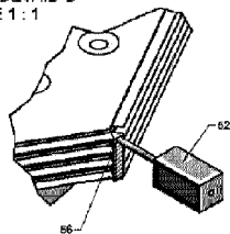
C HOT MELT DETAIL D SCALE 1 : 1
