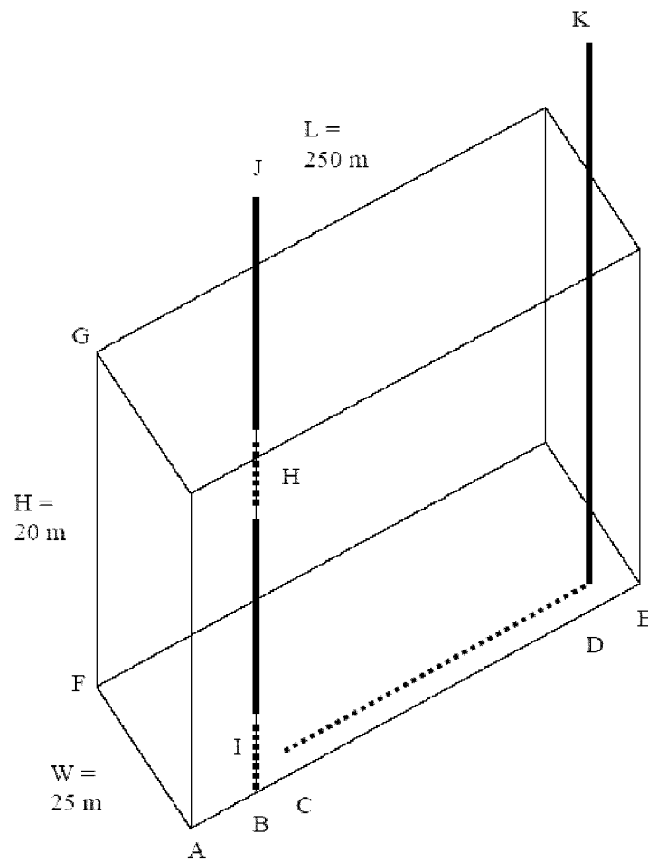
Figure 2. Reservoir Dimensions and Placement of Wells
