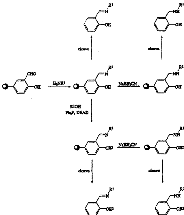
Scheme 28
