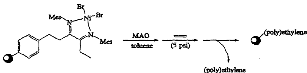
Scheme 20
