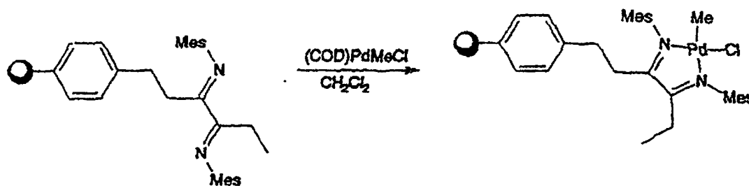
Scheme 18
