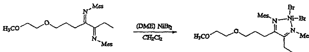
Scheme 8
