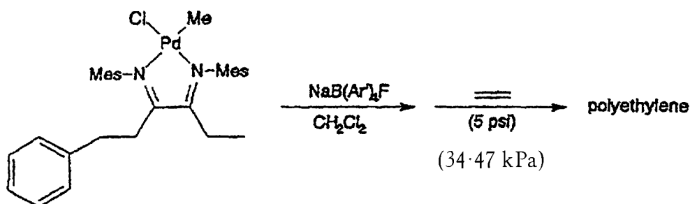
Scheme 26
