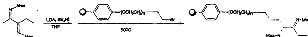
Scheme 14
