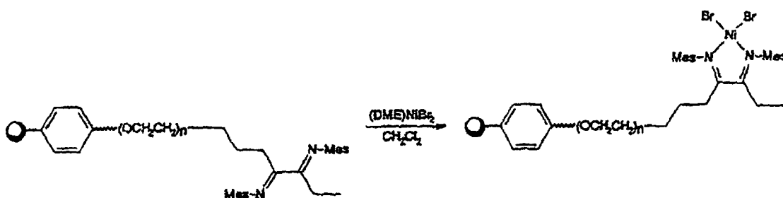
Scheme 16
