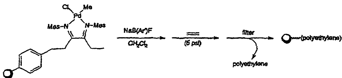
Scheme 25
