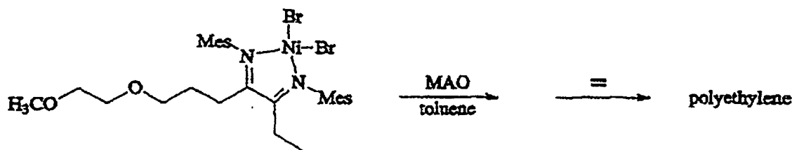
Scheme 21
