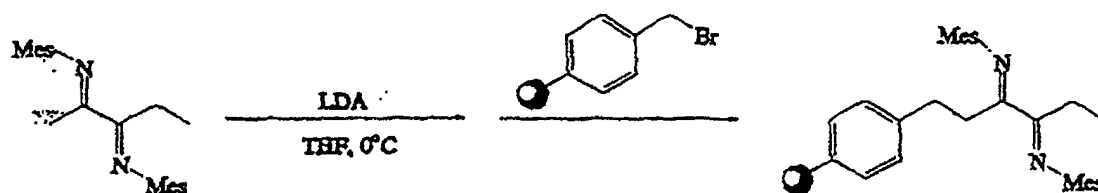
Scheme 12
