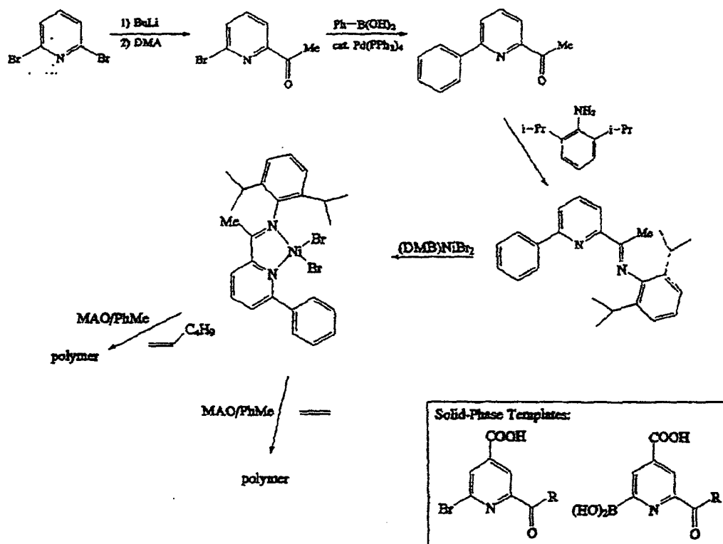
Scheme 27
