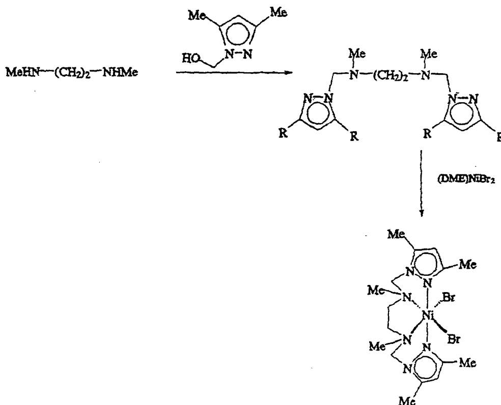
Scheme 29
