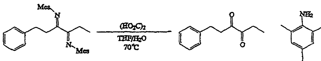
Scheme 6
