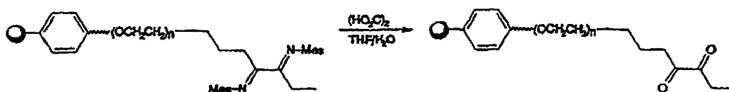
Scheme 15
