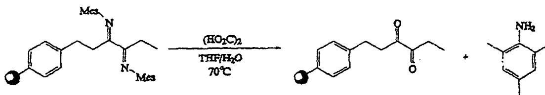
Scheme 13
