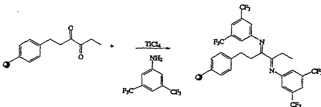
Scheme 19
