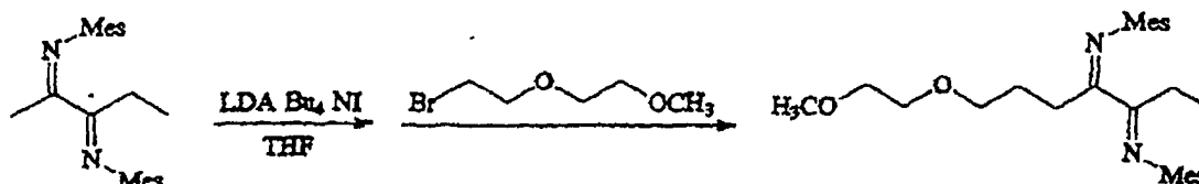
Scheme 7
