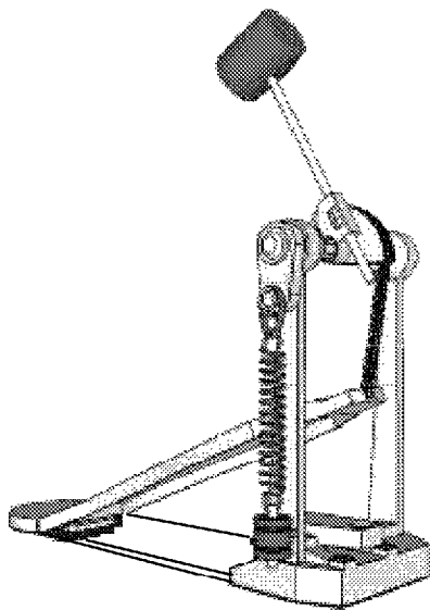
FIG. 2 (prior art)
