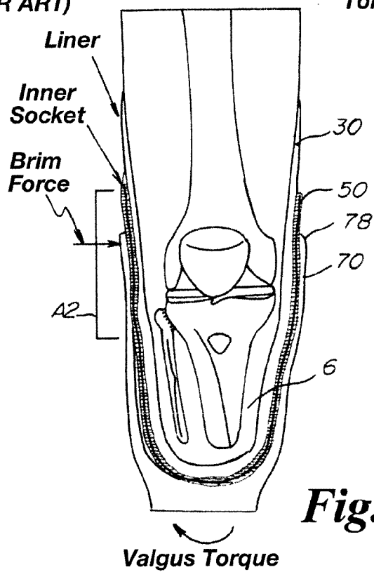
Fig. 5 (PRIOR ART)
