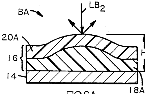
FIG. 6A READ MODE
