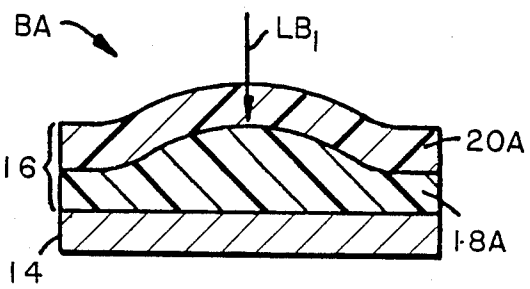
FIG. 7B ERASE/WRITE CYCLE WRITE
