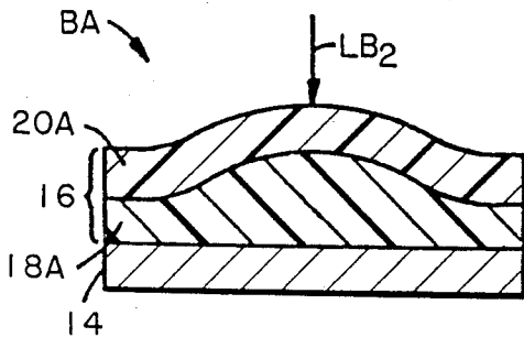
FIG. 7A ERASE/WRITE CYCLE ERASE
