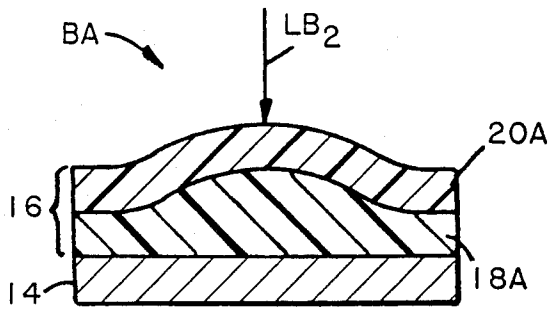
FIG. 5A ERASE MODE
