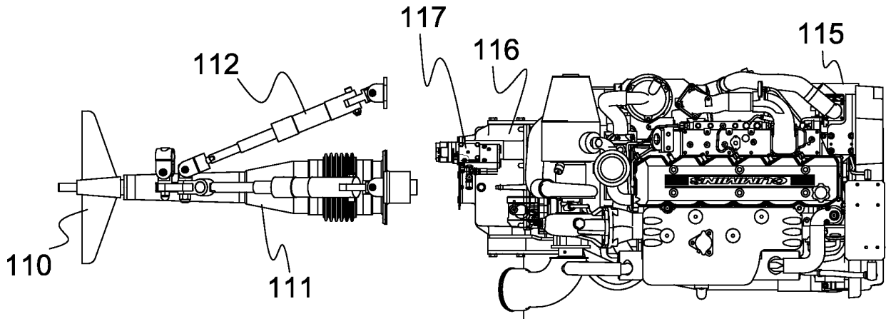
FIG. 1E SURFACE DRIVE TOP VIEW
