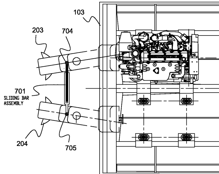
FIGURE 7B SLIDING BAR DRIVES POSITIONED INWARD
