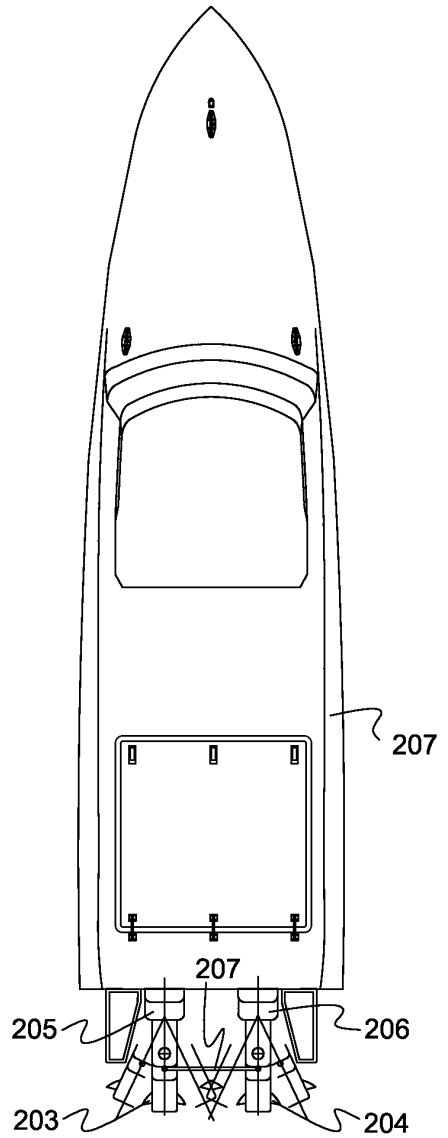
FIG. 2D DUAL STERNDRIVE / OUTDRIVE
