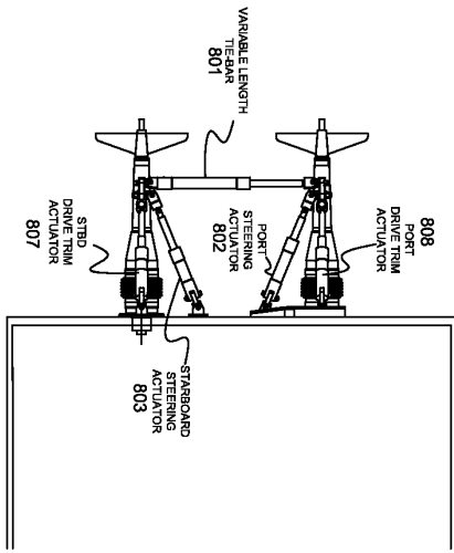
FIGURE 8B VARIABLE LENGTH TIE-BAR (LOCKING OR ACTIVE) DRIVES PARALLEL
