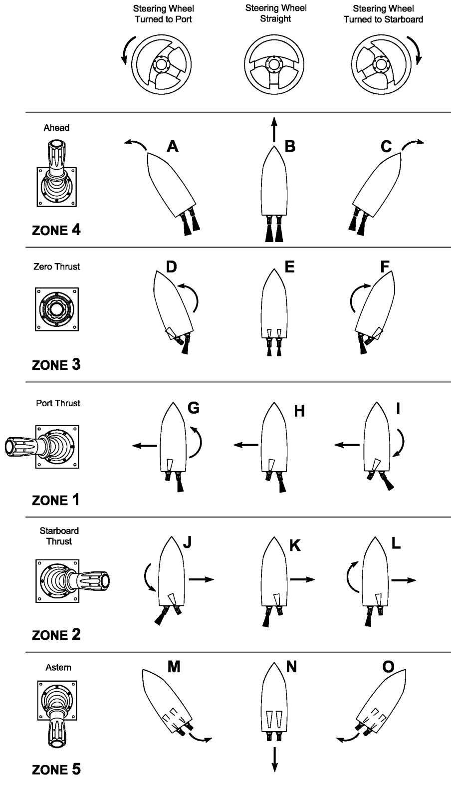
FIGURE 4A DUAL INTEGRATED BUCKET WATERJET NET THRUST VECTORS
