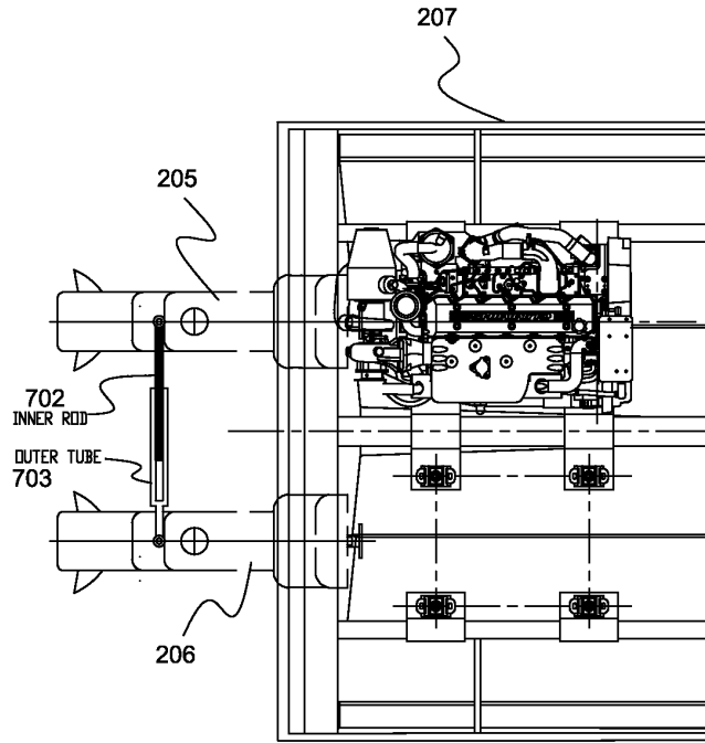
FIGURE 7A SLIDING BAR DRIVES PARALLEL
