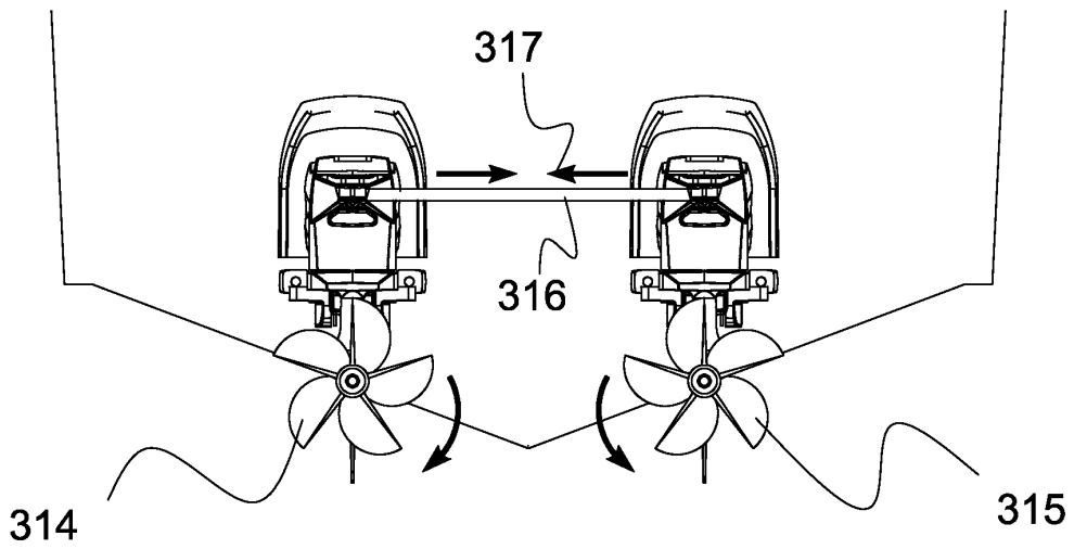
FIG. 3B PROPELLERS TURNING INBOARD
