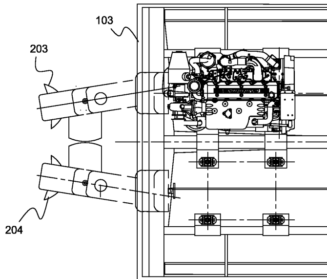
FIGURE 6B BUMPERS DRIVES POSITIONED INWARD
