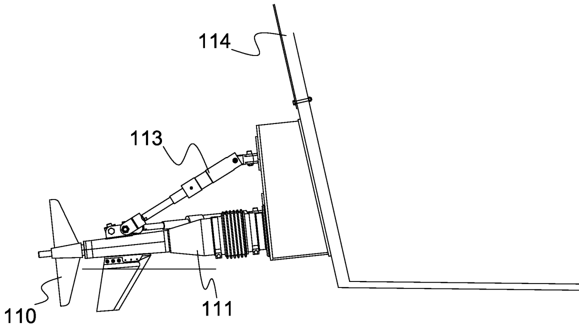
FIG. 1D SURFACE DRIVE SIDE VIEW
