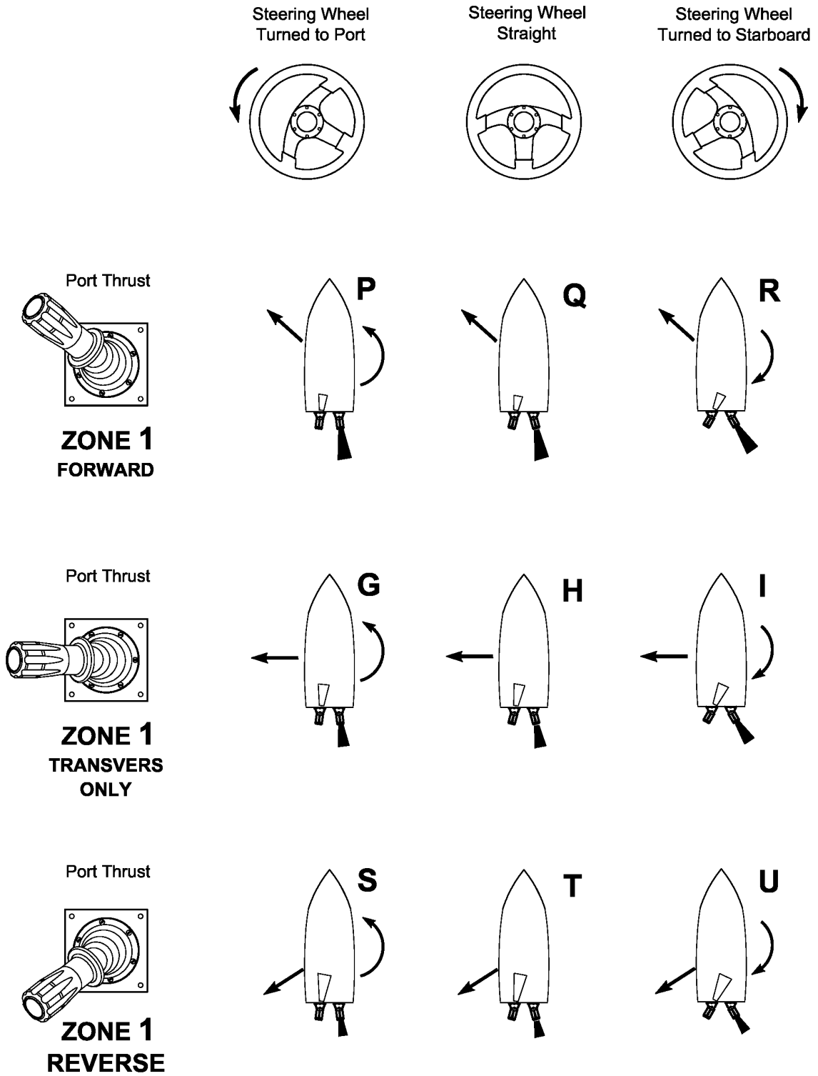
FIGURE 4B DUAL INTEGRATED BUCKET WATERJET NET THRUST VECTORS TRANSVERSE AND DIAGNAL EXAMPLES OF ZONE 1
