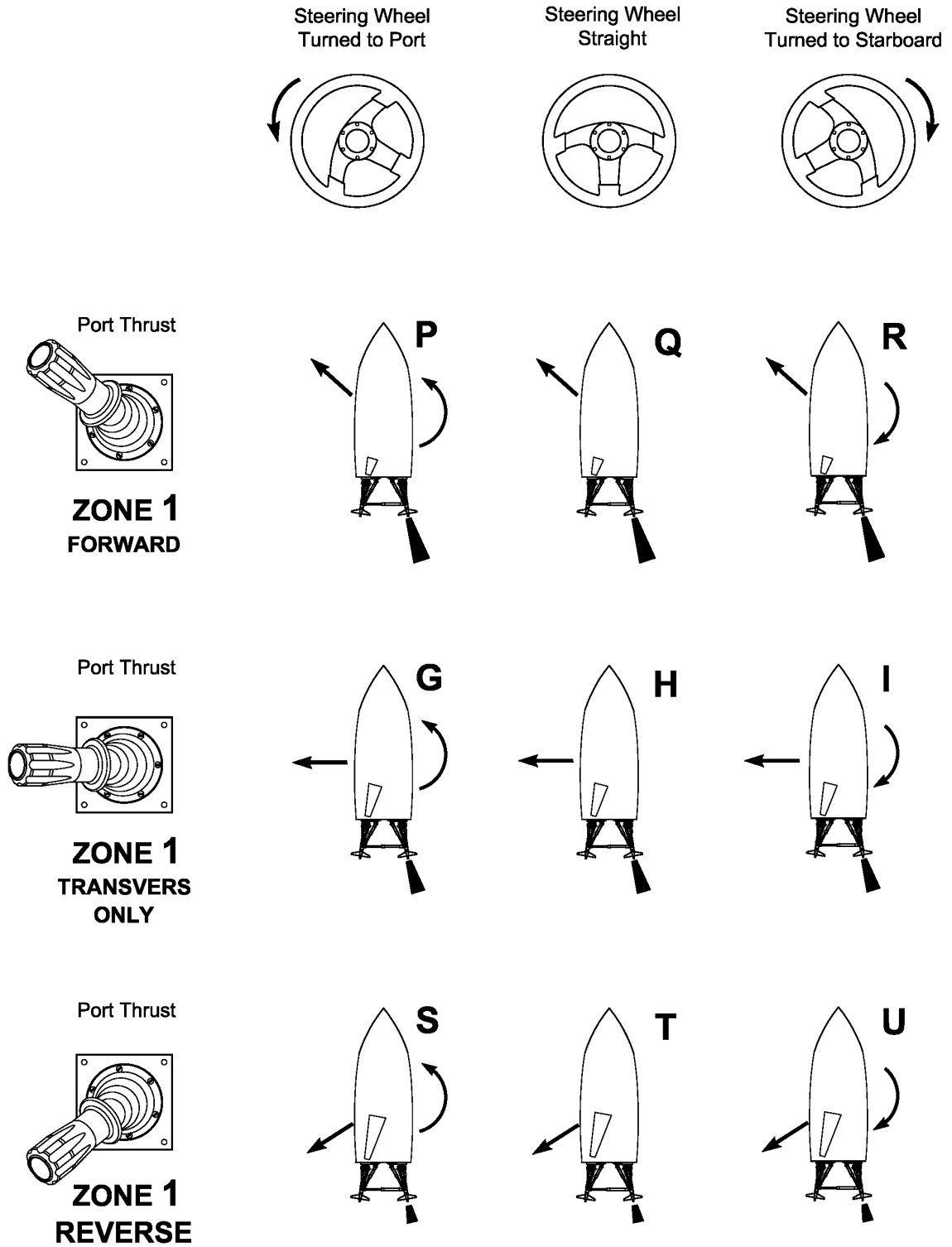
FIGURE 5B DUAL STEERABLE PROPELLER NET THRUST VECTORS TRANSVERSE AND DIAGNAL EXAMPLES OF ZONE 1
