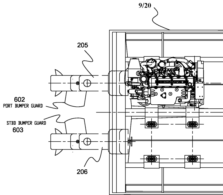
FIGURE 6A BUMPERS DRIVES PARALLEL
