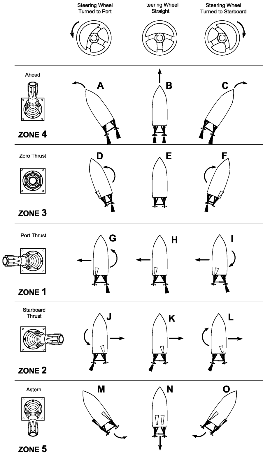
FIGURE 5A DUAL STEERABLE PROPELLER NET THRUST VECTORS
