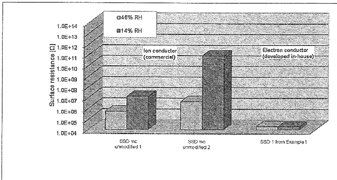
Surface resistance of various self-shining dispersions for floorcoverings having particular requirements of the electrical behaviour for two different atmospheric humidities (RH)
